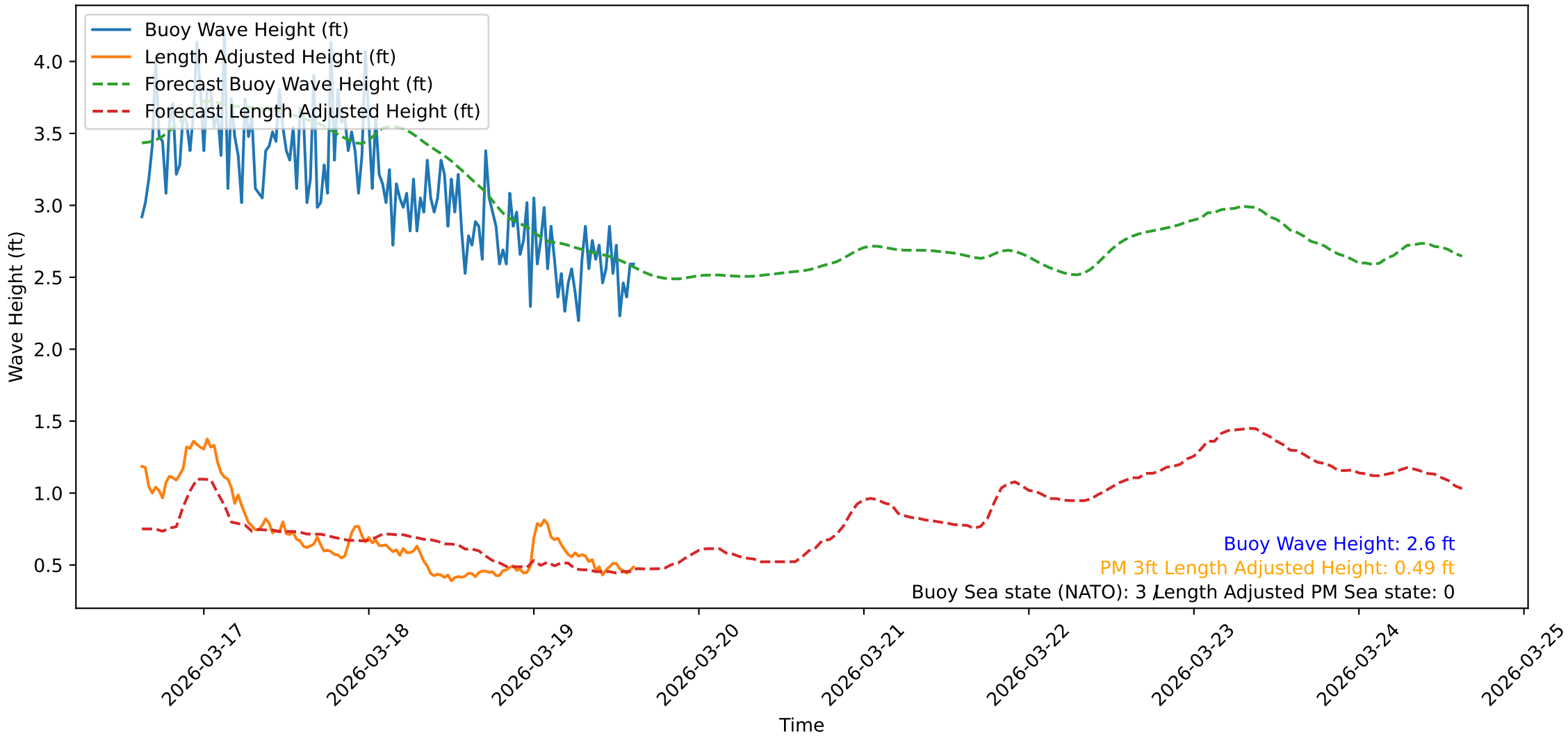
Wave Heights over Time for Green Beach at 2026-03-19 15:11:11
