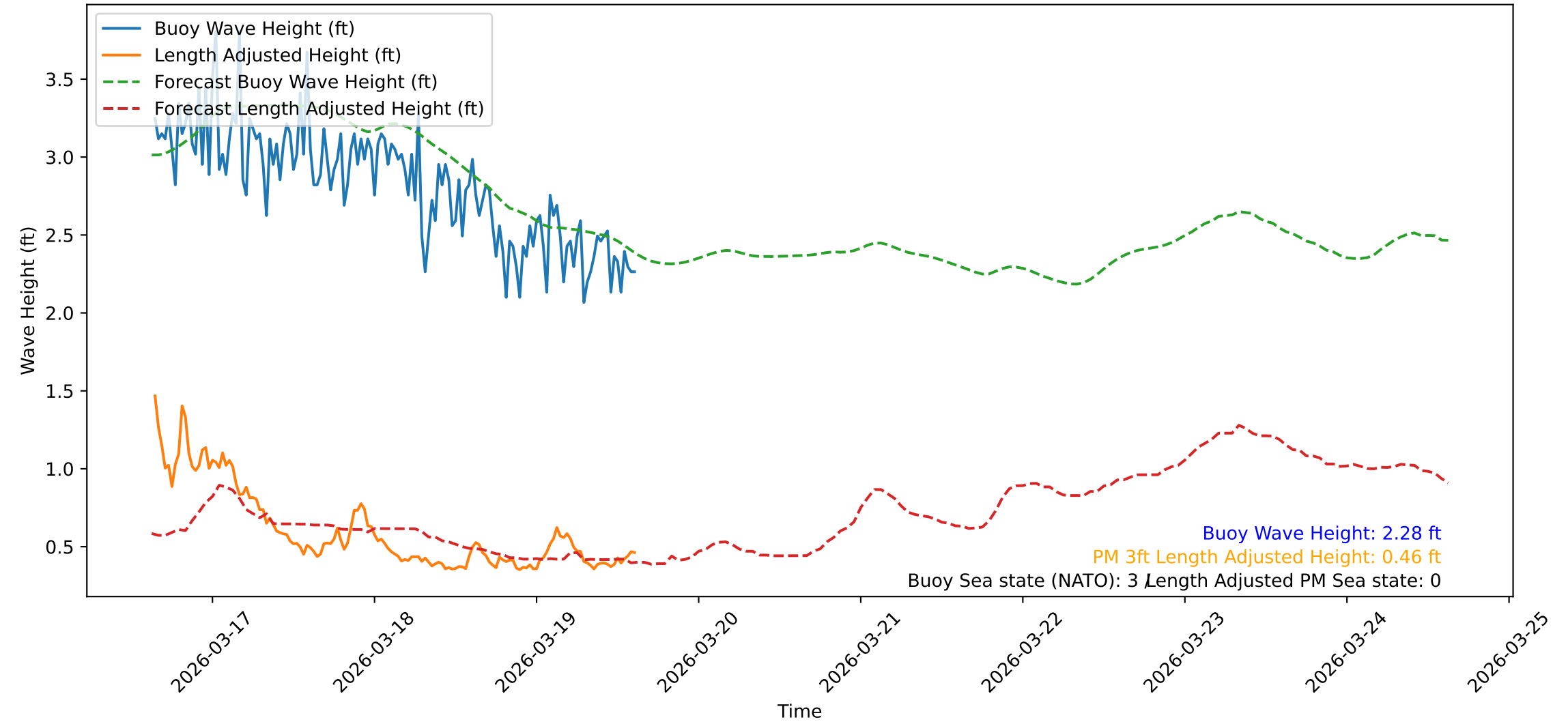
Wave Heights over Time for Red Beach at 2026-03-19 15:10:48
