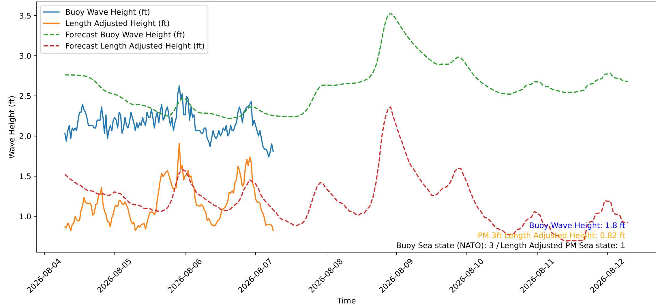
Wave Heights over Time for Green Beach at 2026-08-07 06:51:08
