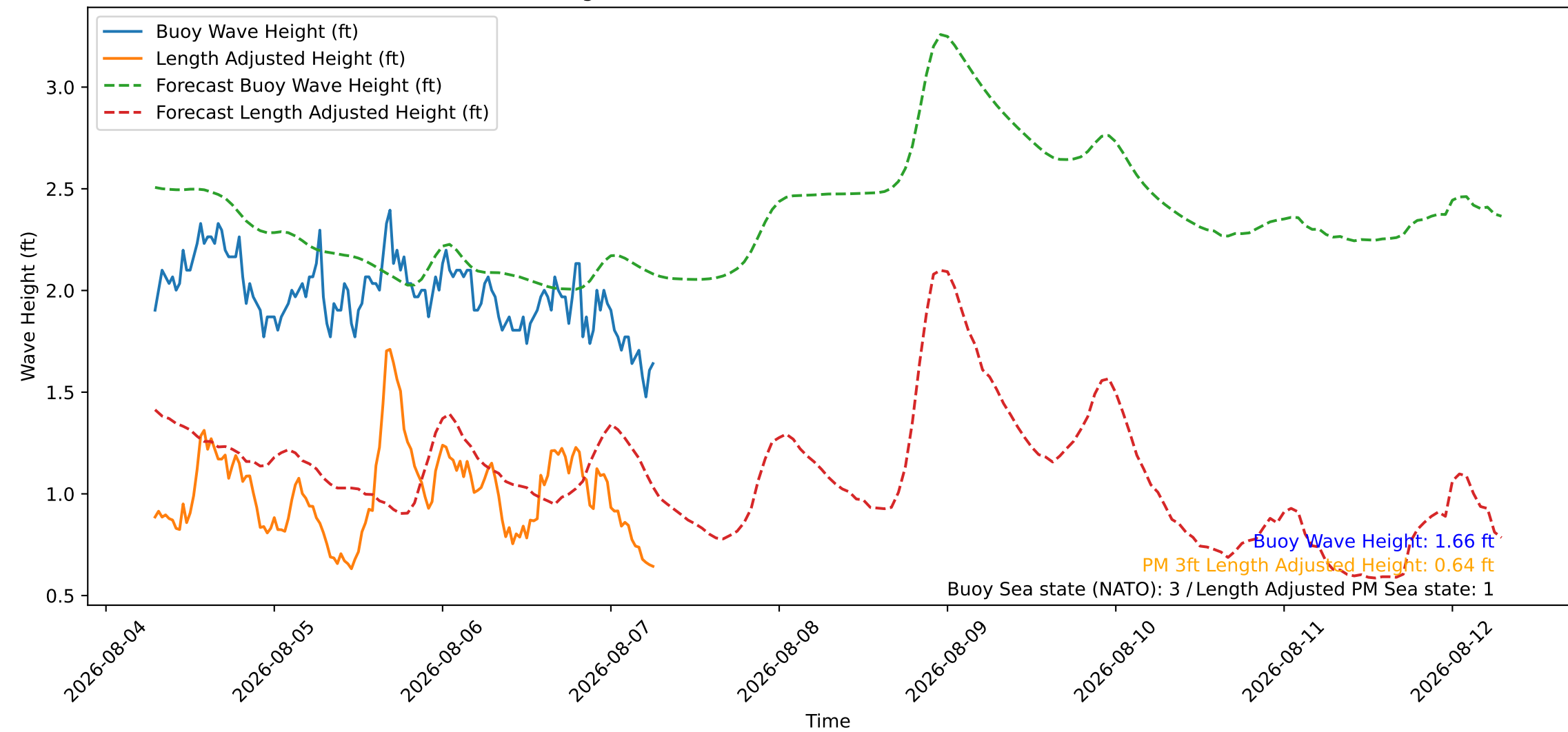
Wave Heights over Time for Red Beach at 2026-08-07 06:50:46
