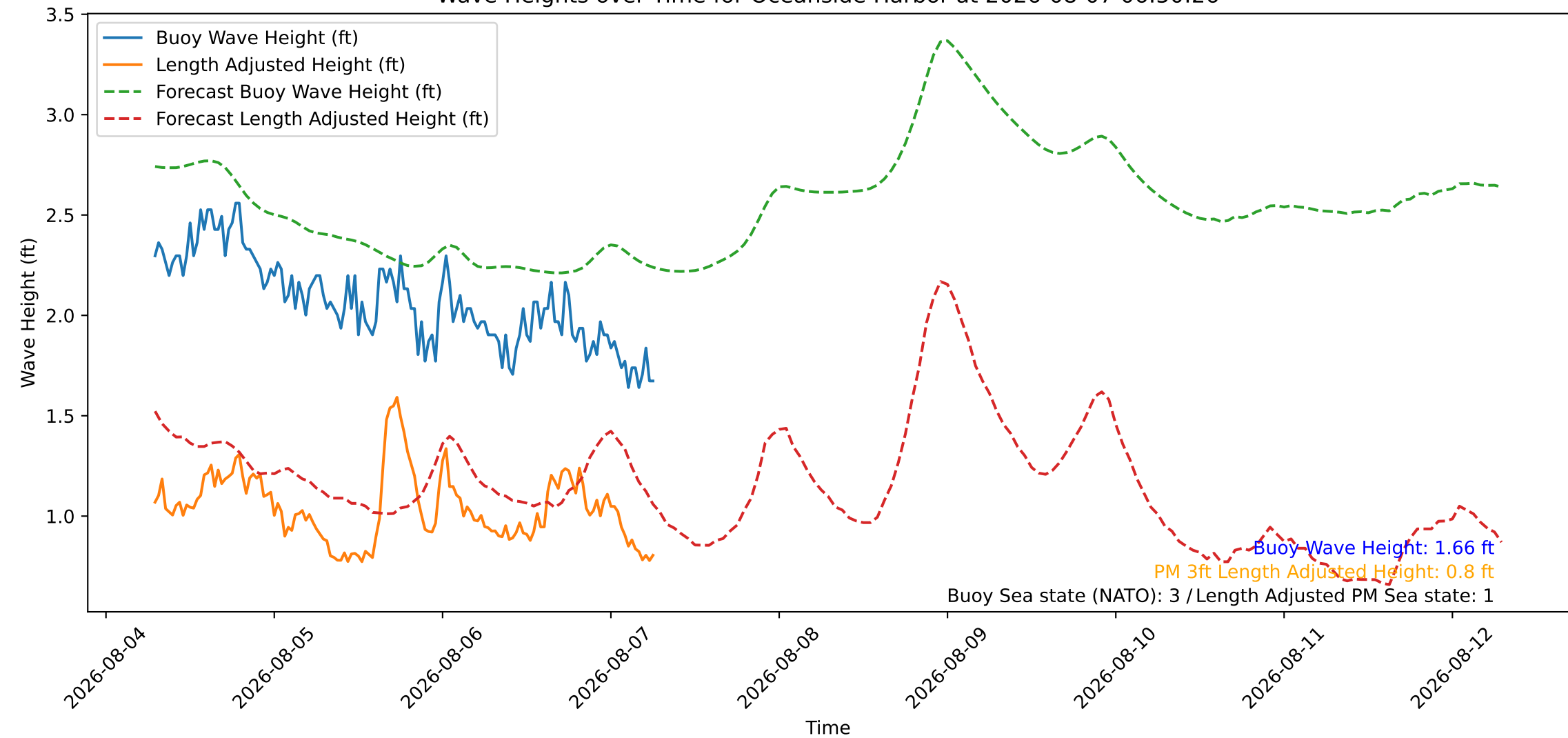
Wave Heights over Time for Oceanside Harbor at 2026-08-07 06:50:26
