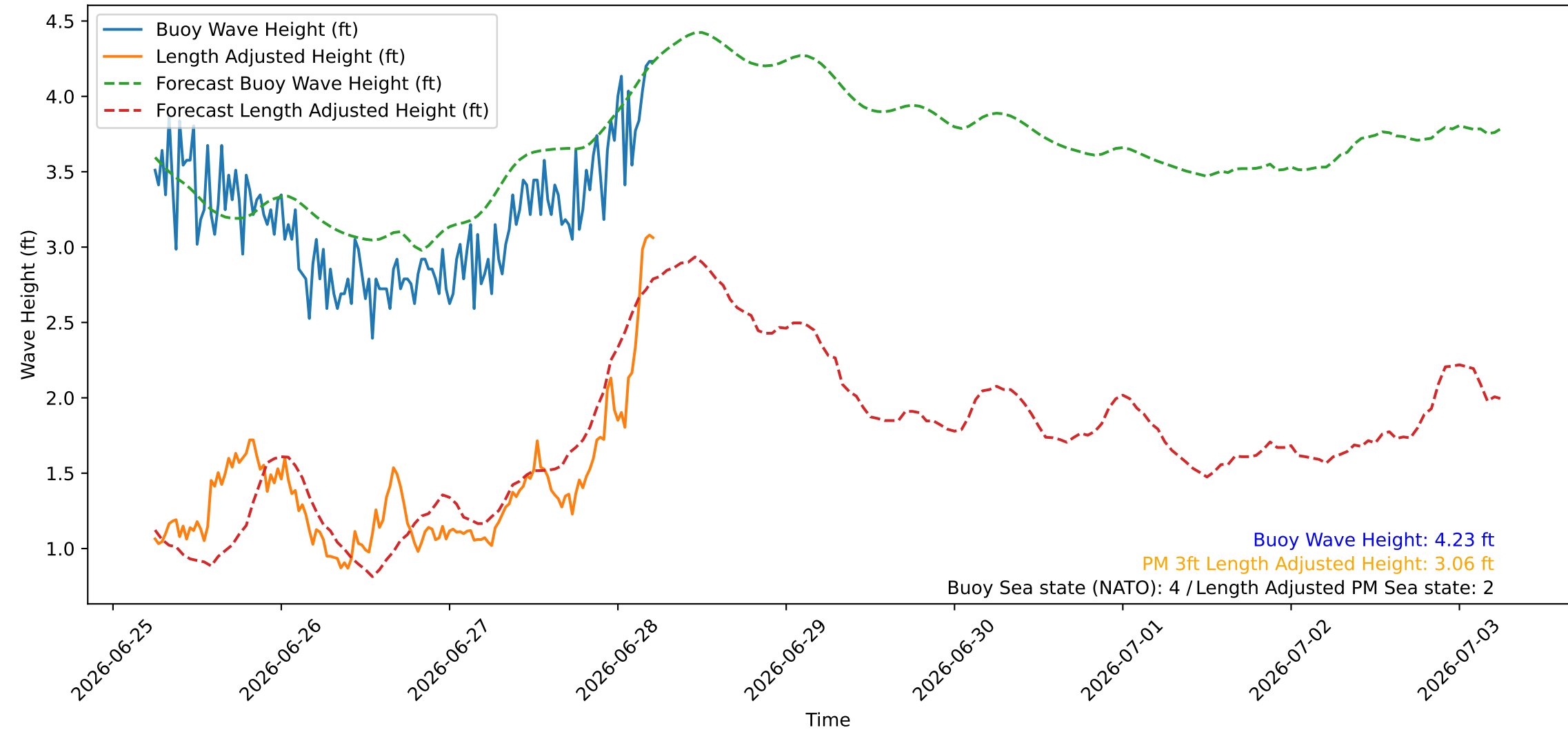
Wave Heights over Time for Oceanside Harbor at 2026-06-28 05:50:26
