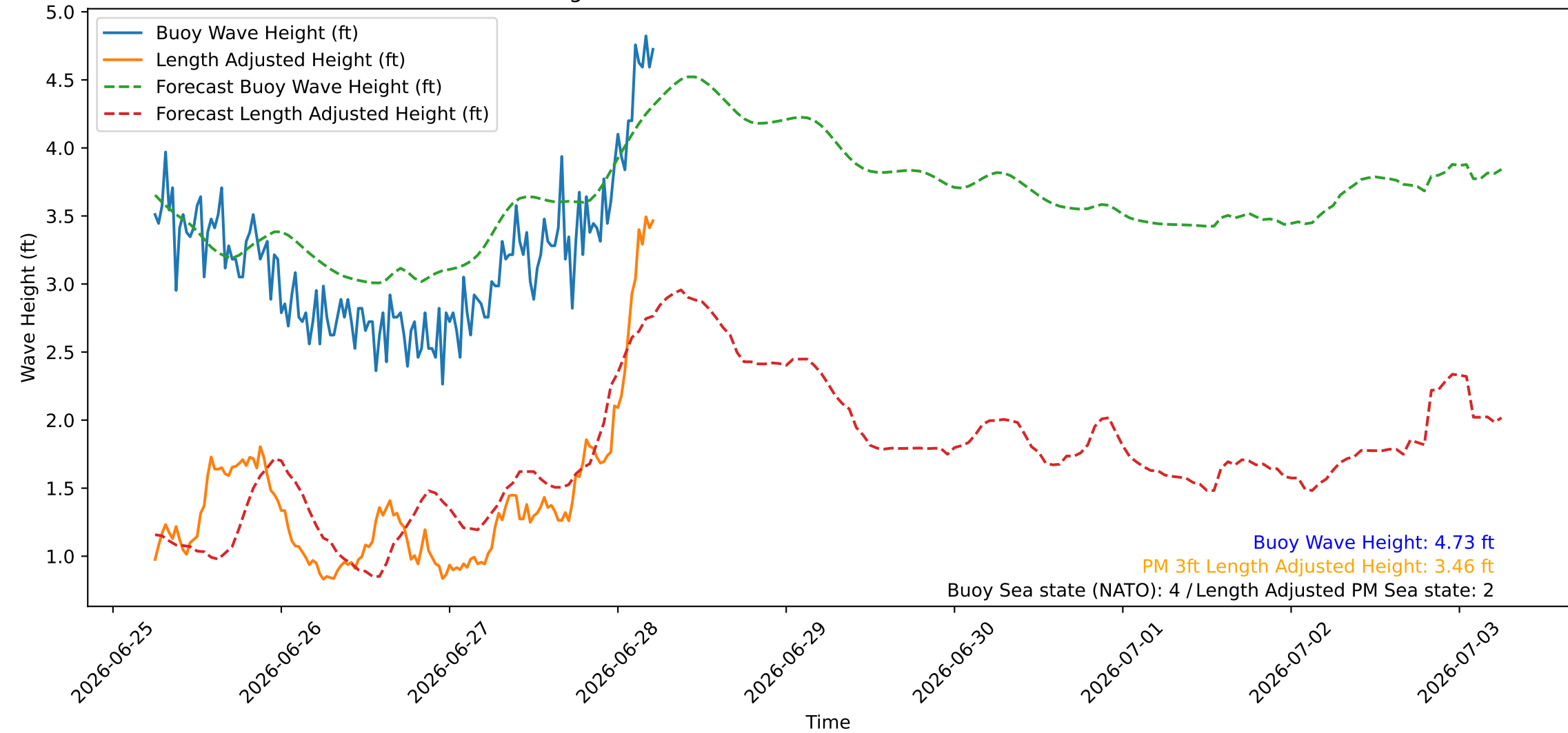
Wave Heights over Time for Green Beach at 2026-06-28 05:51:08
