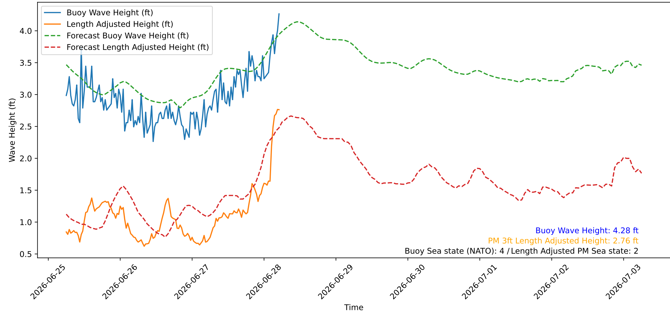
Wave Heights over Time for Red Beach at 2026-06-28 05:50:46
