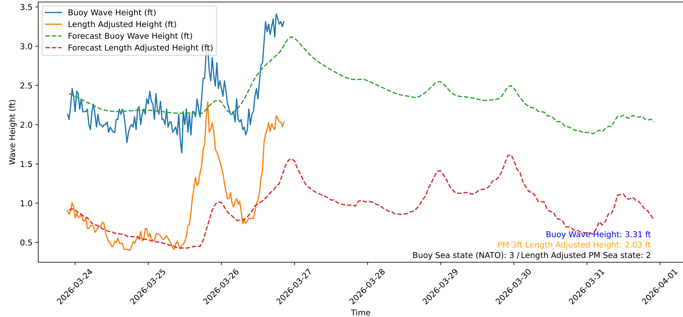
Wave Heights over Time for Green Beach at 2026-03-26 21:31:09
