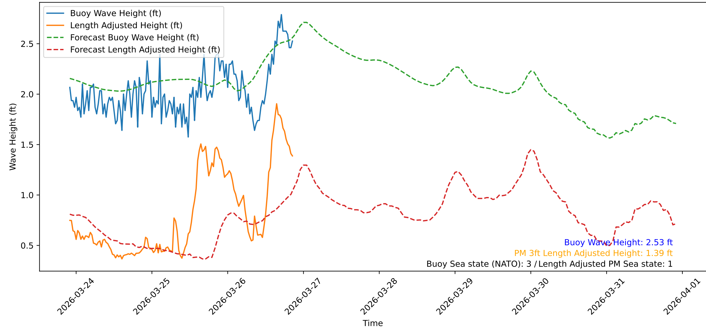
Wave Heights over Time for Red Beach at 2026-03-26 21:30:46
