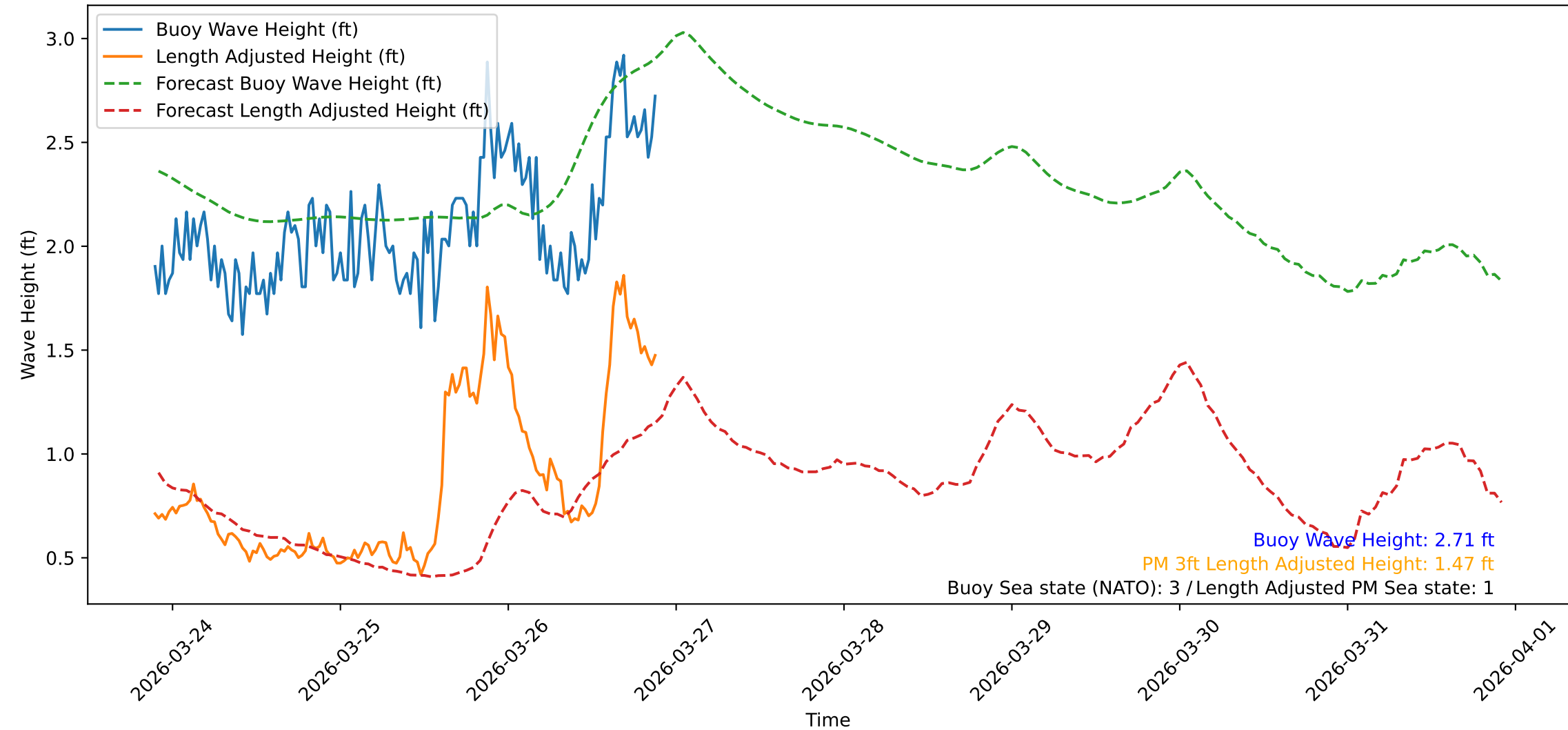
Wave Heights over Time for Oceanside Harbor at 2026-03-26 21:30:31
