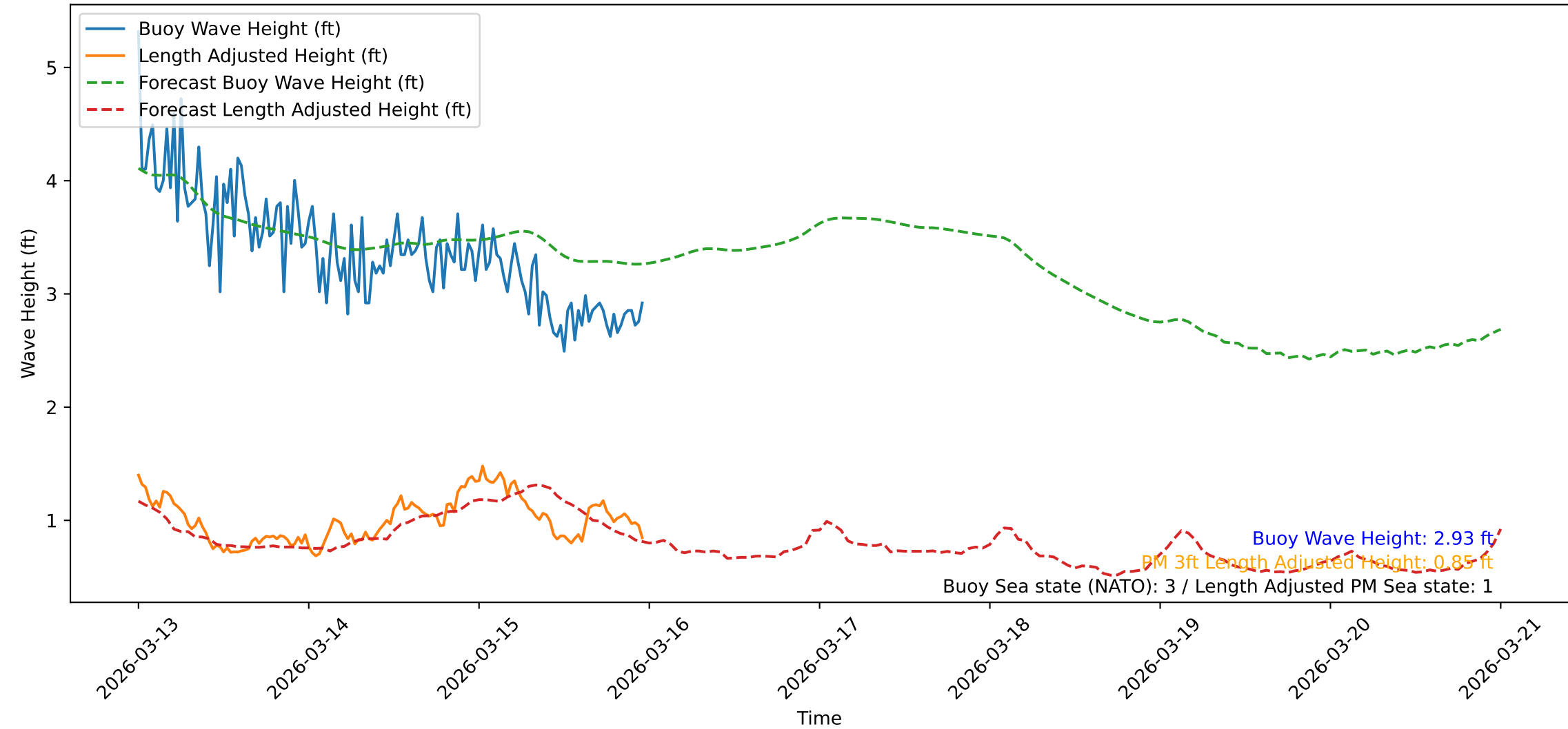
Wave Heights over Time for Oceanside Harbor at 2026-03-15 23:50:42
