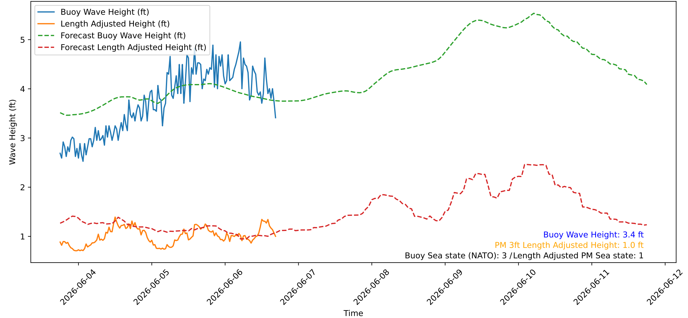
Wave Heights over Time for Red Beach at 2026-06-06 17:40:45
