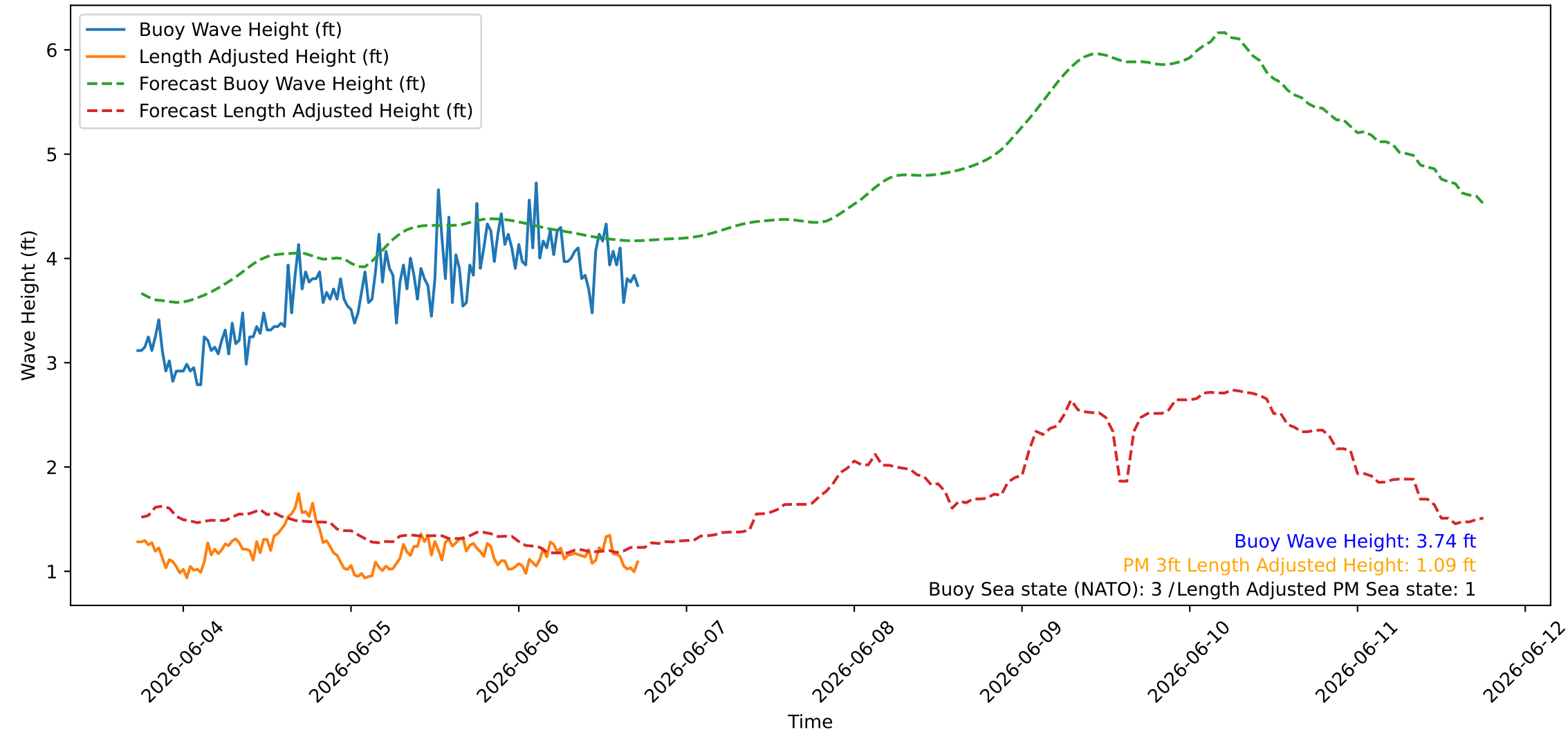
Wave Heights over Time for Green Beach at 2026-06-06 17:41:08
