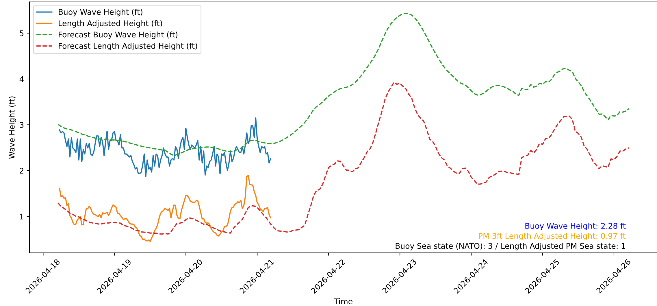
Wave Heights over Time for Green Beach at 2026-04-21 05:21:14
