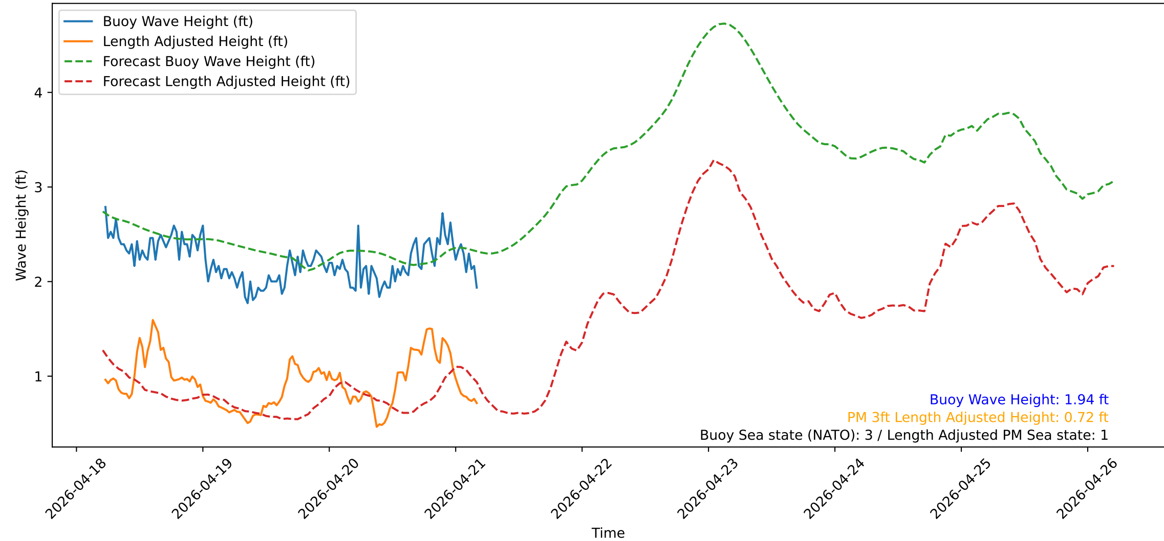
Wave Heights over Time for Red Beach at 2026-04-21 05:20:51
