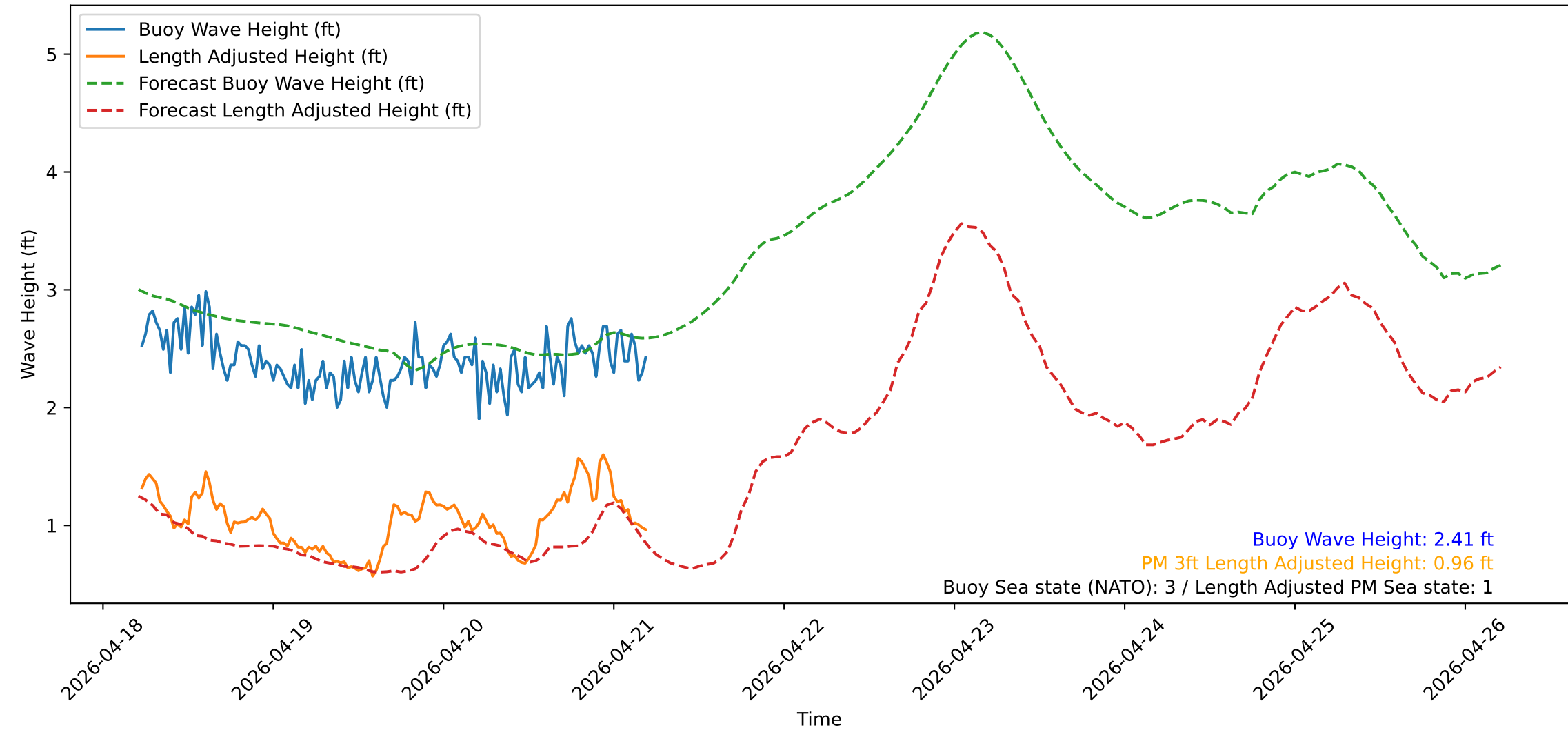
Wave Heights over Time for Oceanside Harbor at 2026-04-21 05:20:31
