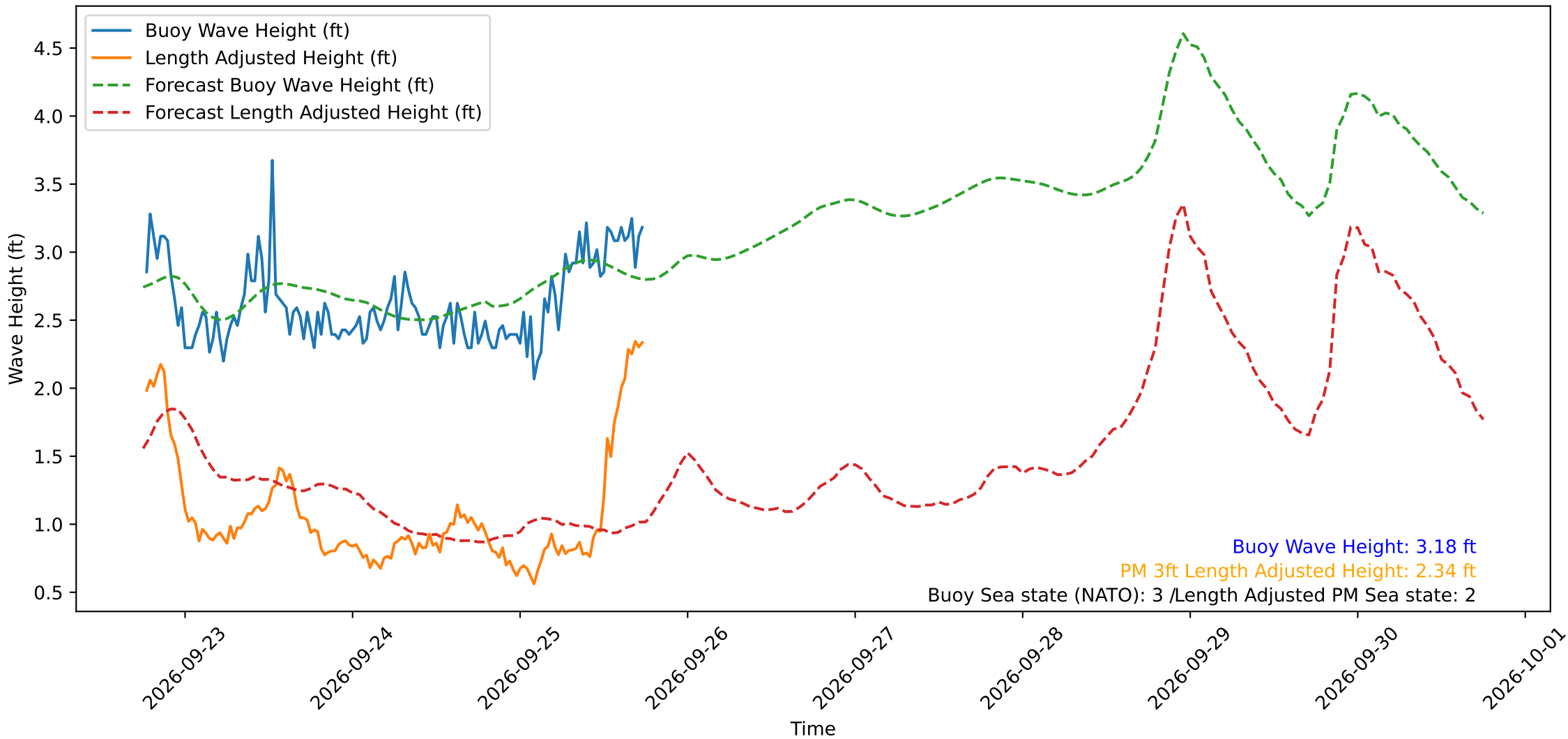
Wave Heights over Time for Red Beach at 2026-09-25 18:10:49
