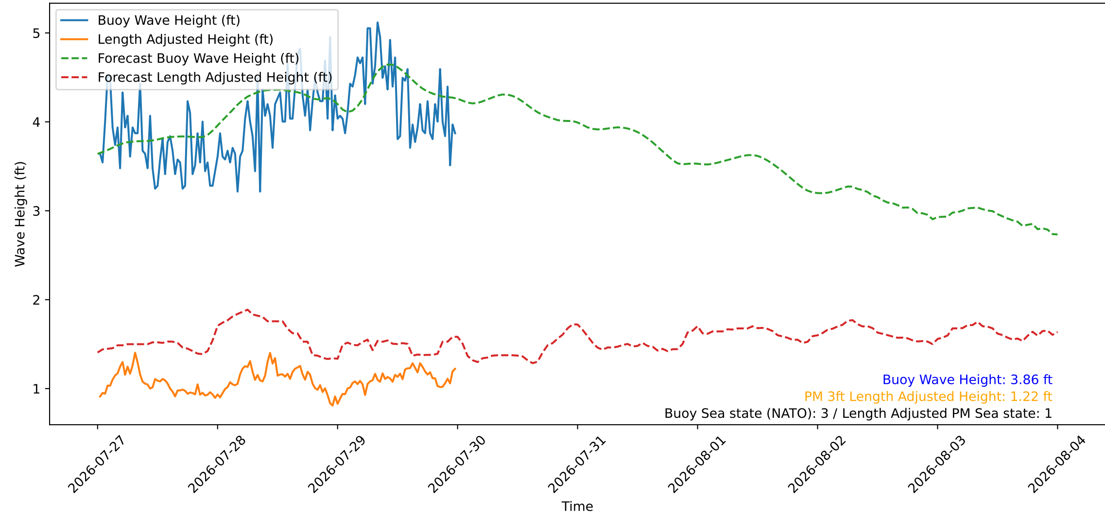
Wave Heights over Time for Red Beach at 2026-07-30 00:20:47
