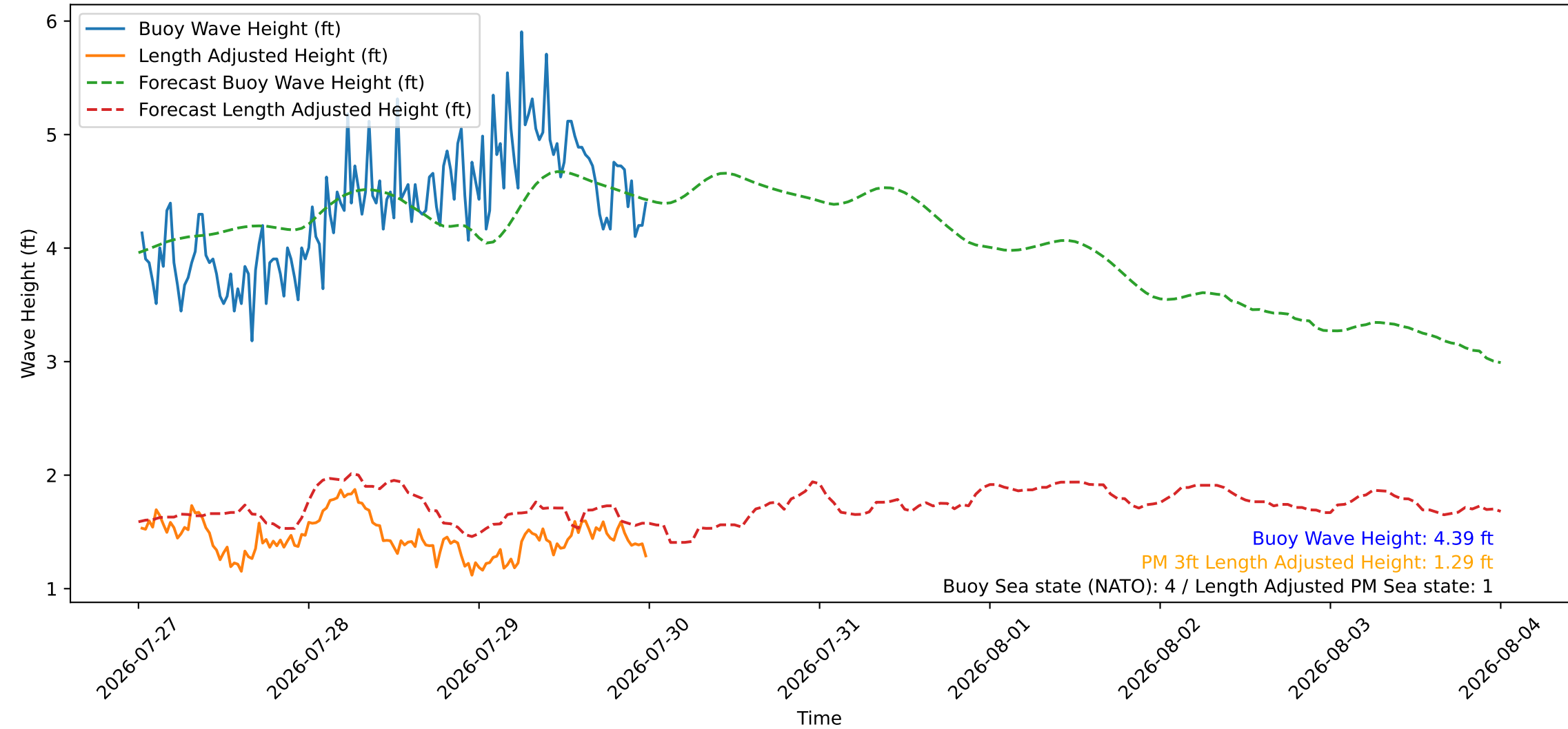
Wave Heights over Time for Oceanside Harbor at 2026-07-30 00:20:27
