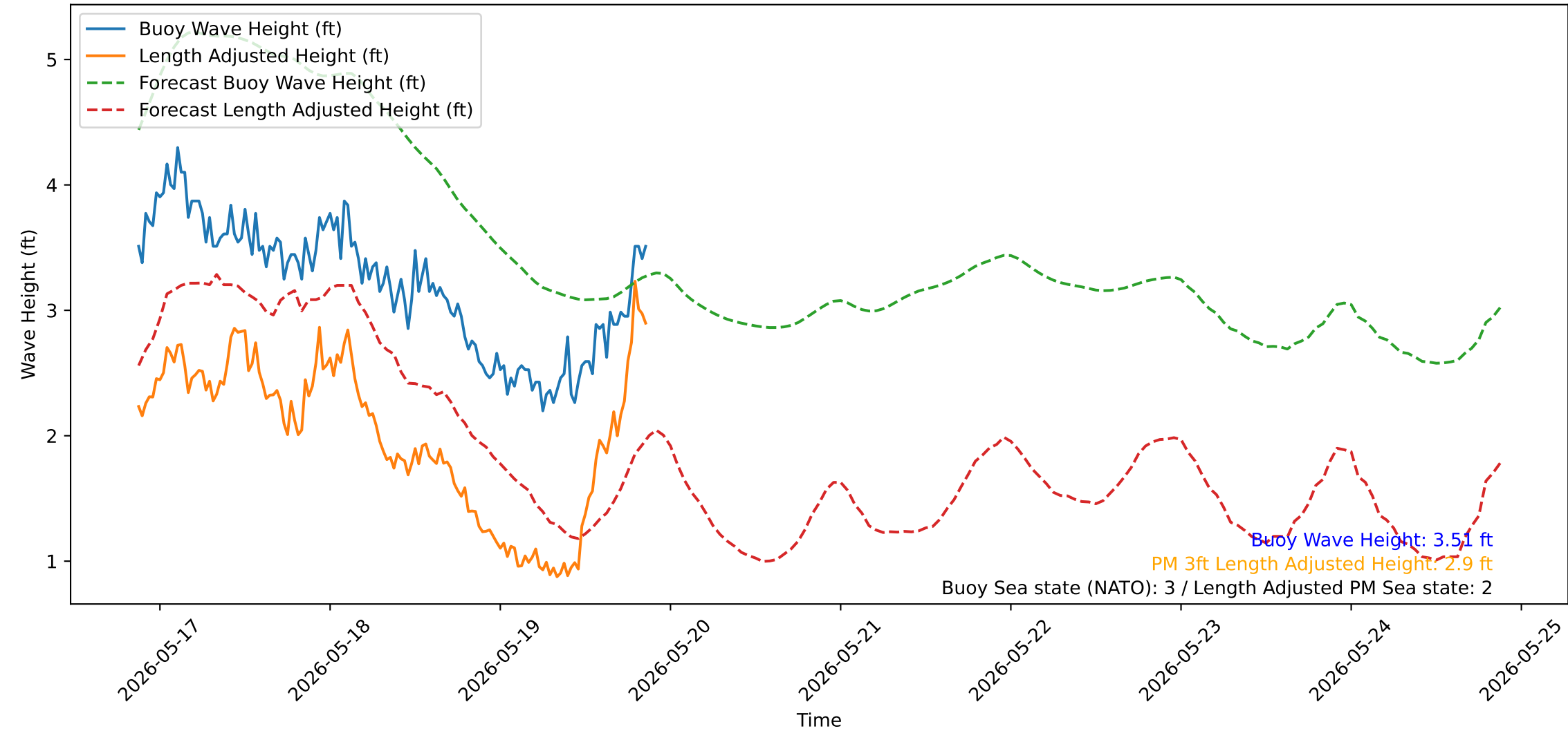
Wave Heights over Time for Oceanside Harbor at 2026-05-19 21:10:32
