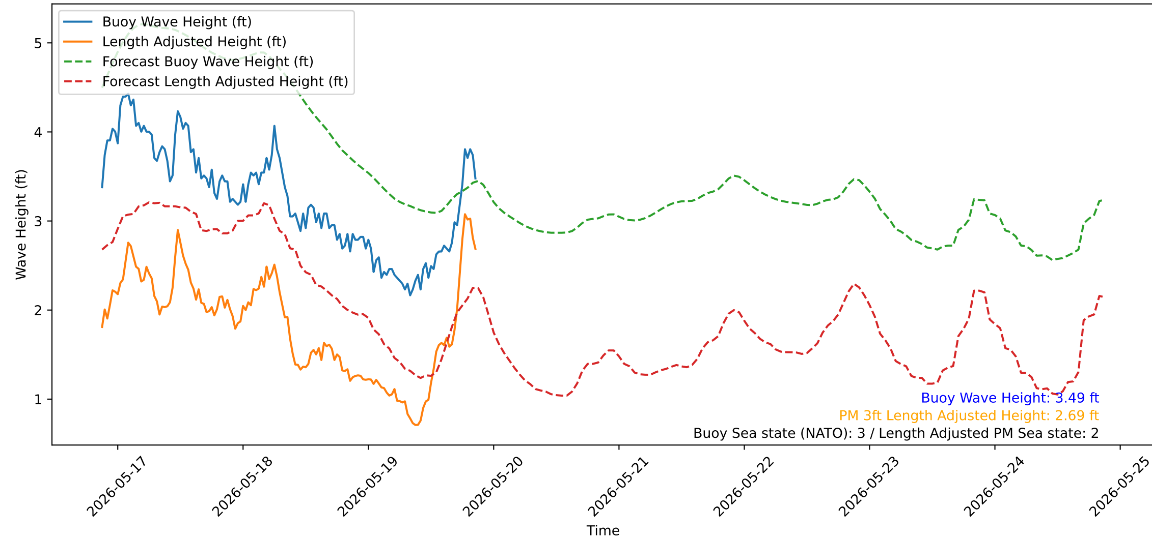
Wave Heights over Time for Green Beach at 2026-05-19 21:11:14
