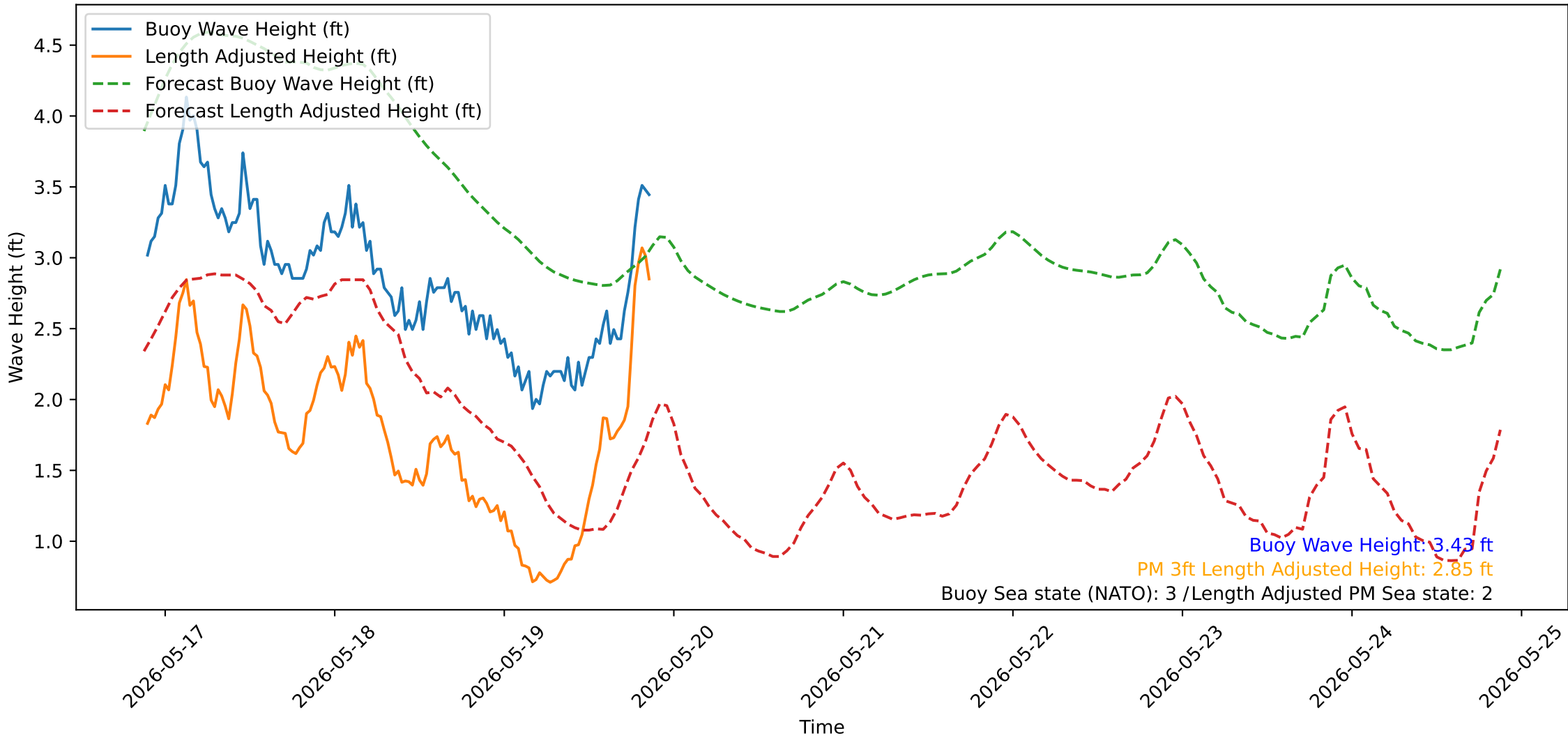
Wave Heights over Time for Red Beach at 2026-05-19 21:10:51
