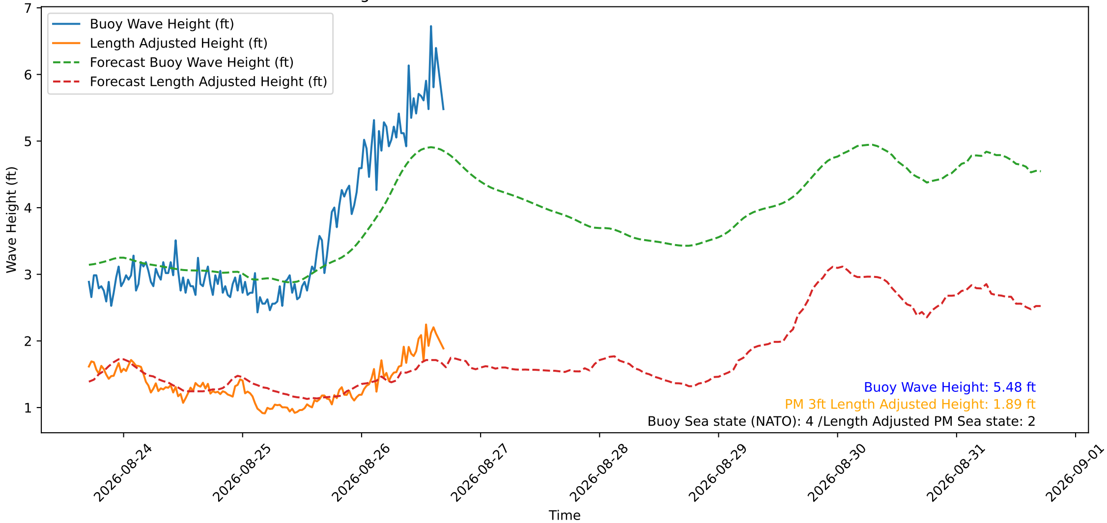
Wave Heights over Time for Oceanside Harbor at 2026-08-26 17:10:29
