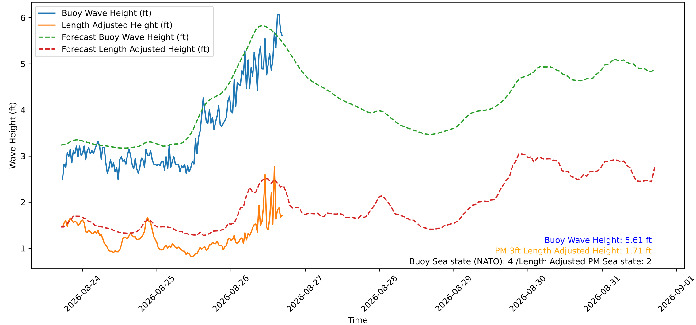
Wave Heights over Time for Green Beach at 2026-08-26 17:11:11
