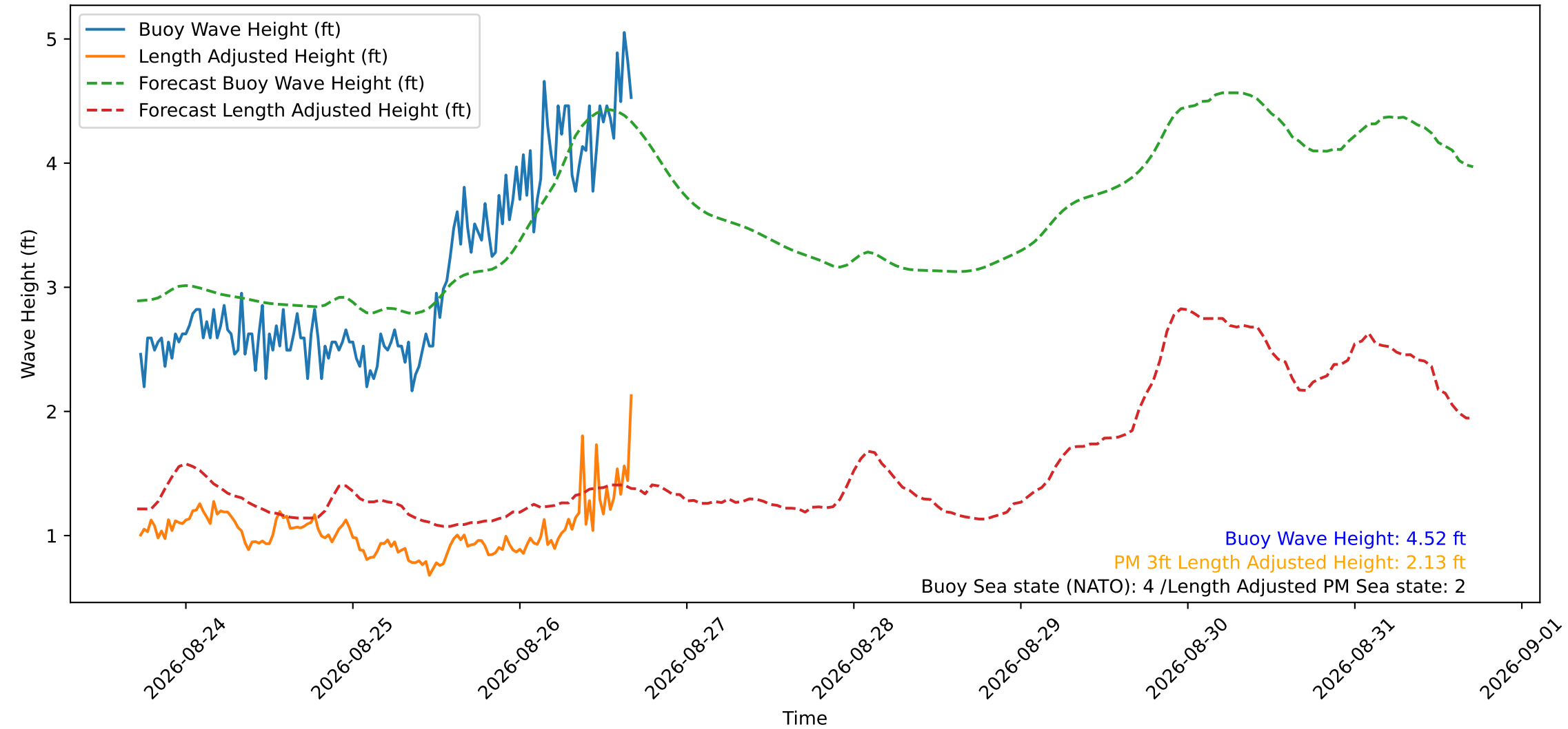
Wave Heights over Time for Red Beach at 2026-08-26 17:10:49
