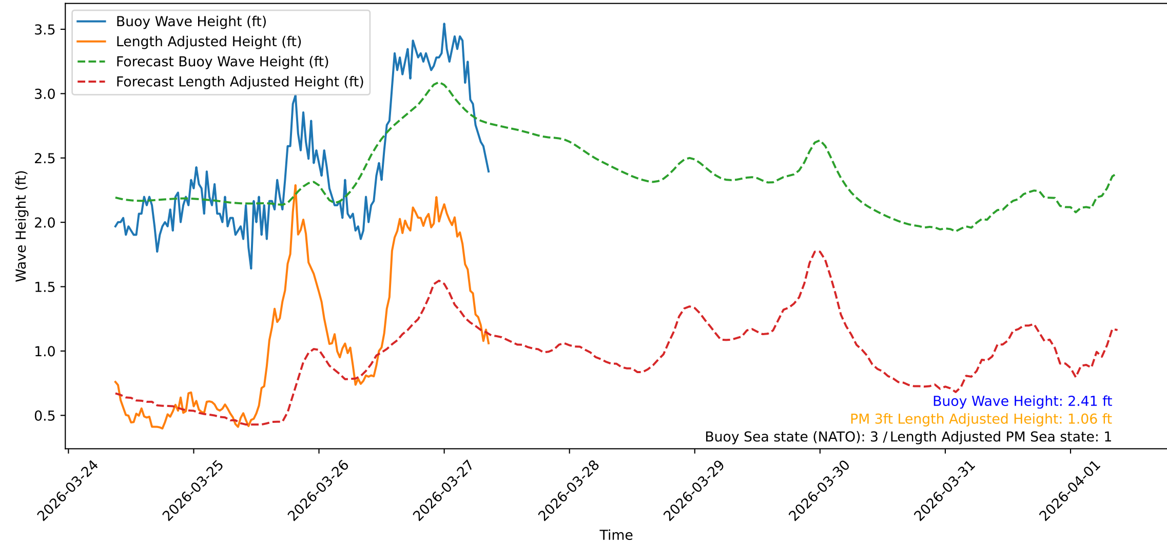
Wave Heights over Time for Green Beach at 2026-03-27 09:11:10
