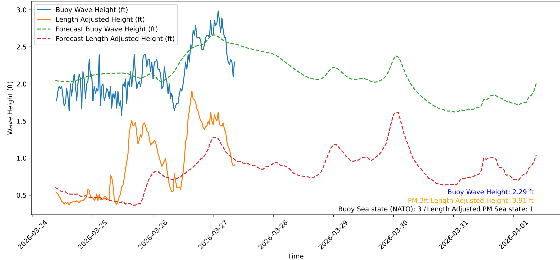
Wave Heights over Time for Red Beach at 2026-03-27 09:10:48
