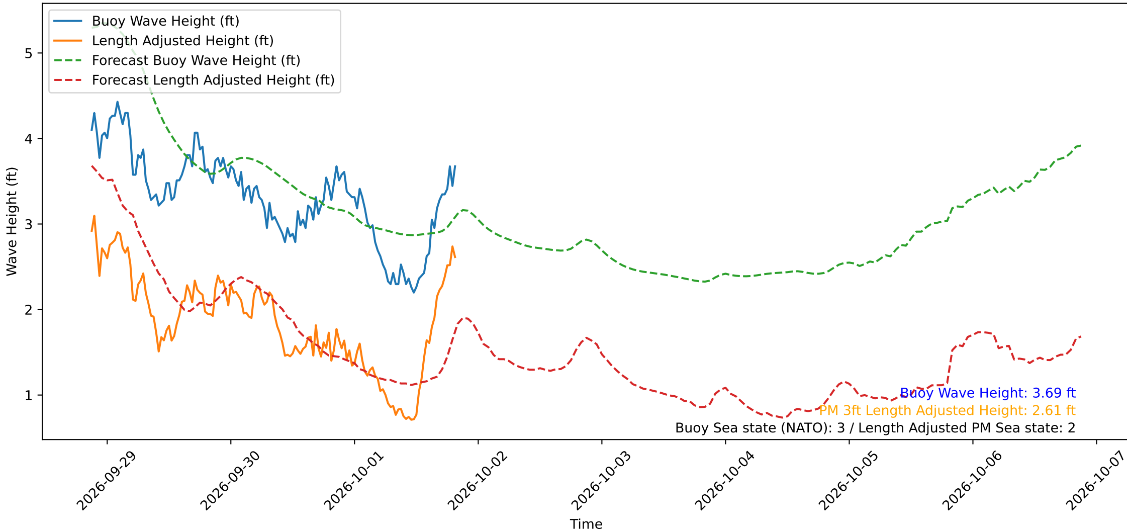
Wave Heights over Time for Green Beach at 2026-10-01 20:31:14
