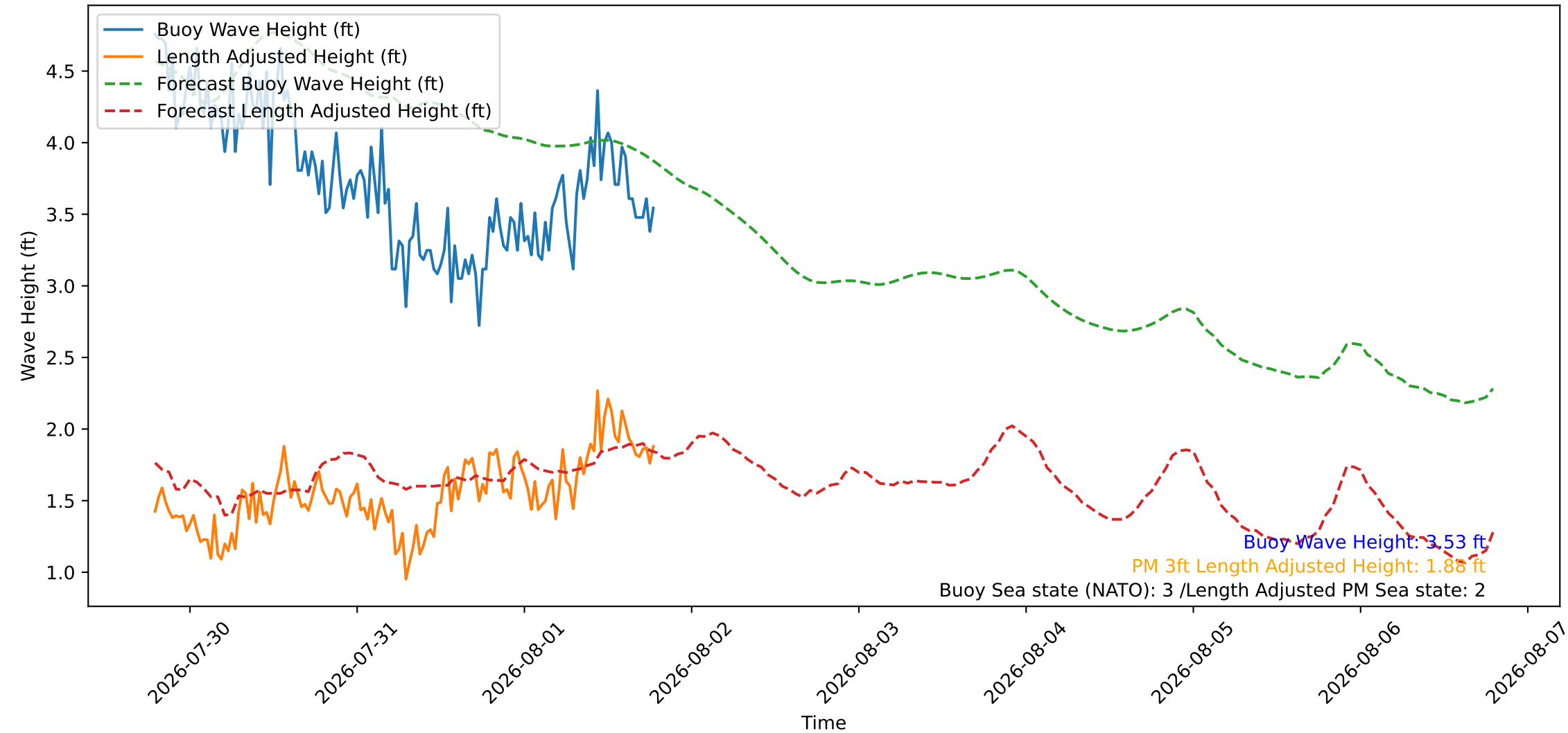
Wave Heights over Time for Oceanside Harbor at 2026-08-01 19:10:26
