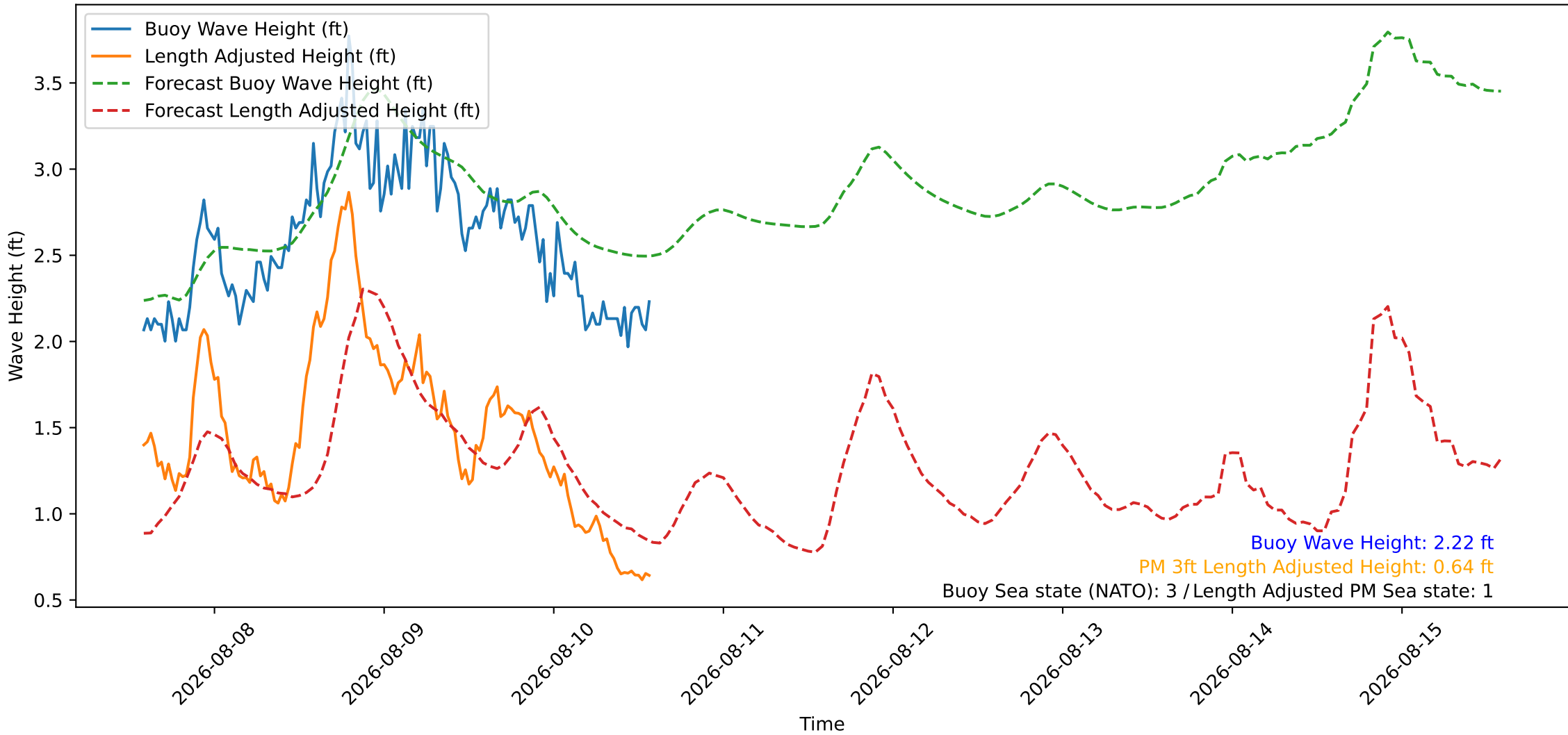
Wave Heights over Time for Green Beach at 2026-08-10 14:11:08
