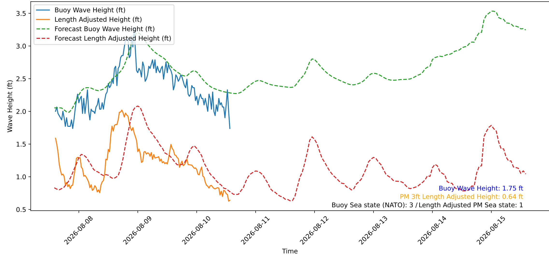
Wave Heights over Time for Red Beach at 2026-08-10 14:10:46
