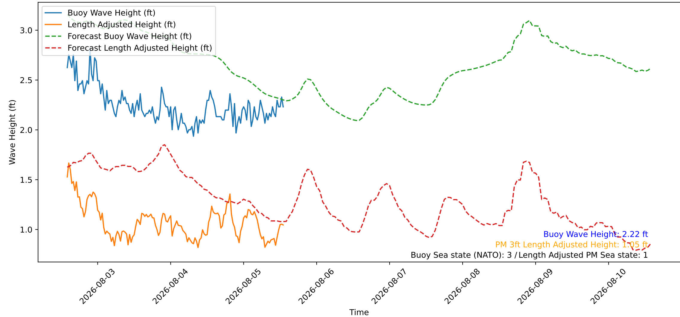
Wave Heights over Time for Green Beach at 2026-08-05 13:51:10
