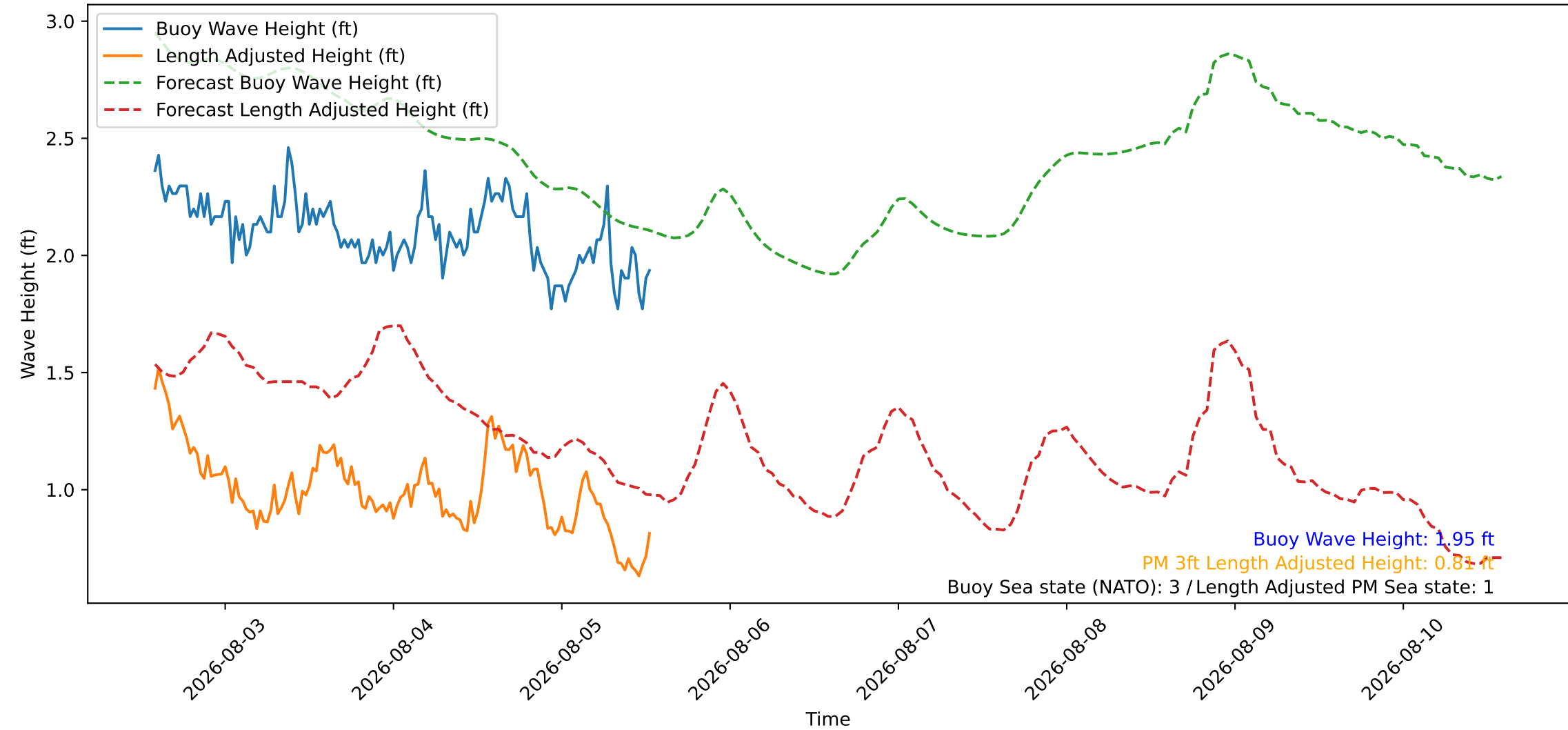
Wave Heights over Time for Red Beach at 2026-08-05 13:50:47
