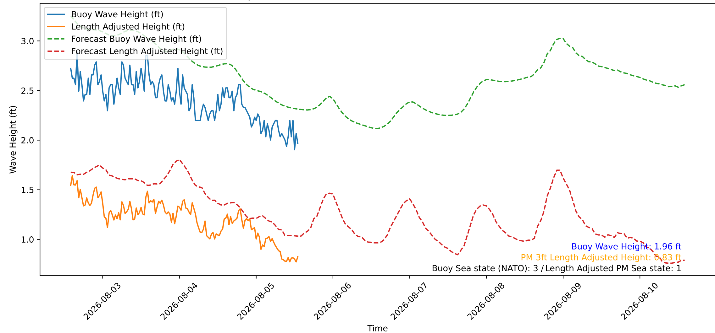
Wave Heights over Time for Oceanside Harbor at 2026-08-05 13:50:27
