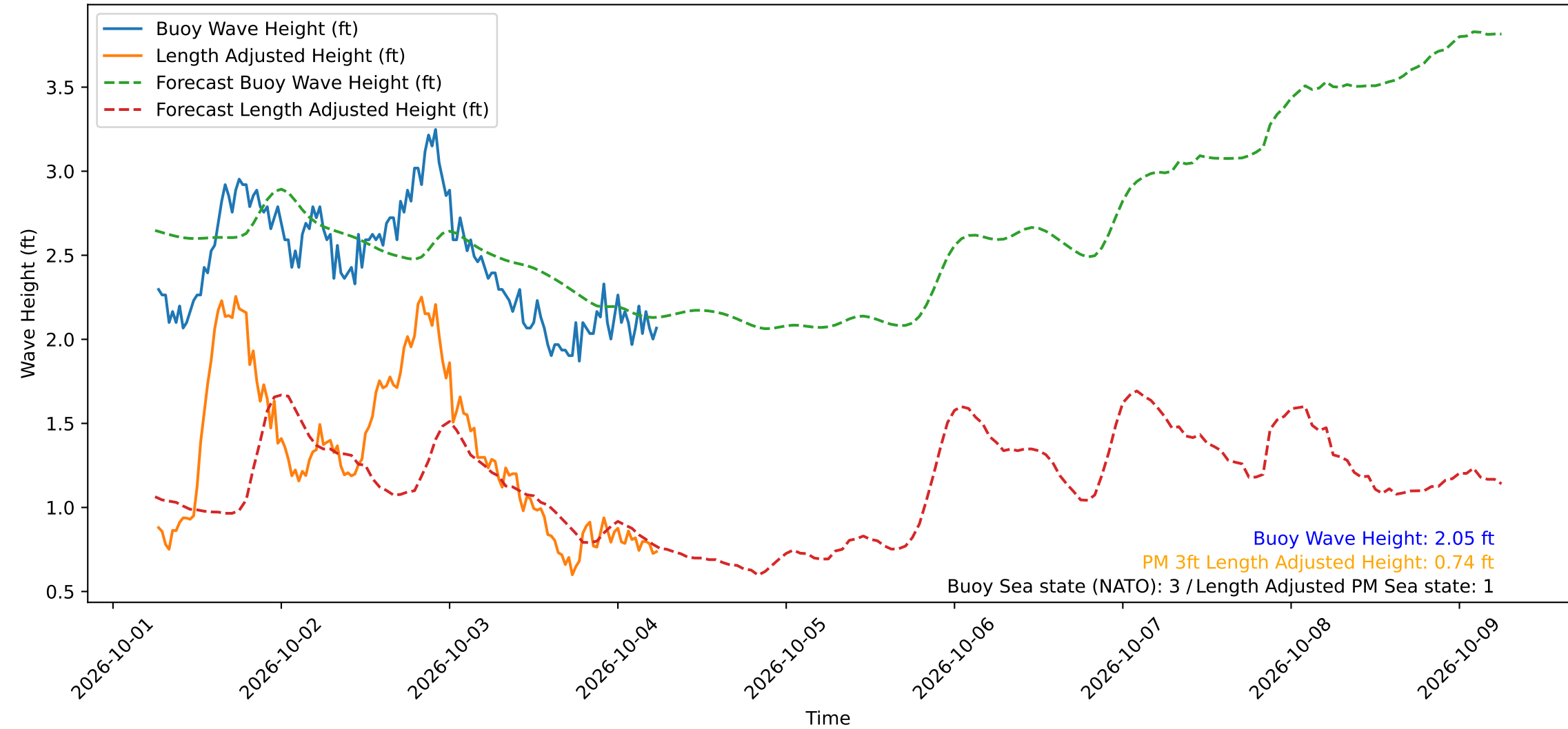
Wave Heights over Time for Red Beach at 2026-10-04 06:10:50
