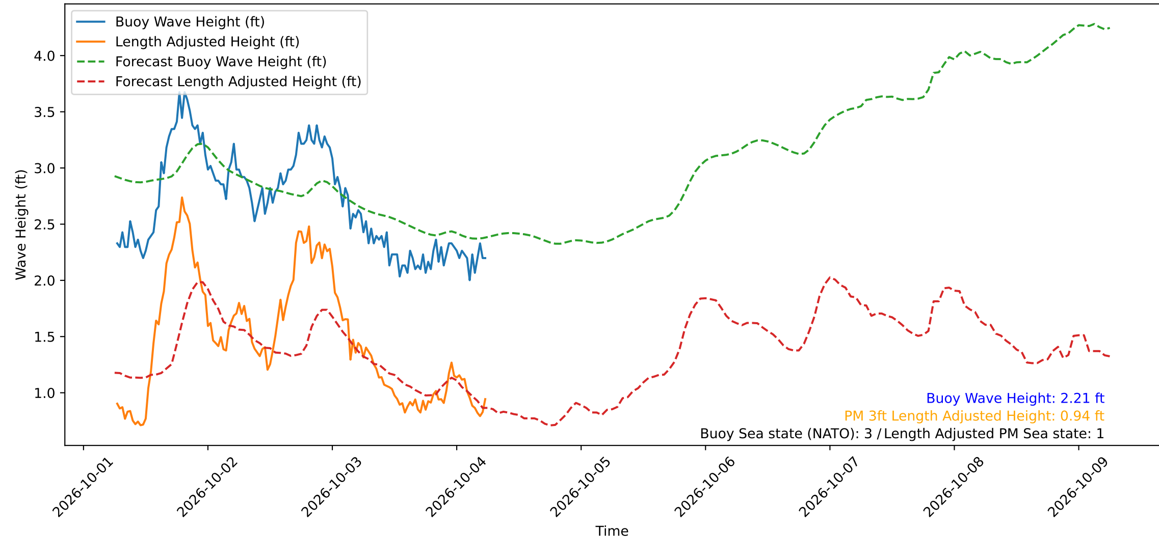
Wave Heights over Time for Green Beach at 2026-10-04 06:11:13
