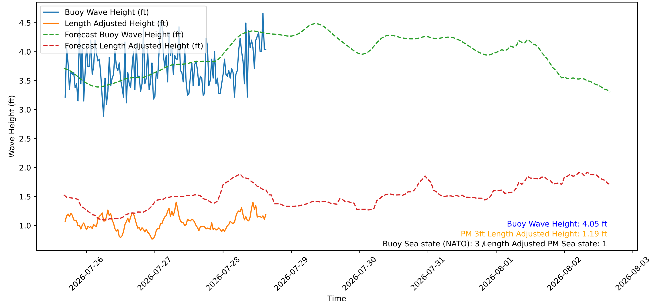
Wave Heights over Time for Red Beach at 2026-07-28 16:00:45
