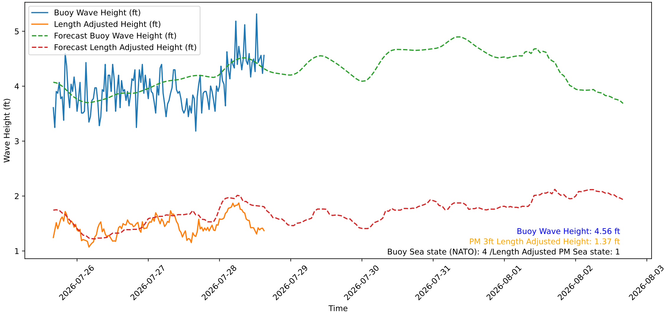
Wave Heights over Time for Oceanside Harbor at 2026-07-28 16:00:26
