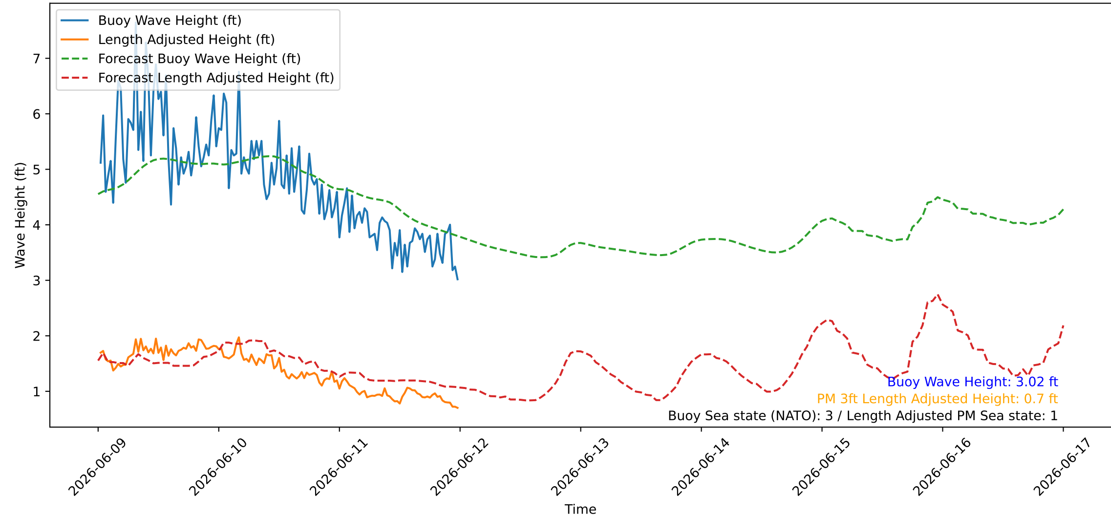
Wave Heights over Time for Red Beach at 2026-06-12 00:10:45
