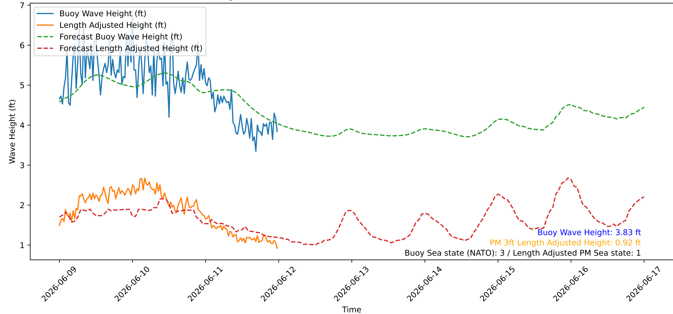
Wave Heights over Time for Oceanside Harbor at 2026-06-12 00:10:26
