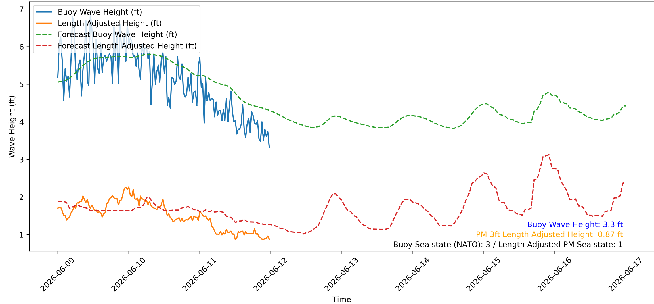
Wave Heights over Time for Green Beach at 2026-06-12 00:11:08
