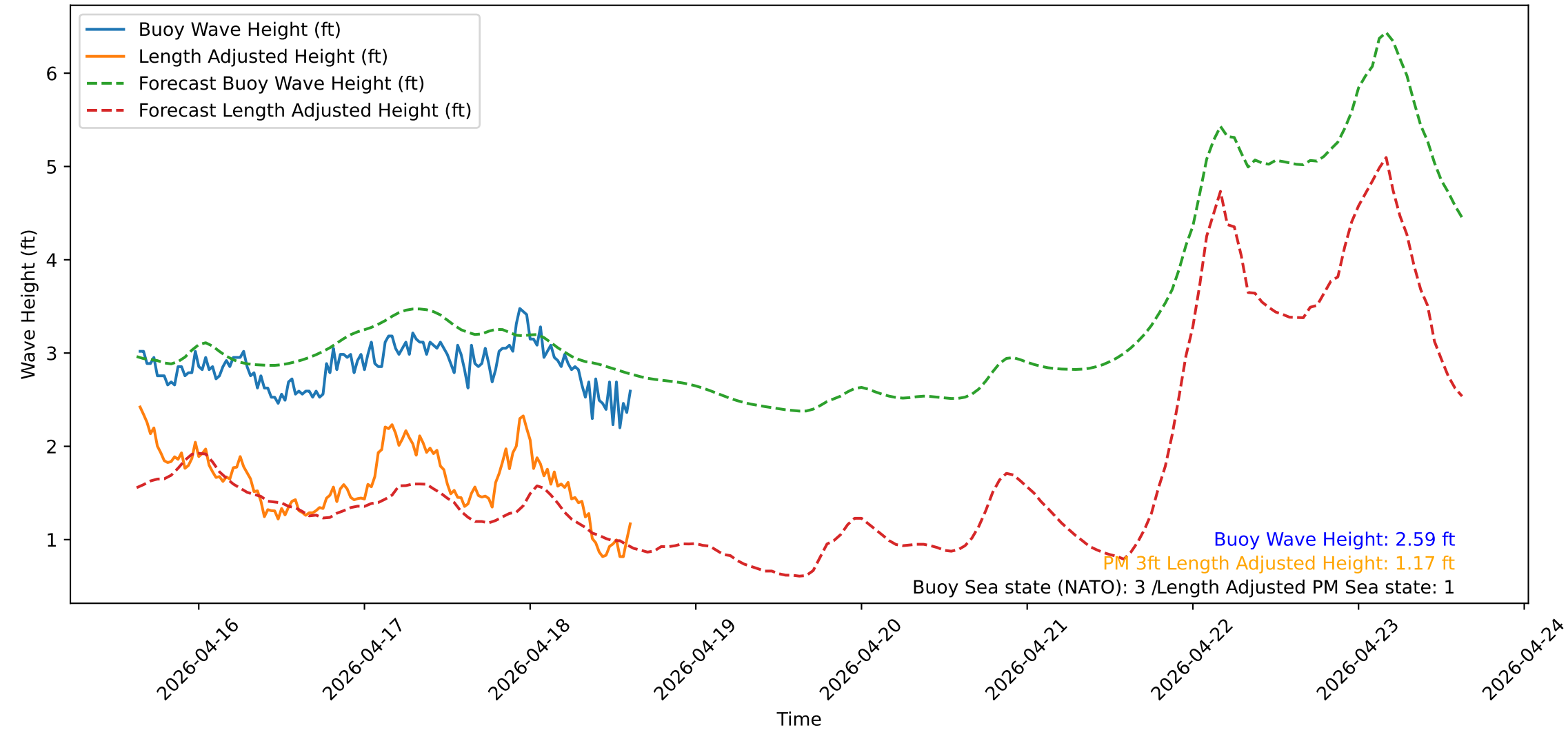
Wave Heights over Time for Green Beach at 2026-04-18 15:21:13
