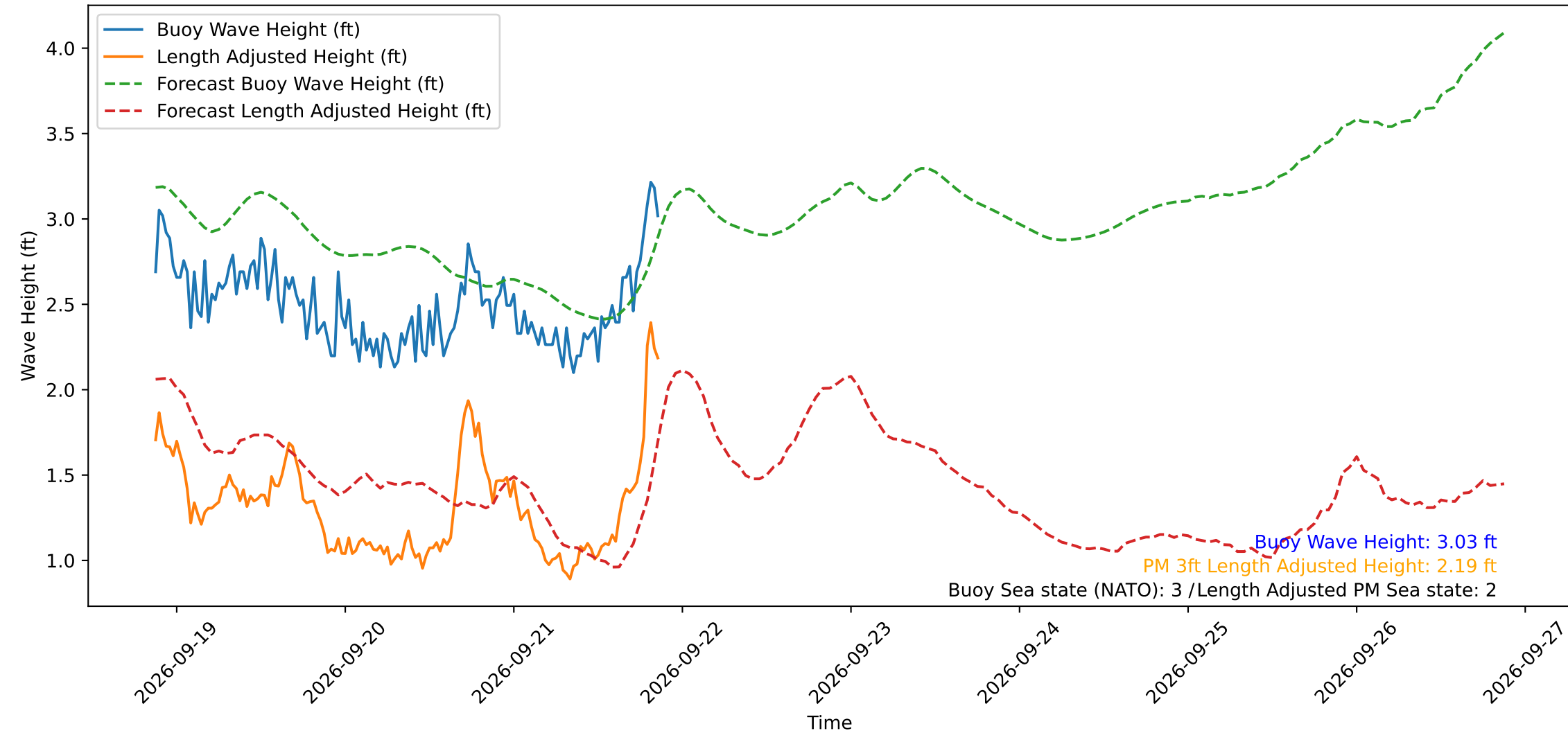
Wave Heights over Time for Oceanside Harbor at 2026-09-21 21:10:29
