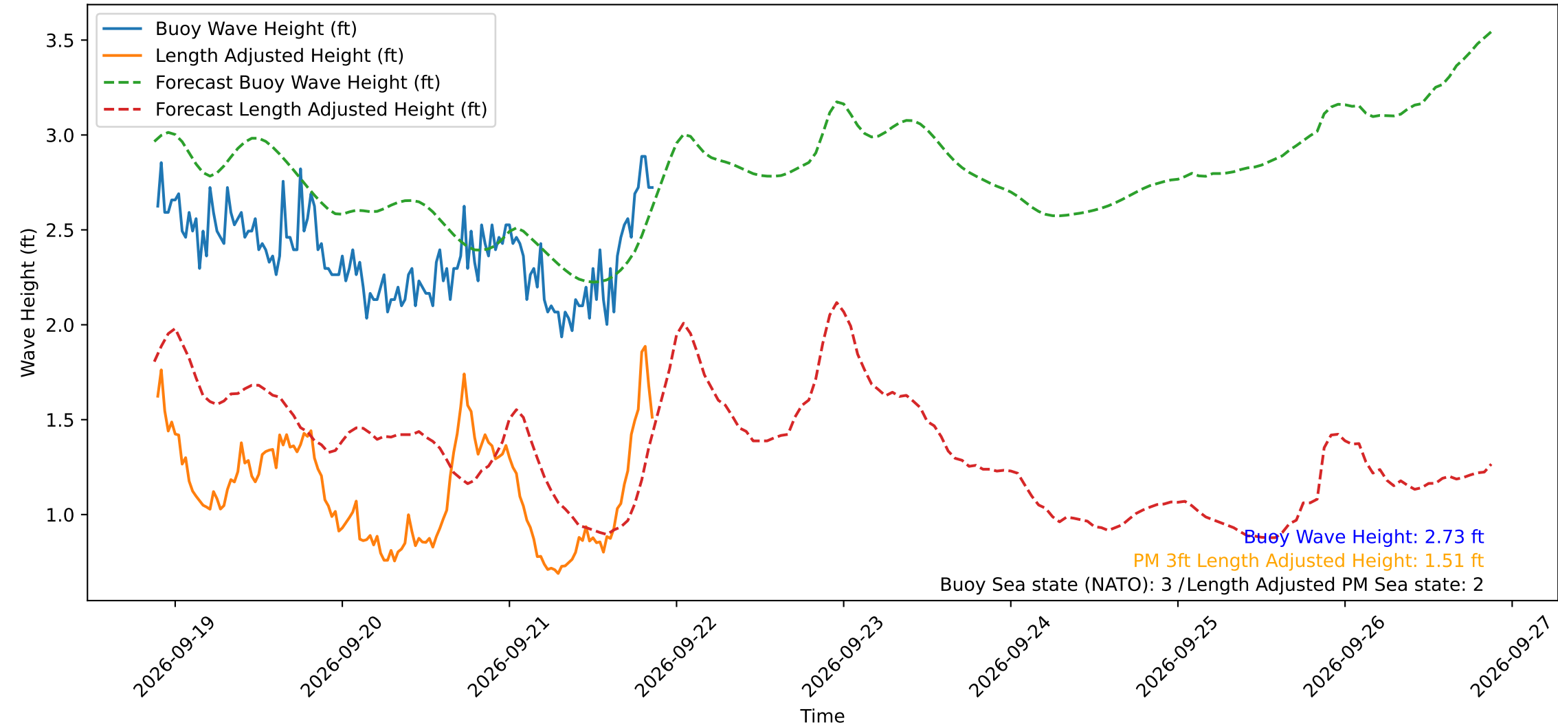
Wave Heights over Time for Red Beach at 2026-09-21 21:10:49
