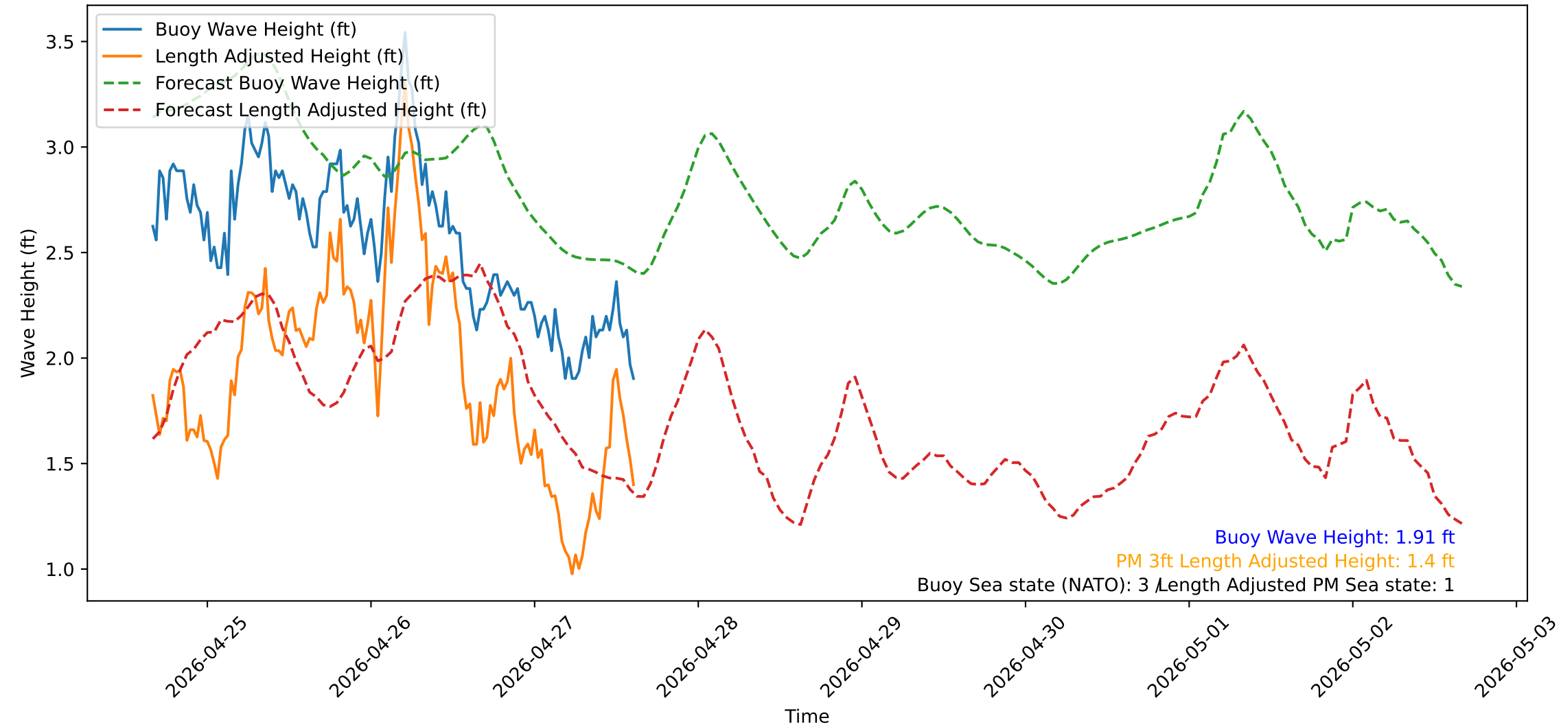
Wave Heights over Time for Red Beach at 2026-04-27 15:30:50
