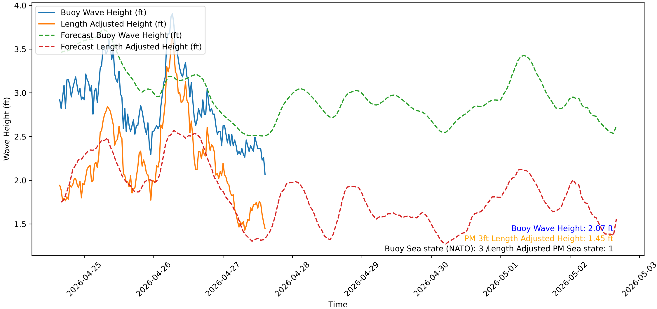
Wave Heights over Time for Oceanside Harbor at 2026-04-27 15:30:31
