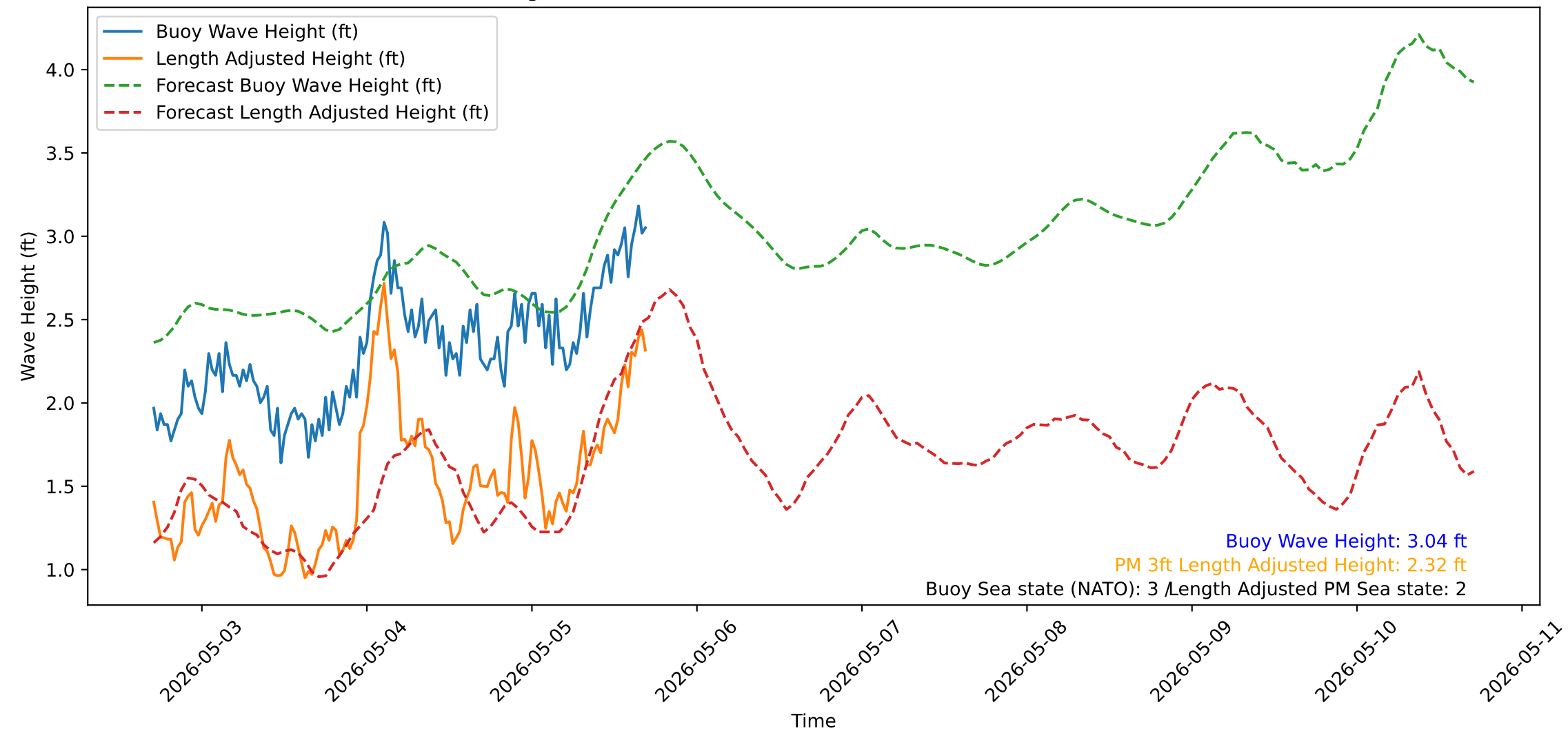
Wave Heights over Time for Oceanside Harbor at 2026-05-05 17:10:31
