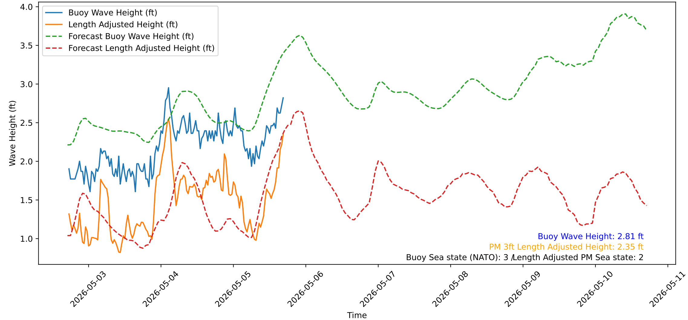
Wave Heights over Time for Red Beach at 2026-05-05 17:10:50
