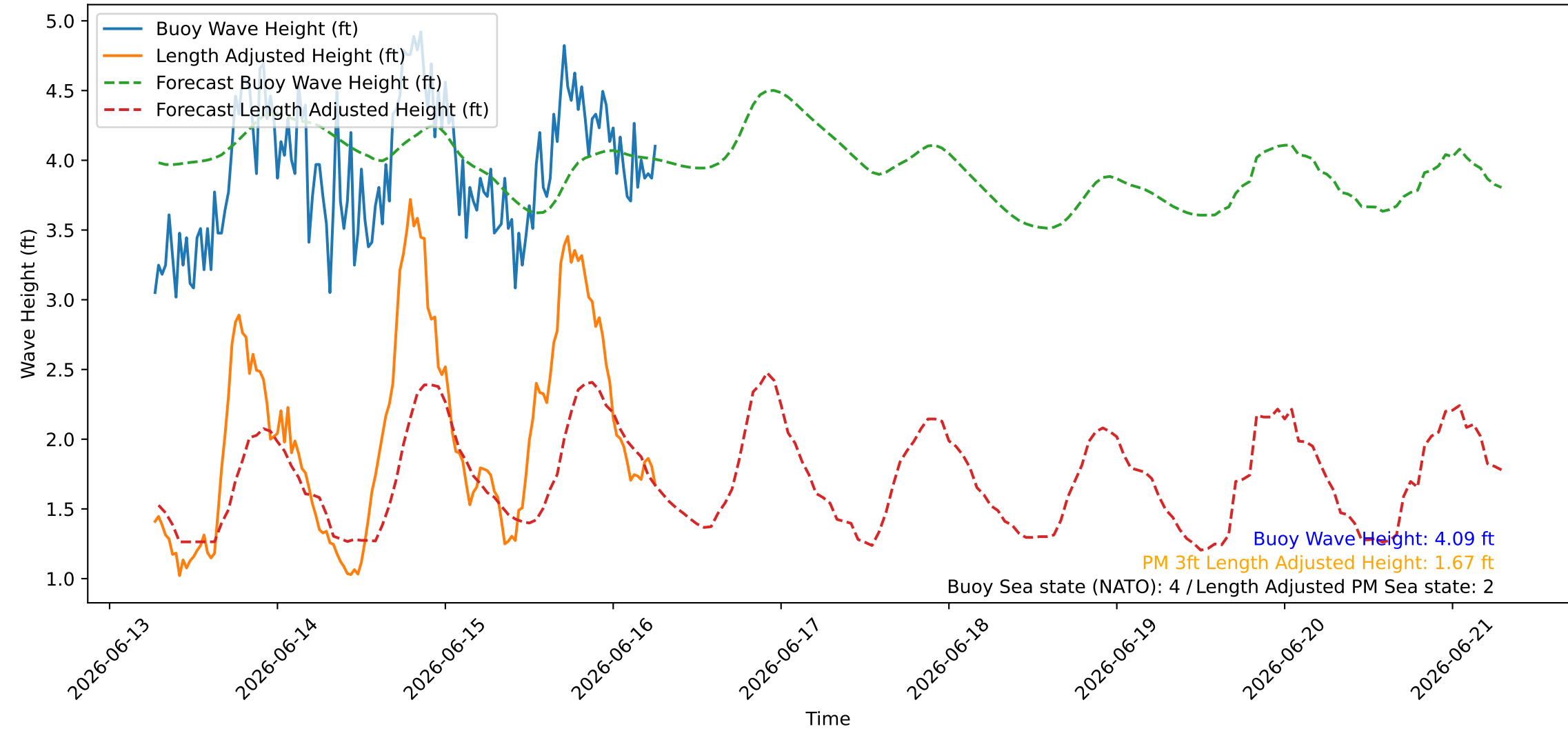
Wave Heights over Time for Green Beach at 2026-06-16 06:41:08
