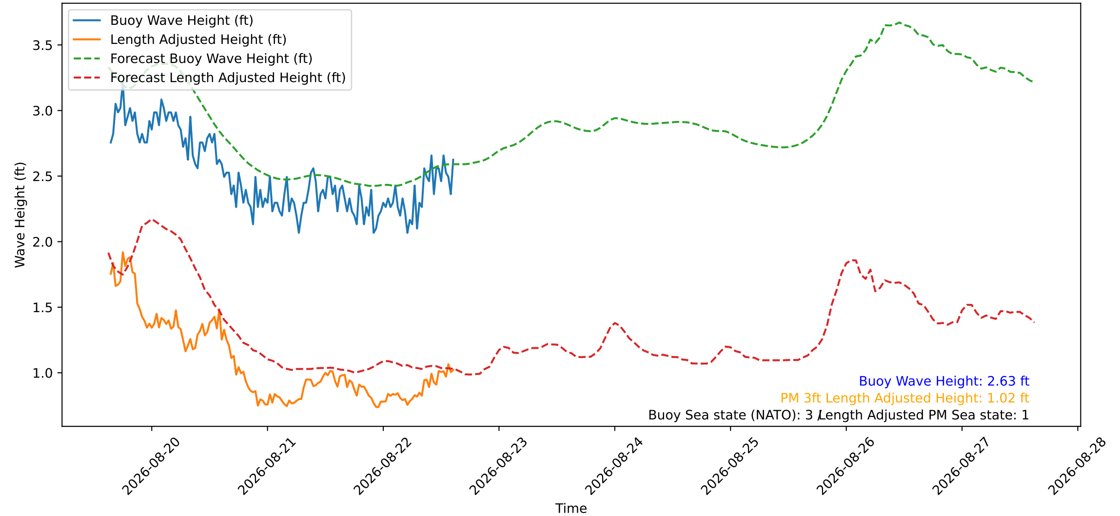
Wave Heights over Time for Red Beach at 2026-08-22 15:20:50
