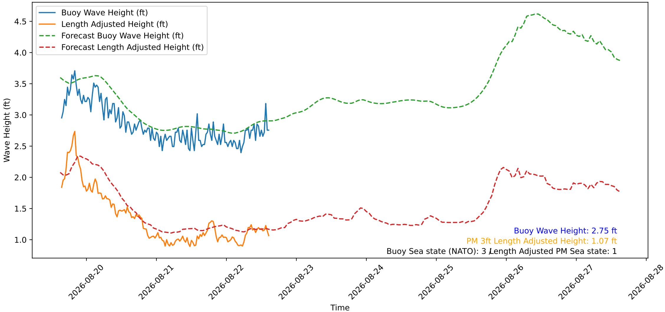
Wave Heights over Time for Green Beach at 2026-08-22 15:21:14
