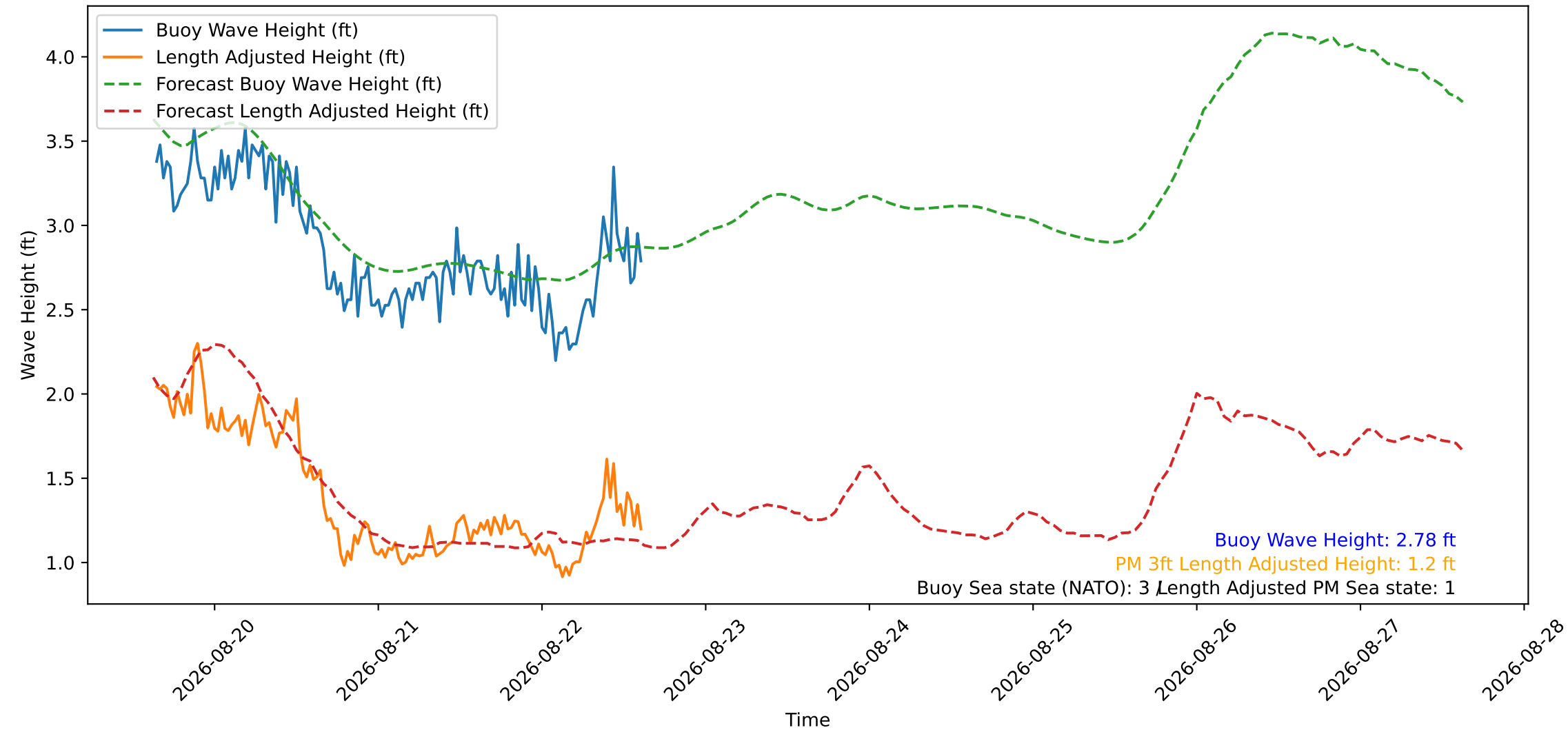
Wave Heights over Time for Oceanside Harbor at 2026-08-22 15:20:29
