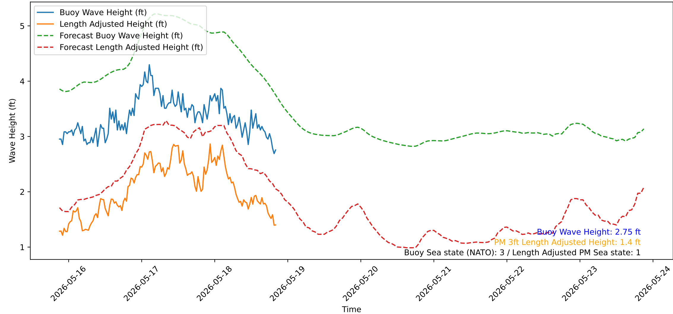
Wave Heights over Time for Oceanside Harbor at 2026-05-18 20:50:32
