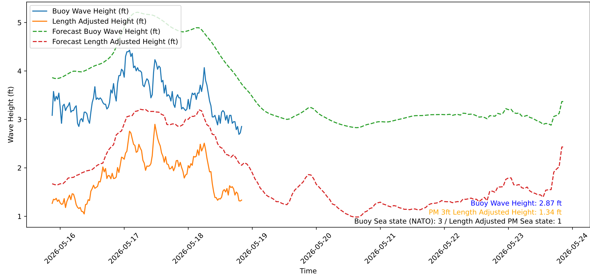
Wave Heights over Time for Green Beach at 2026-05-18 20:51:16
