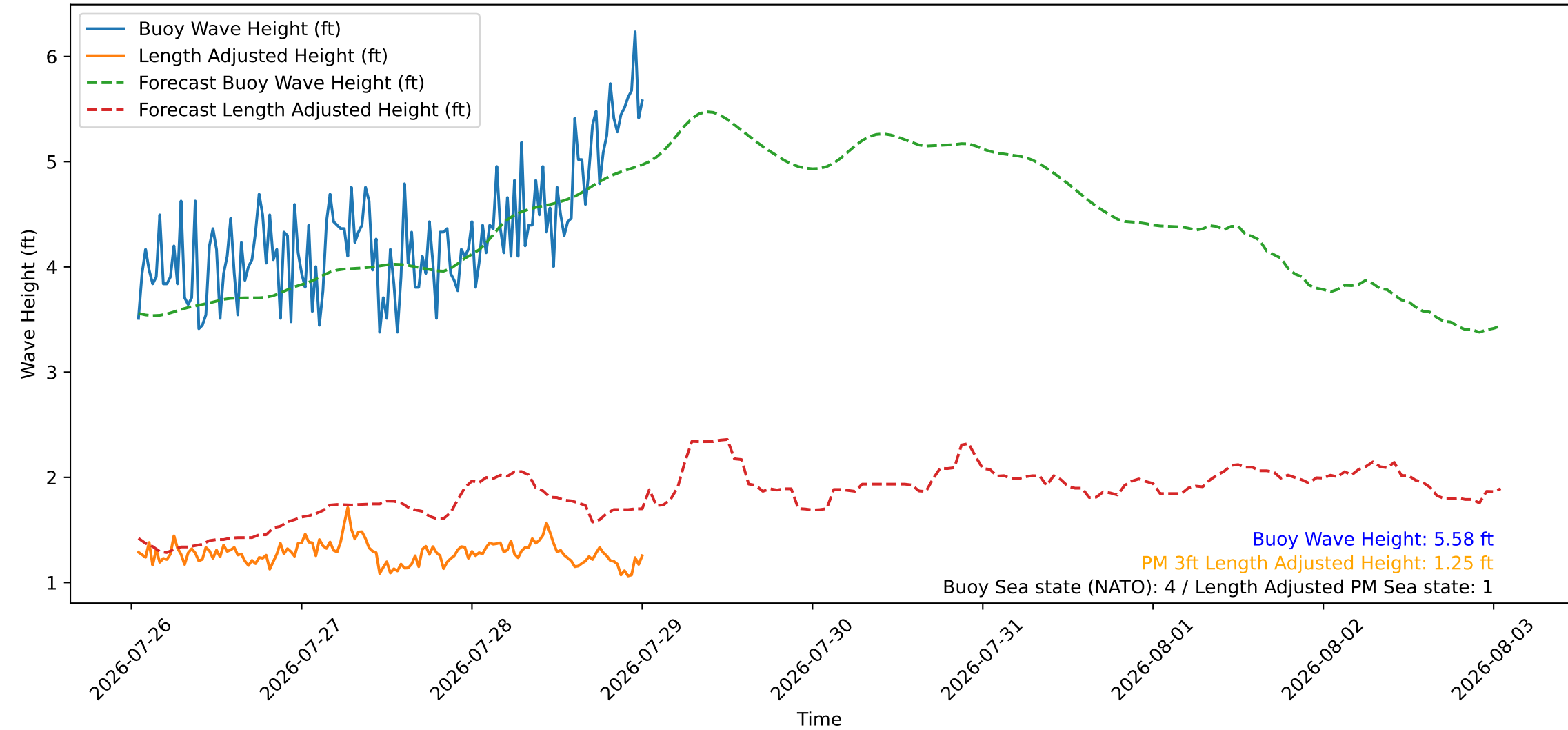
Wave Heights over Time for Green Beach at 2026-07-29 00:51:10
