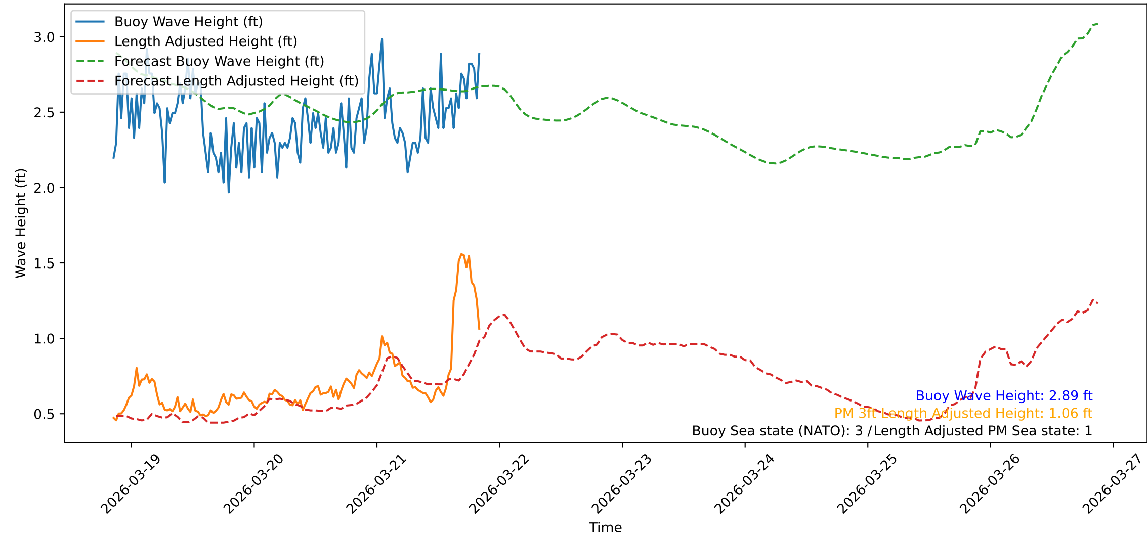
Wave Heights over Time for Oceanside Harbor at 2026-03-21 20:40:32
