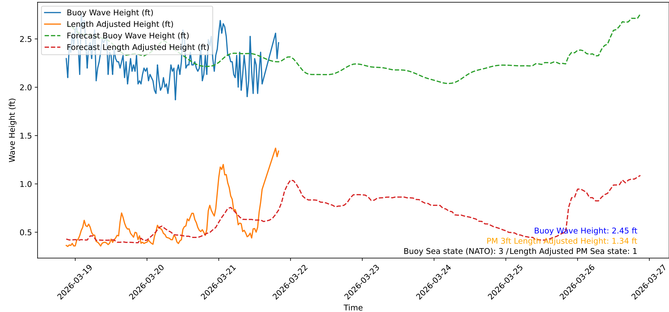
Wave Heights over Time for Red Beach at 2026-03-21 20:40:47
