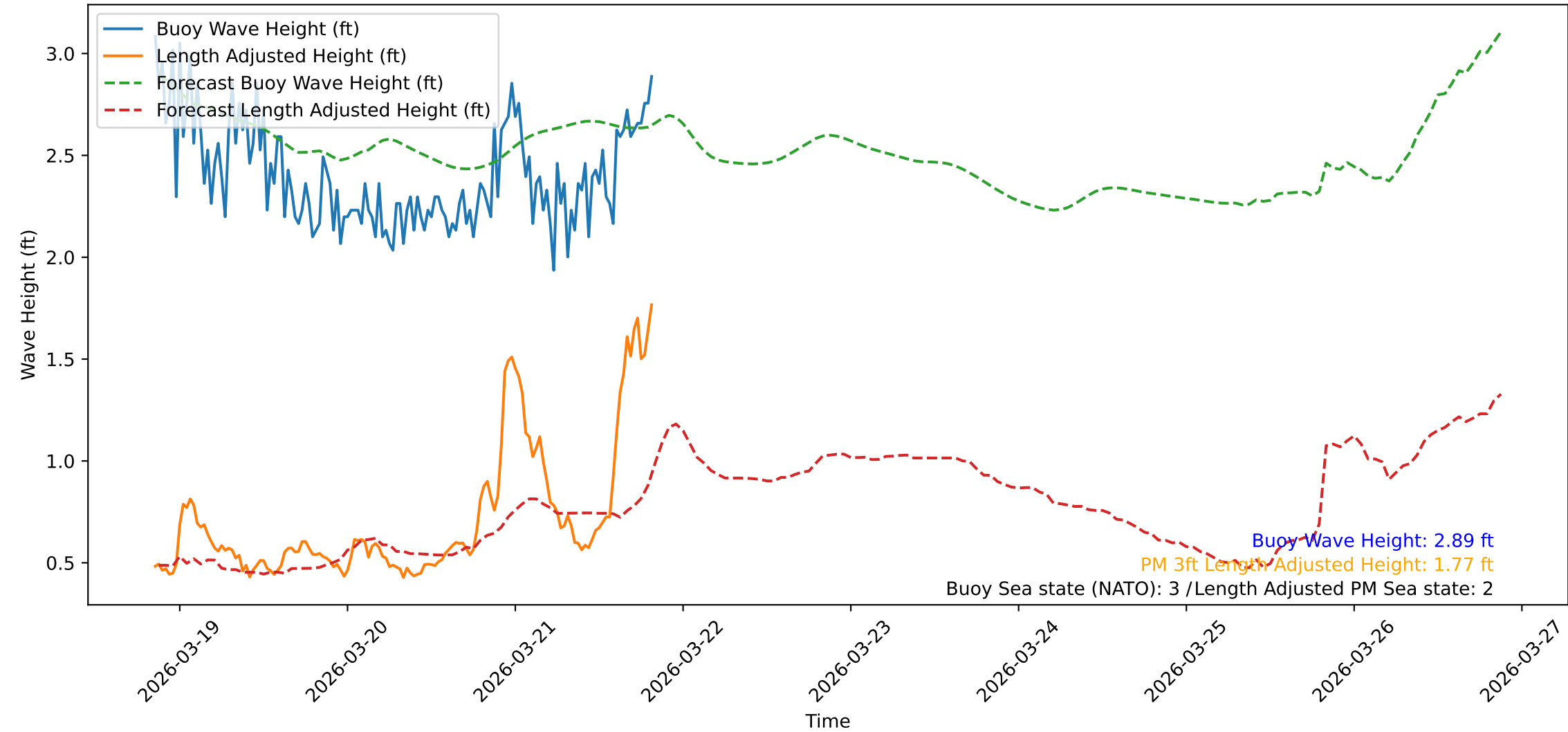
Wave Heights over Time for Green Beach at 2026-03-21 20:41:10
