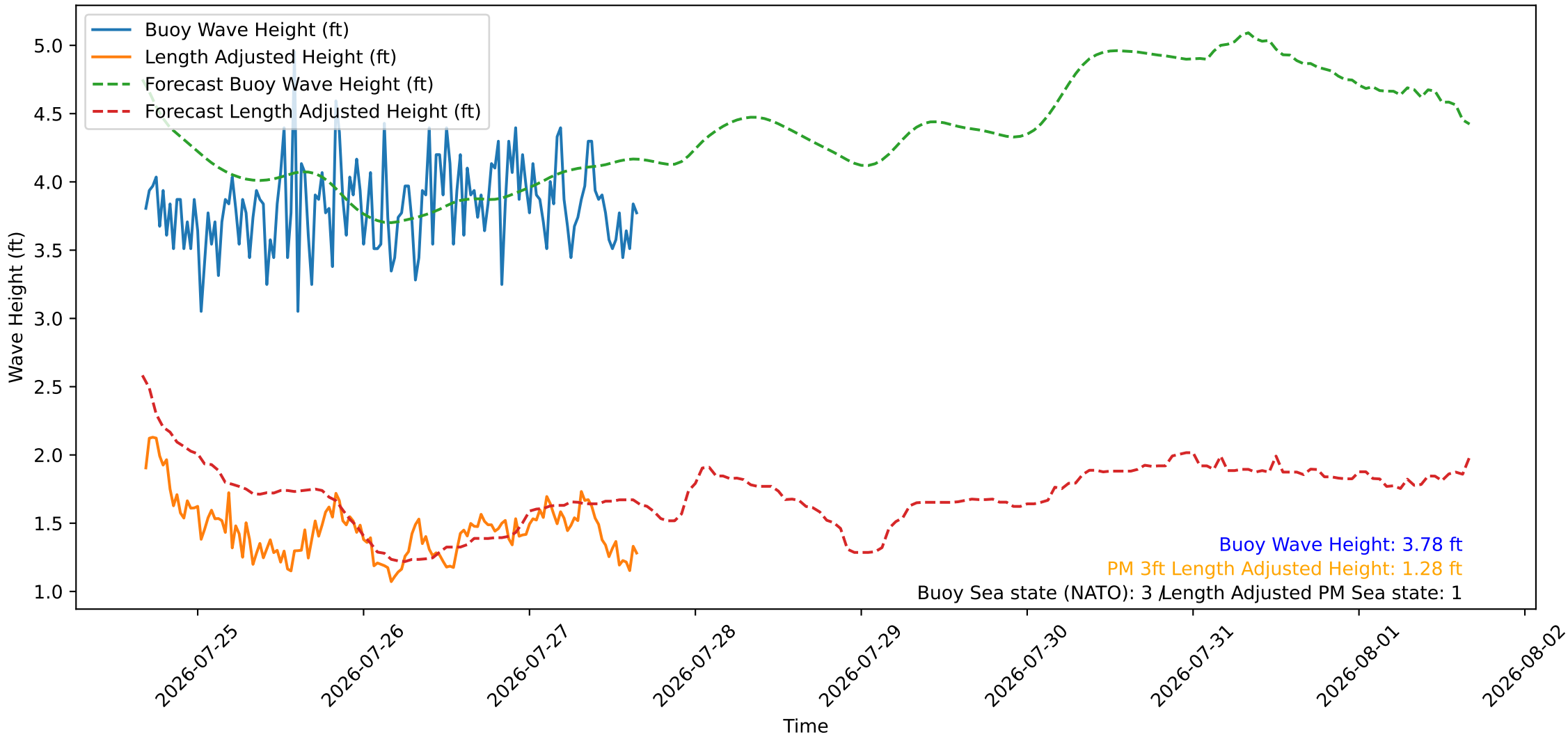
Wave Heights over Time for Oceanside Harbor at 2026-07-27 16:20:26
