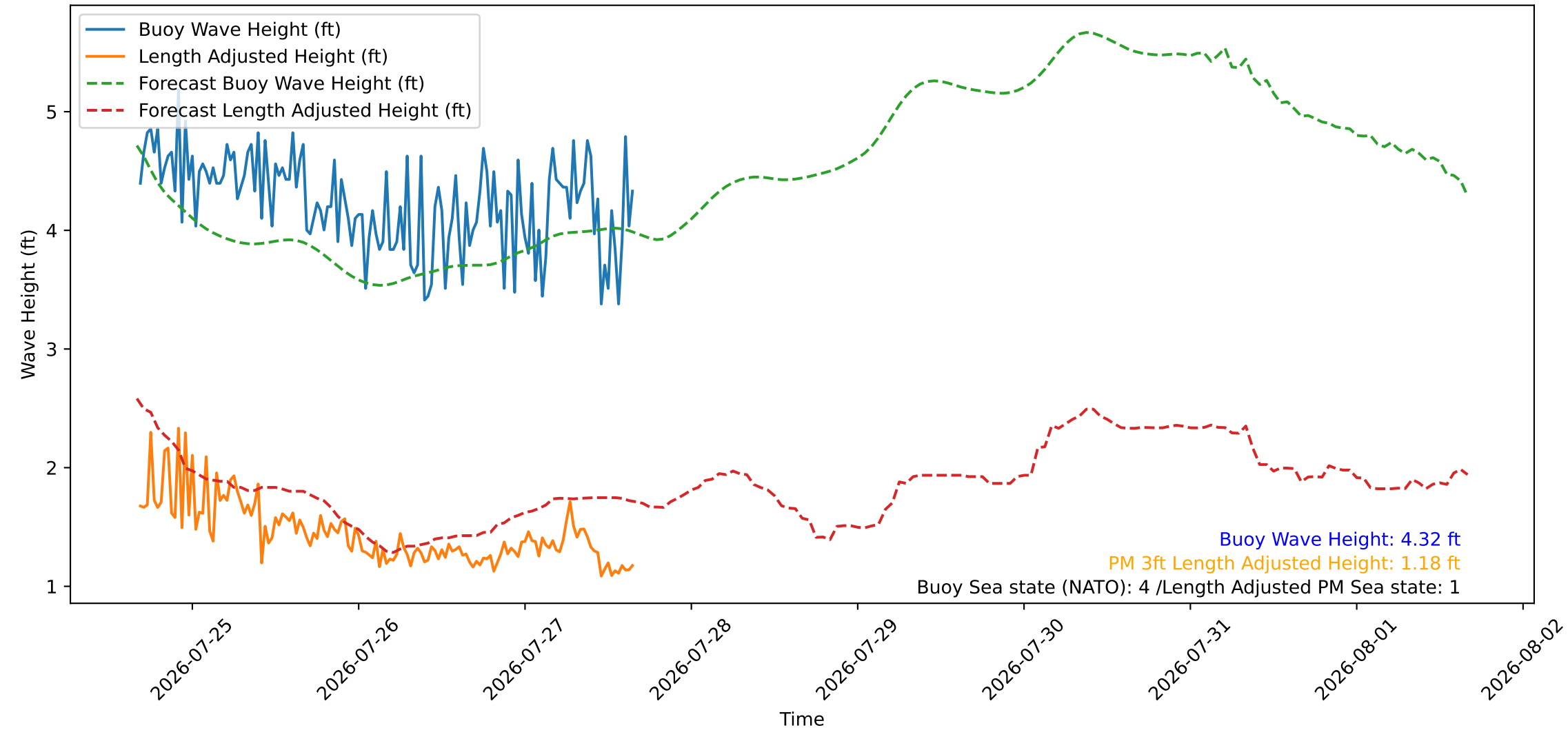
Wave Heights over Time for Green Beach at 2026-07-27 16:21:10
