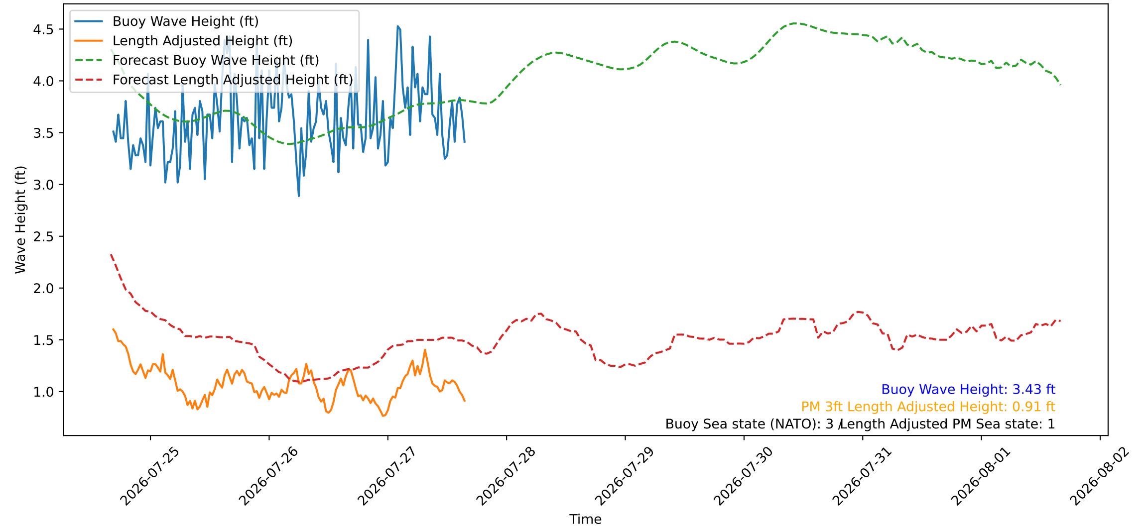
Wave Heights over Time for Red Beach at 2026-07-27 16:20:47
