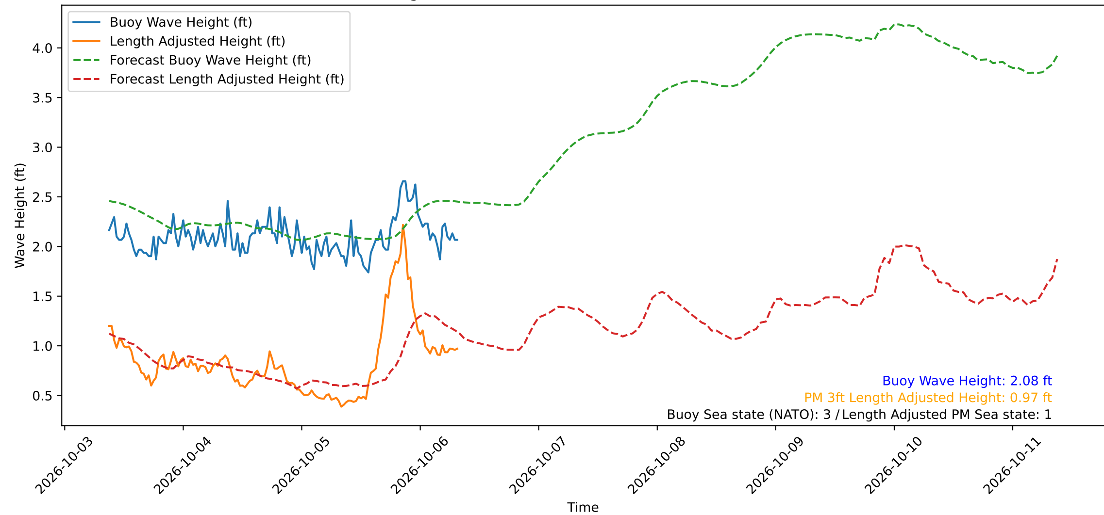
Wave Heights over Time for Red Beach at 2026-10-06 08:30:49
