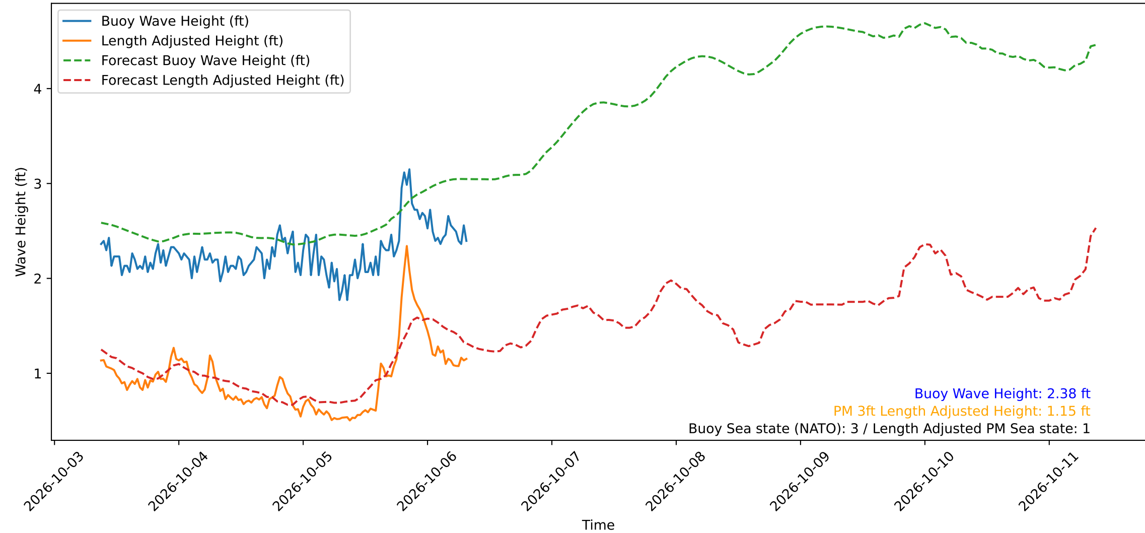
Wave Heights over Time for Green Beach at 2026-10-06 08:31:11
