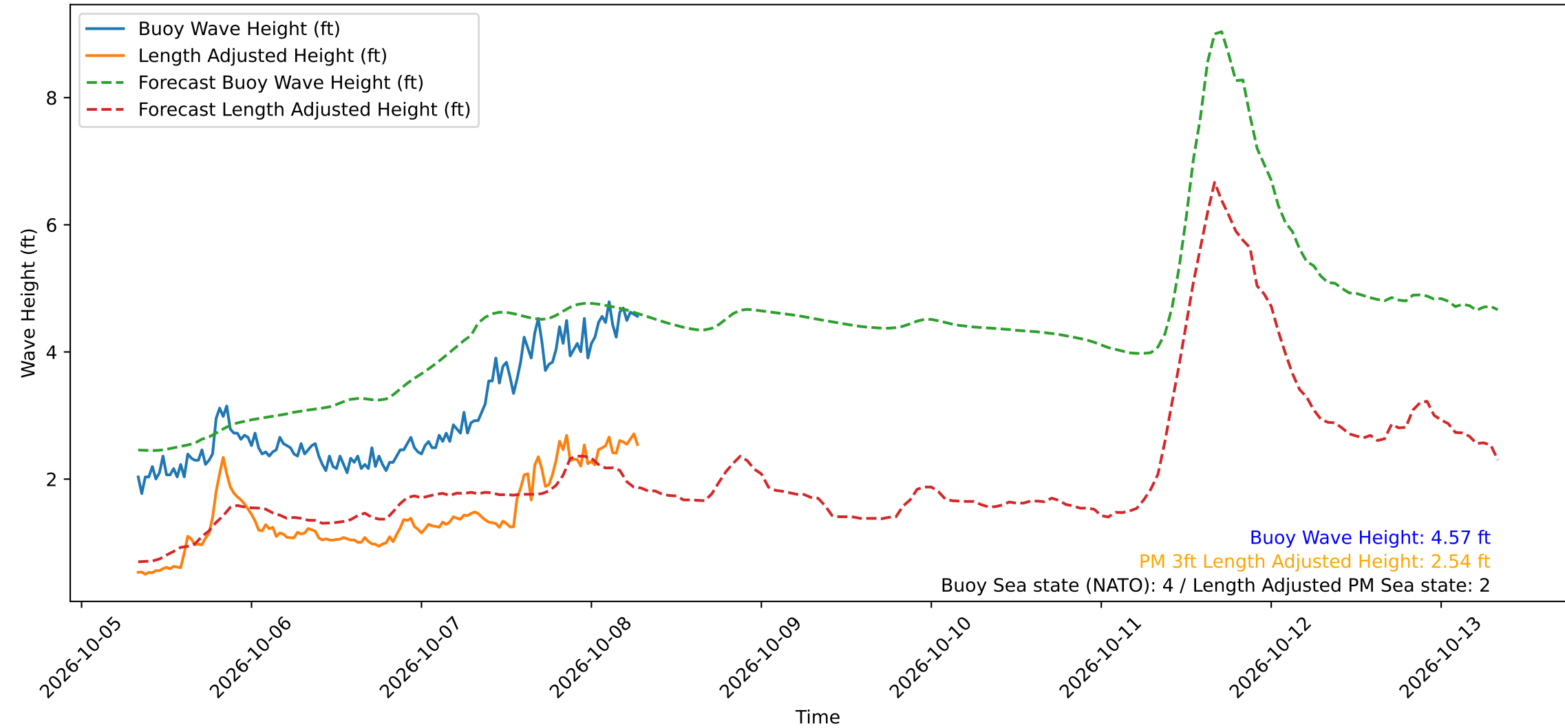
Wave Heights over Time for Green Beach at 2026-10-08 07:31:11
