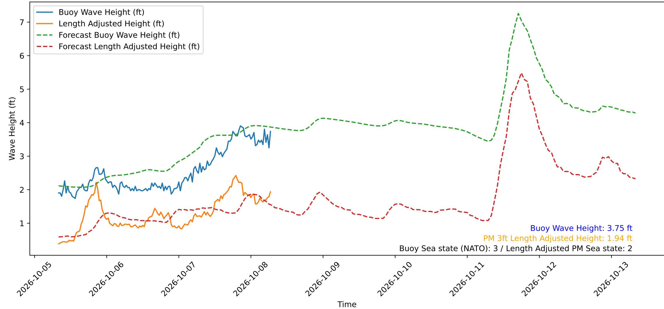
Wave Heights over Time for Red Beach at 2026-10-08 07:30:49
