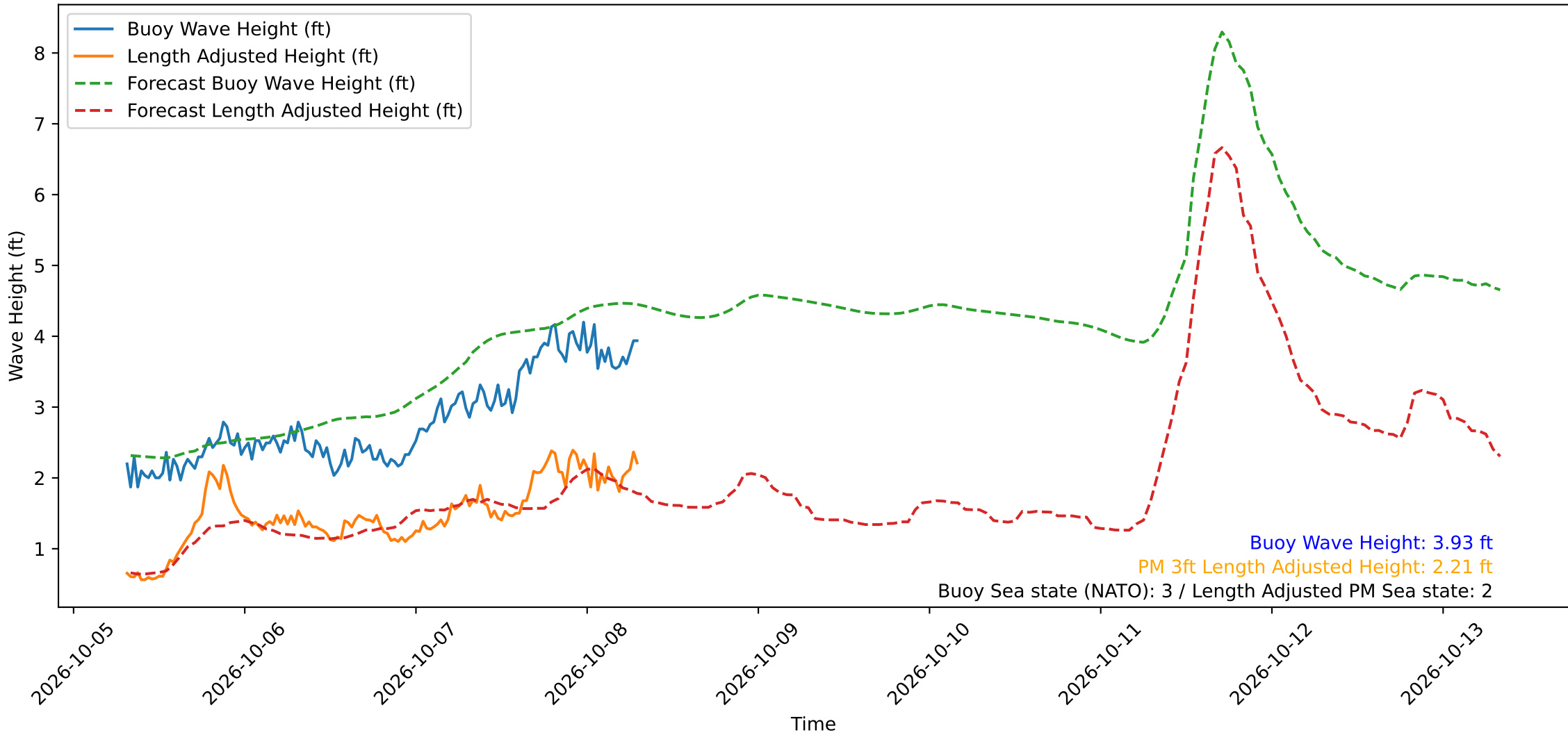
Wave Heights over Time for Oceanside Harbor at 2026-10-08 07:30:29
