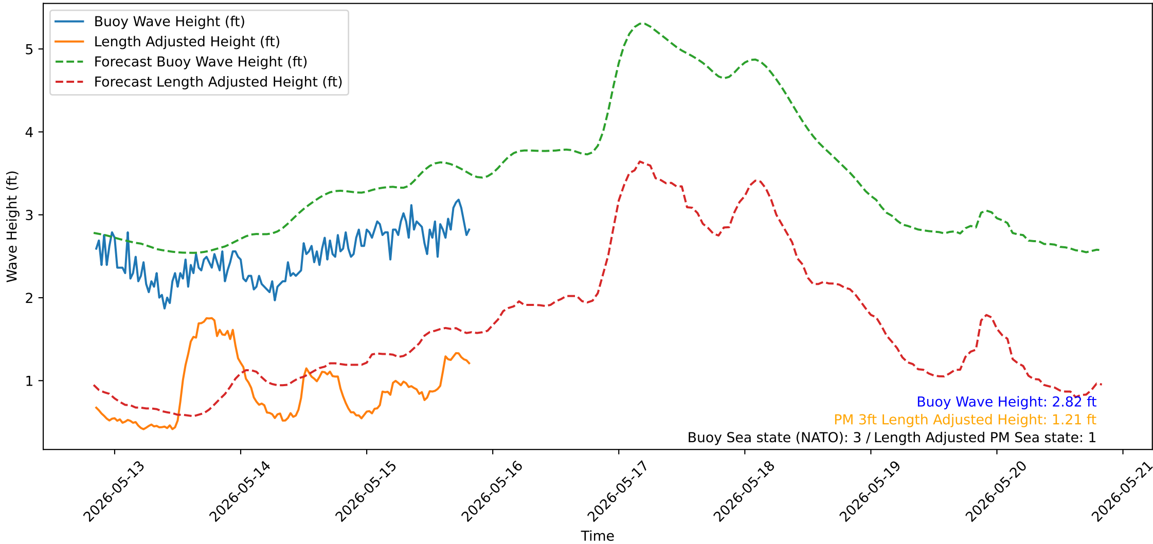
Wave Heights over Time for Red Beach at 2026-05-15 20:10:50
