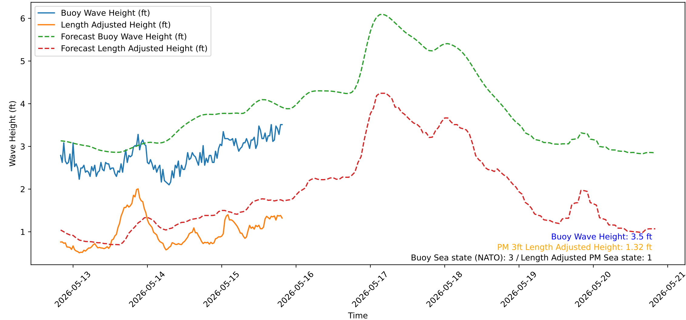
Wave Heights over Time for Green Beach at 2026-05-15 20:11:13
