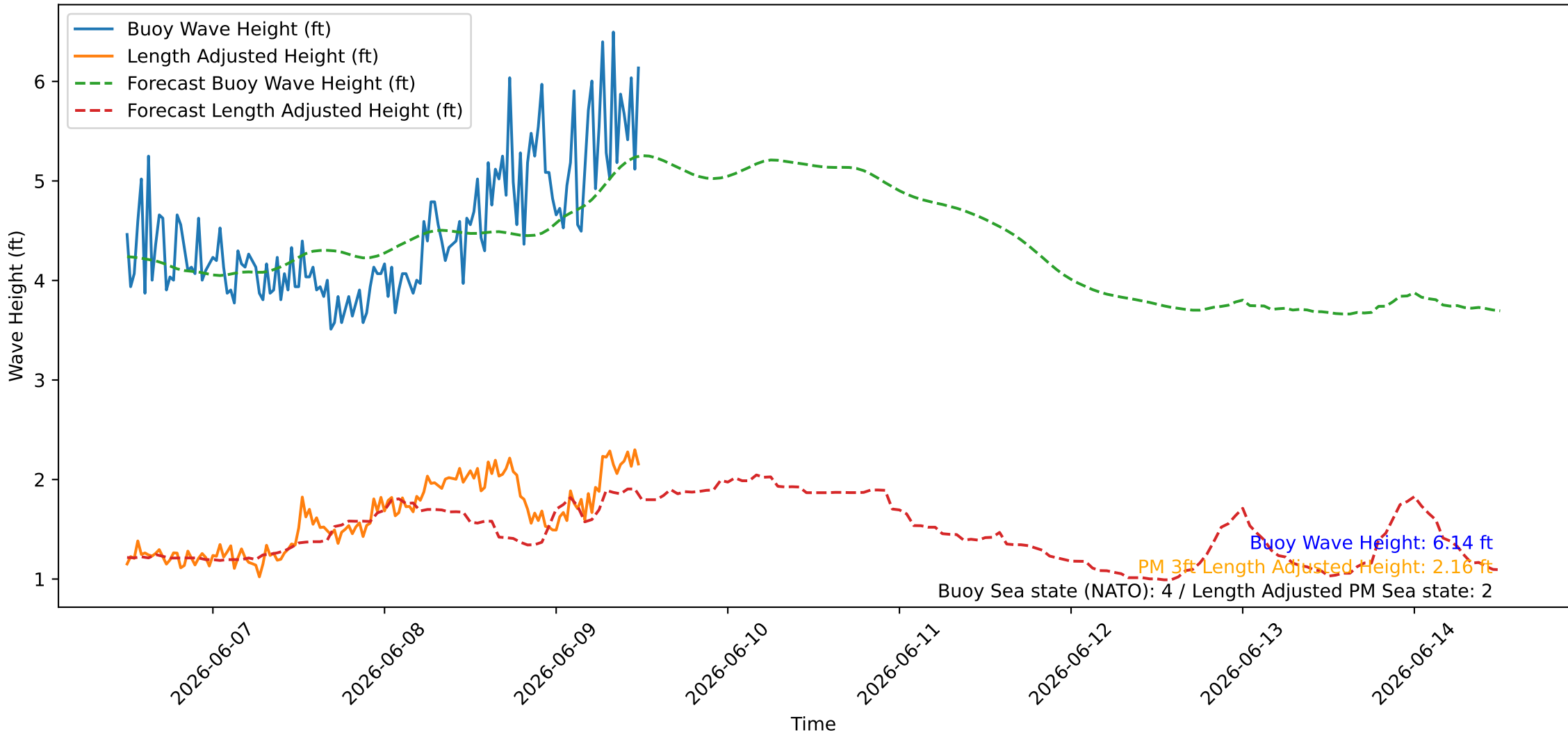
Wave Heights over Time for Oceanside Harbor at 2026-06-09 12:10:26
