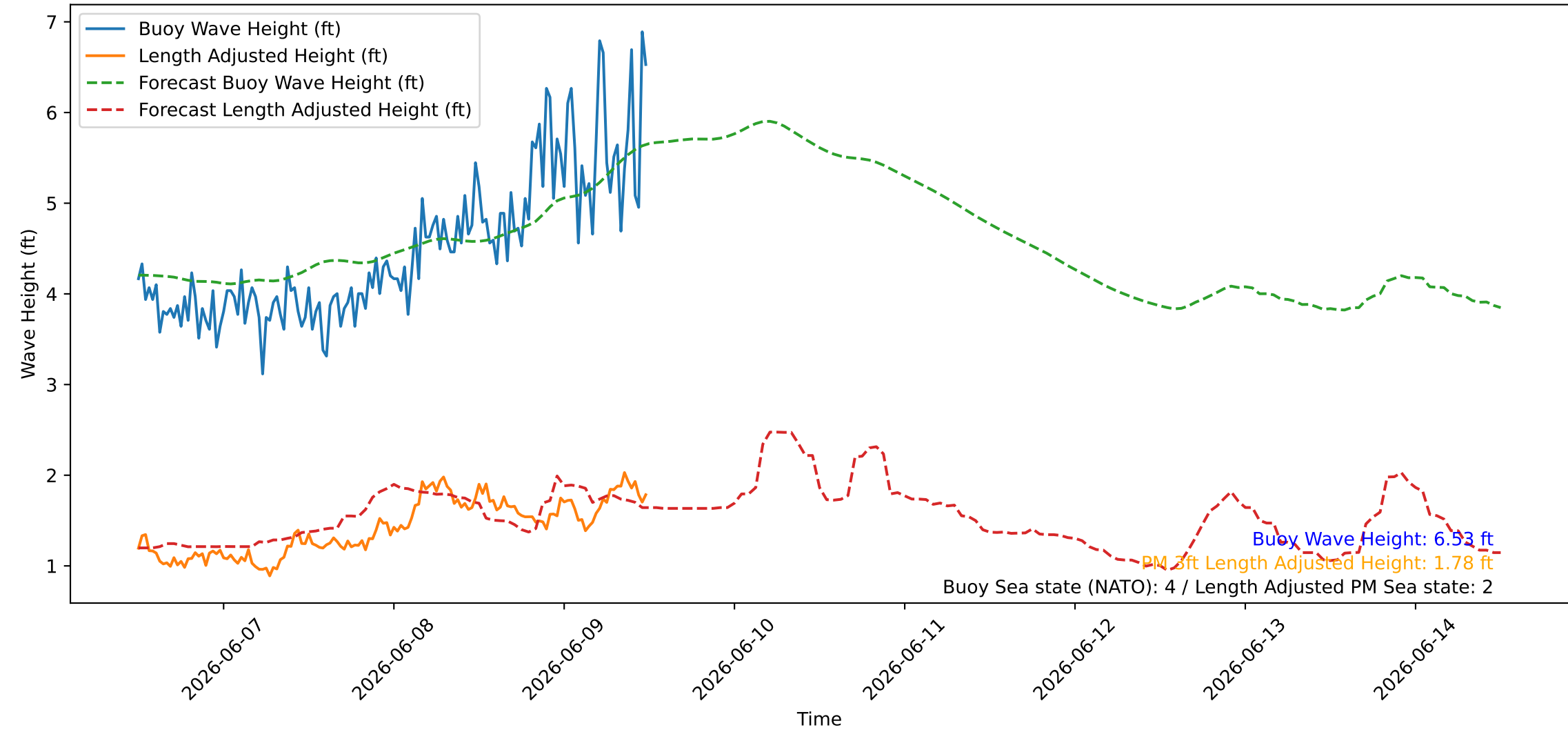
Wave Heights over Time for Green Beach at 2026-06-09 12:11:08
