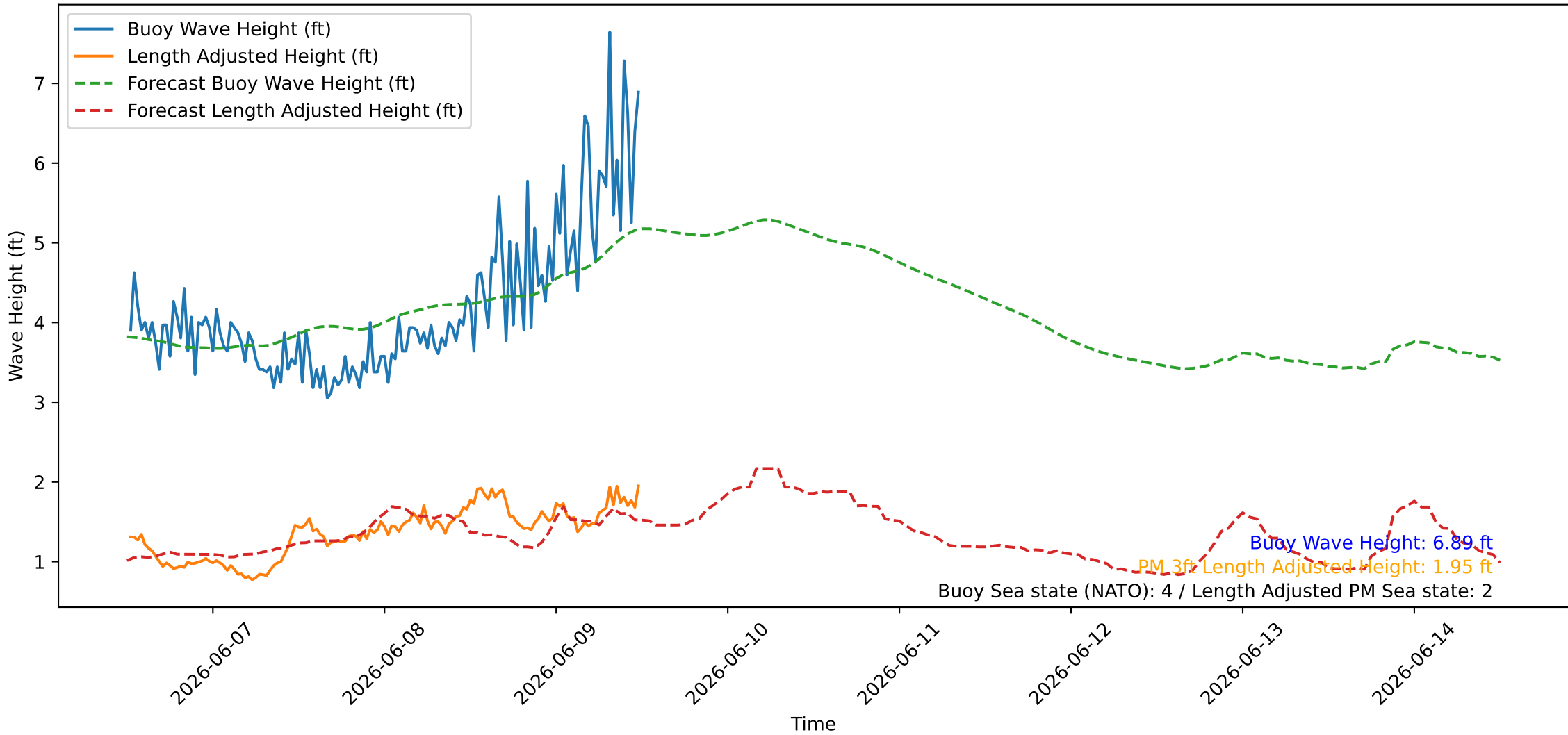
Wave Heights over Time for Red Beach at 2026-06-09 12:10:45
