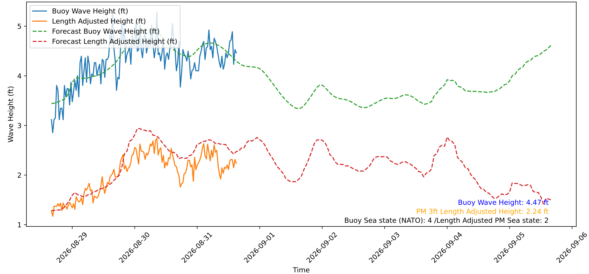
Wave Heights over Time for Oceanside Harbor at 2026-08-31 15:50:30
