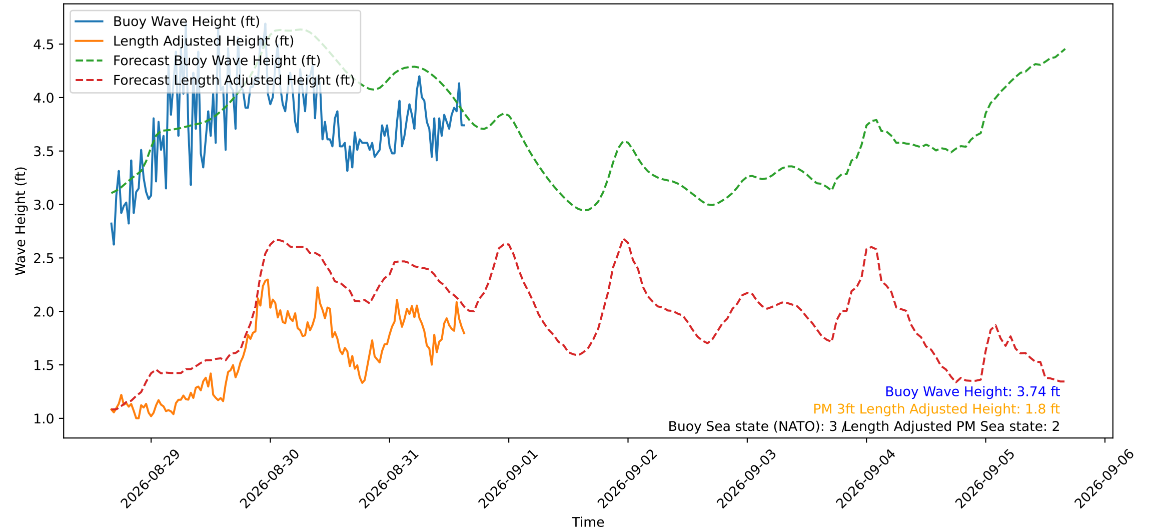
Wave Heights over Time for Red Beach at 2026-08-31 15:50:50
