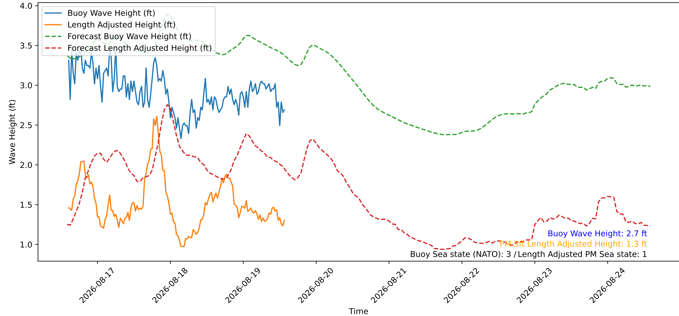
Wave Heights over Time for Red Beach at 2026-08-19 14:20:47
