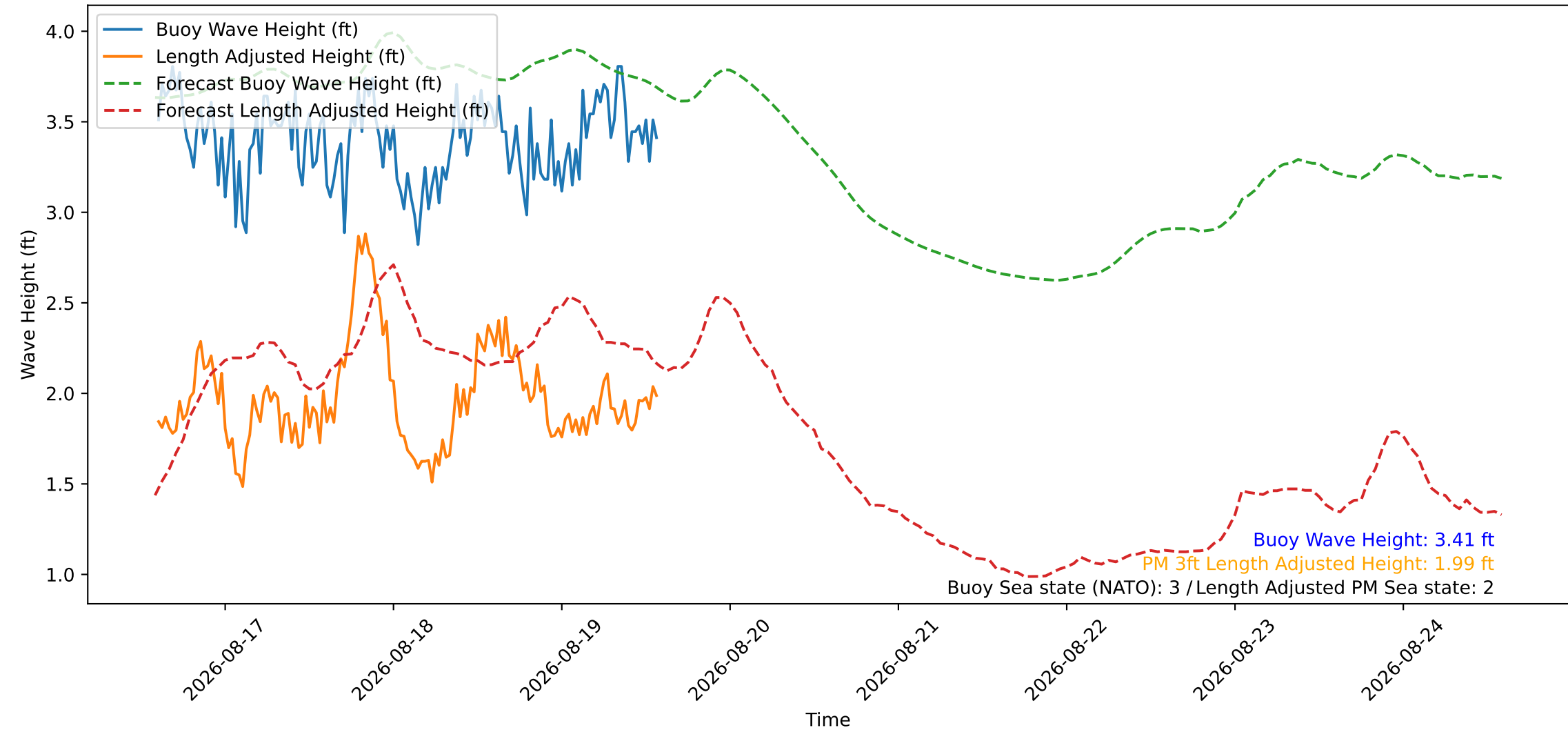
Wave Heights over Time for Oceanside Harbor at 2026-08-19 14:20:26
