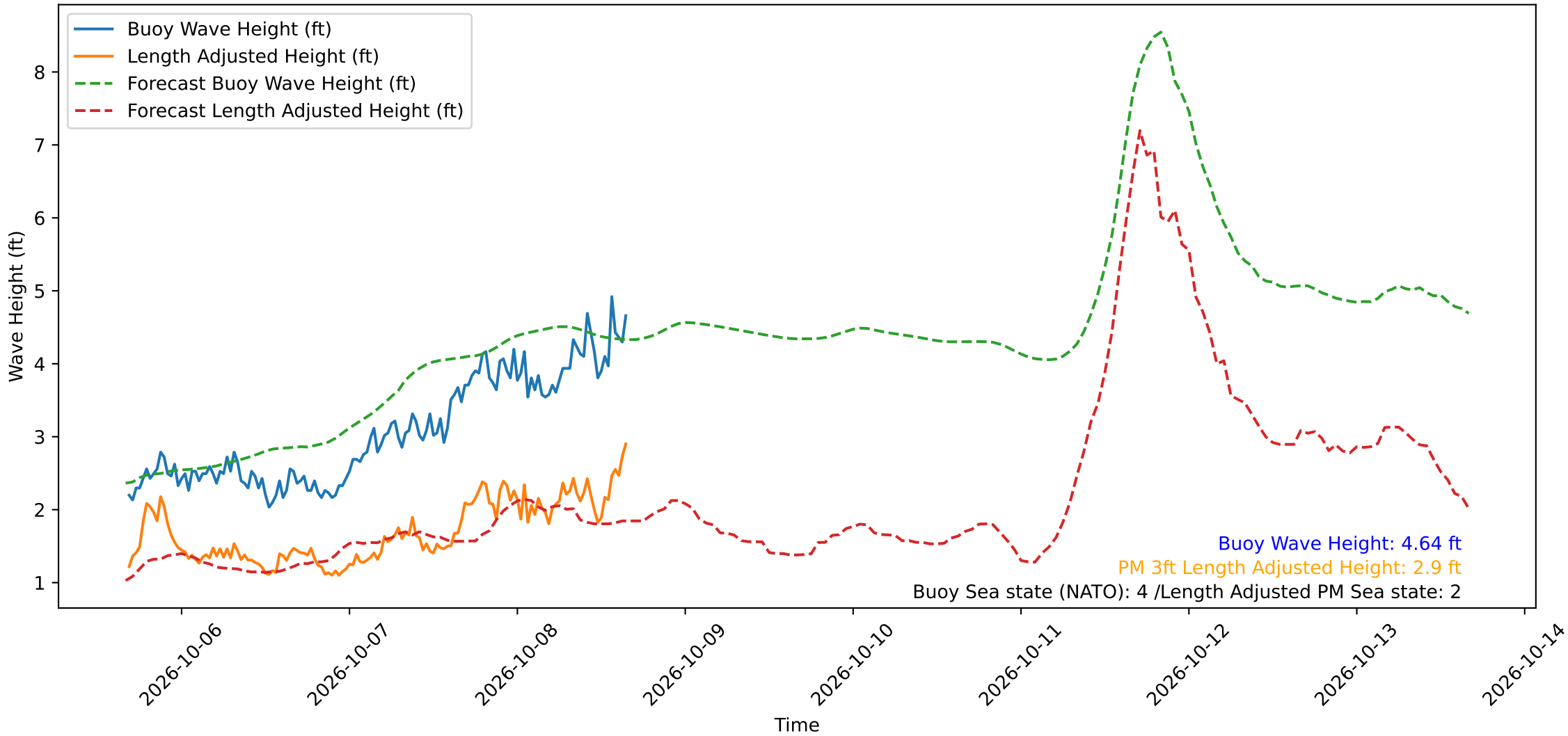
Wave Heights over Time for Oceanside Harbor at 2026-10-08 16:20:30
