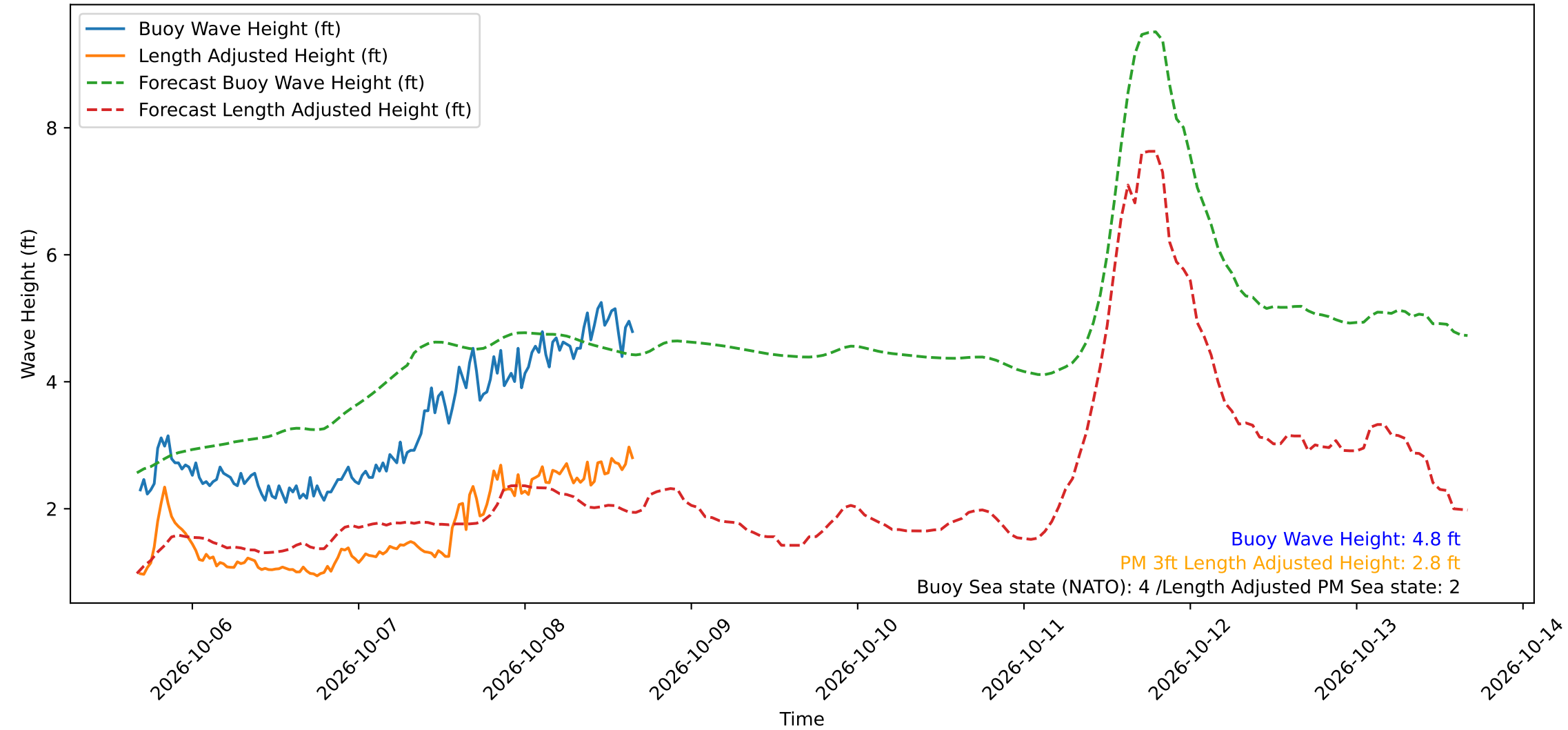
Wave Heights over Time for Green Beach at 2026-10-08 16:21:14
