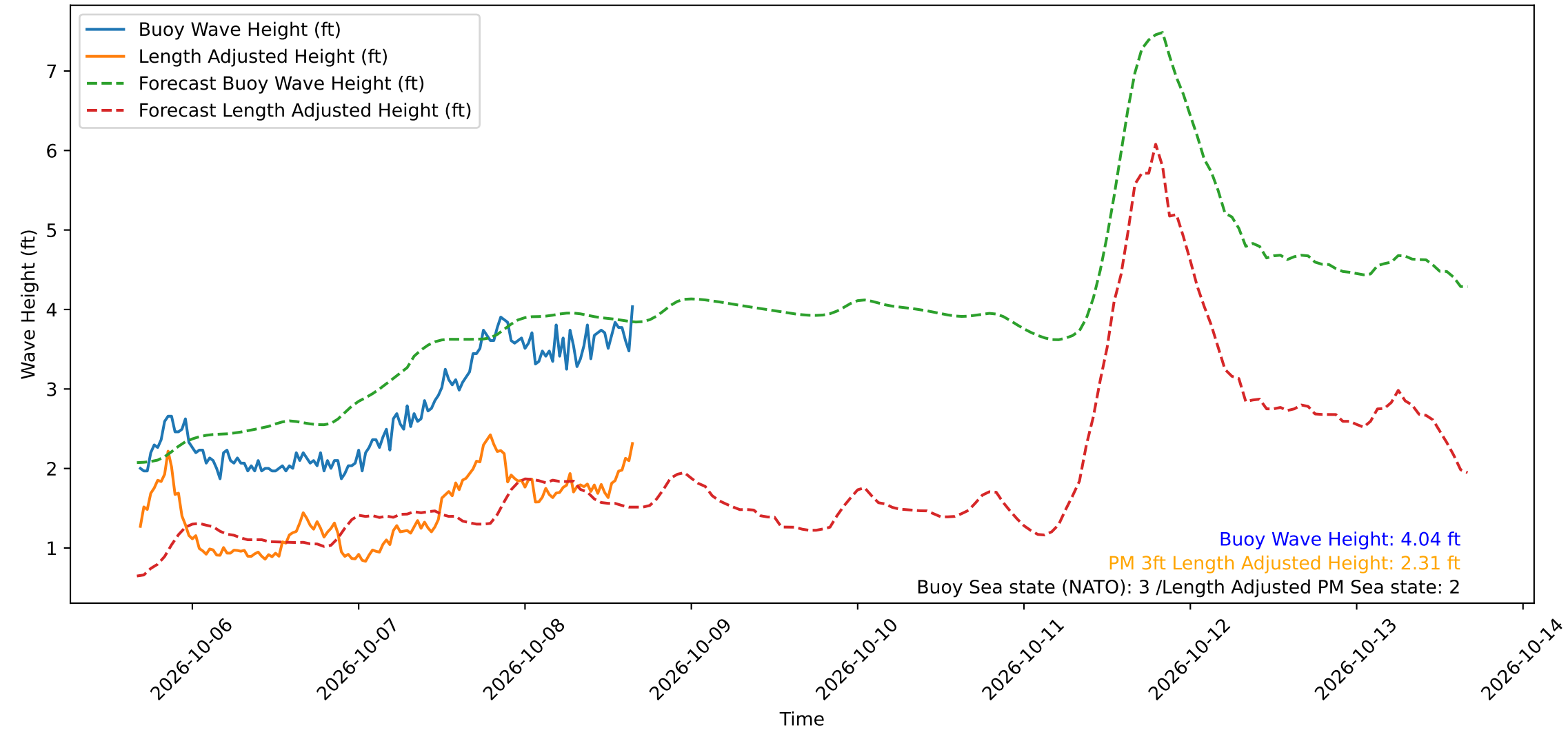
Wave Heights over Time for Red Beach at 2026-10-08 16:20:50
