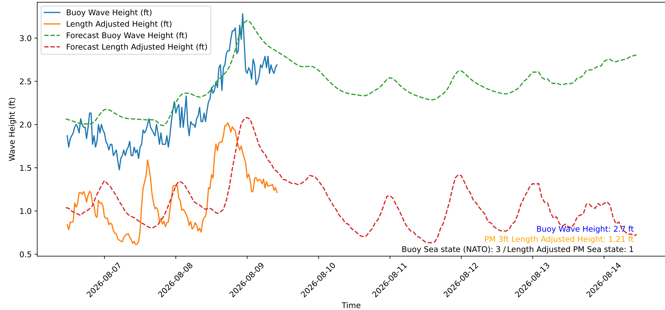
Wave Heights over Time for Red Beach at 2026-08-09 11:10:46
