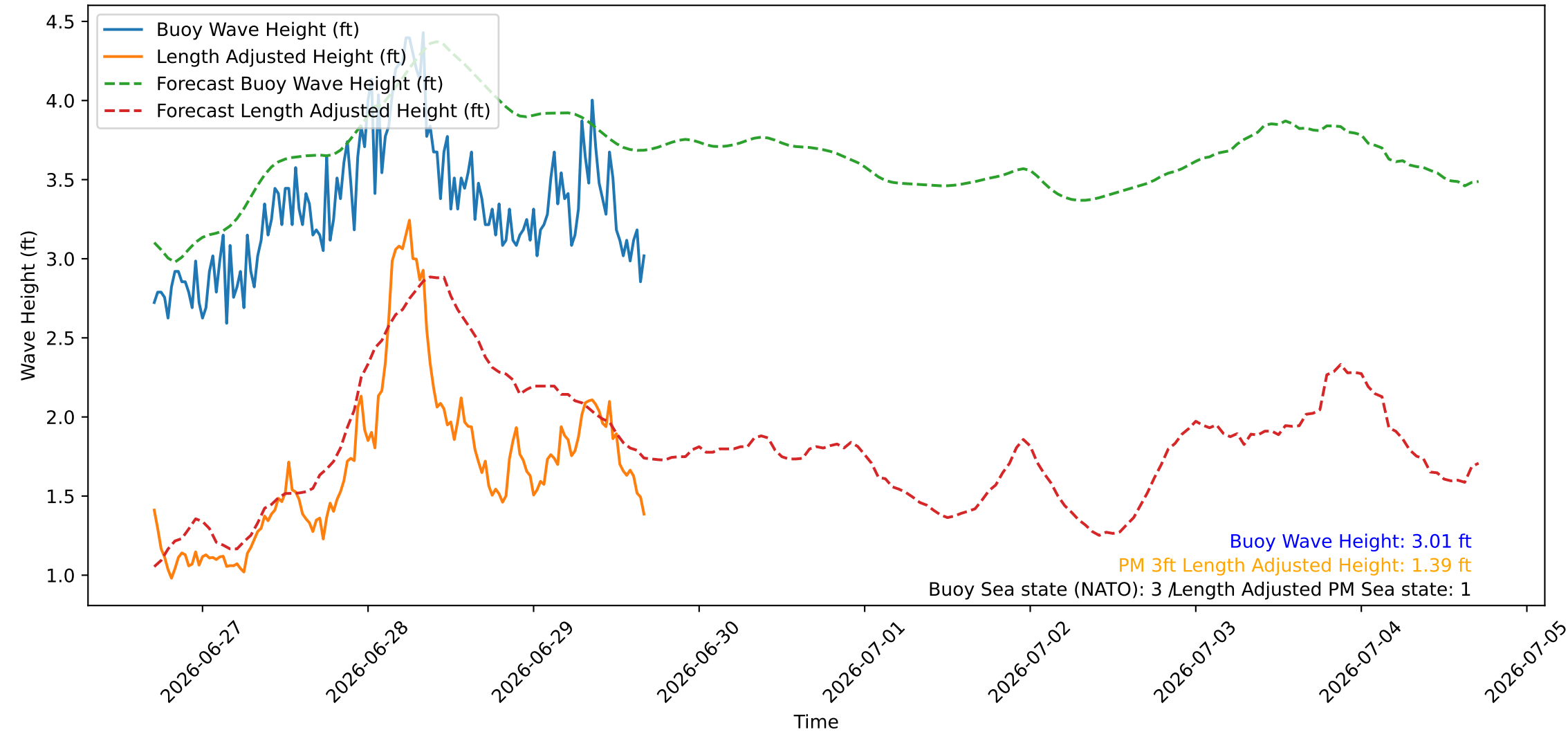
Wave Heights over Time for Oceanside Harbor at 2026-06-29 17:00:26
