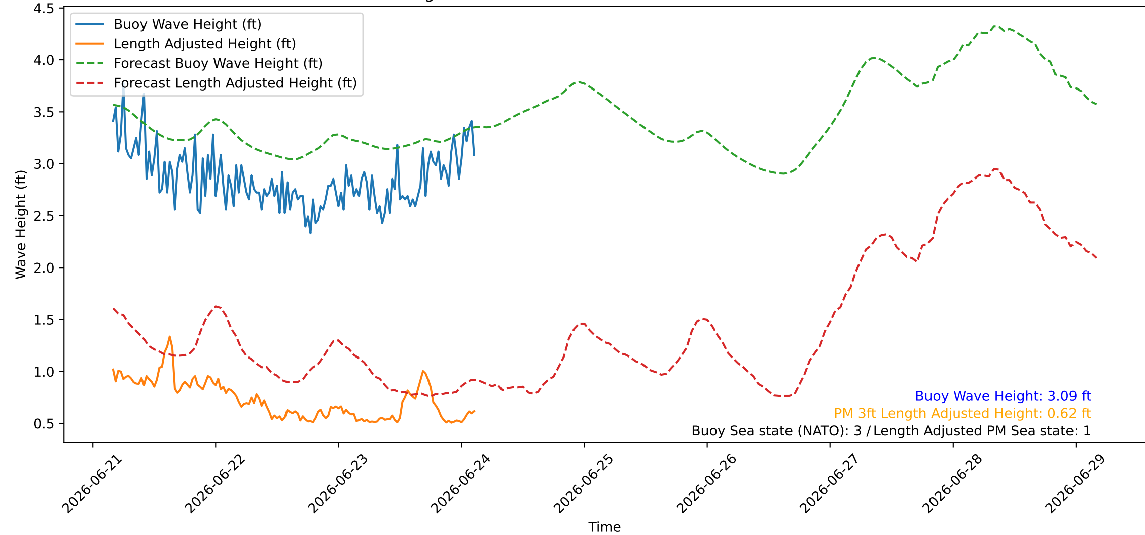
Wave Heights over Time for Red Beach at 2026-06-24 03:30:45
