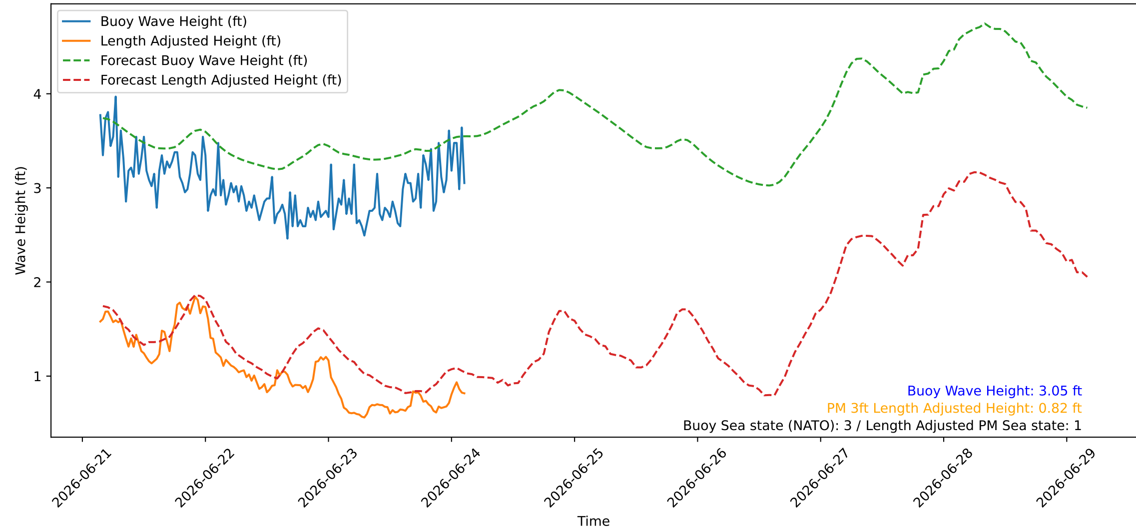
Wave Heights over Time for Green Beach at 2026-06-24 03:31:08
