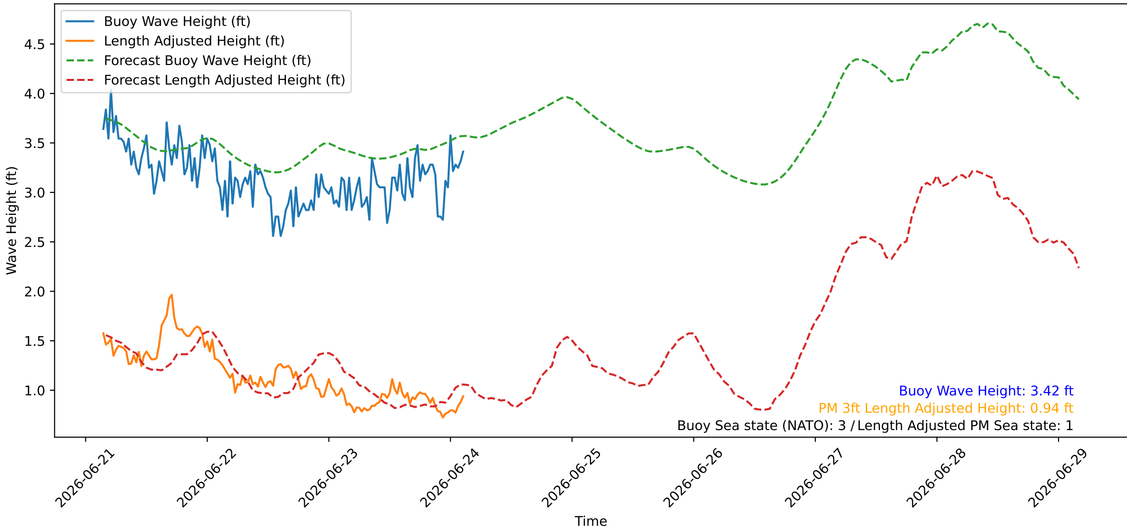
Wave Heights over Time for Oceanside Harbor at 2026-06-24 03:30:26
