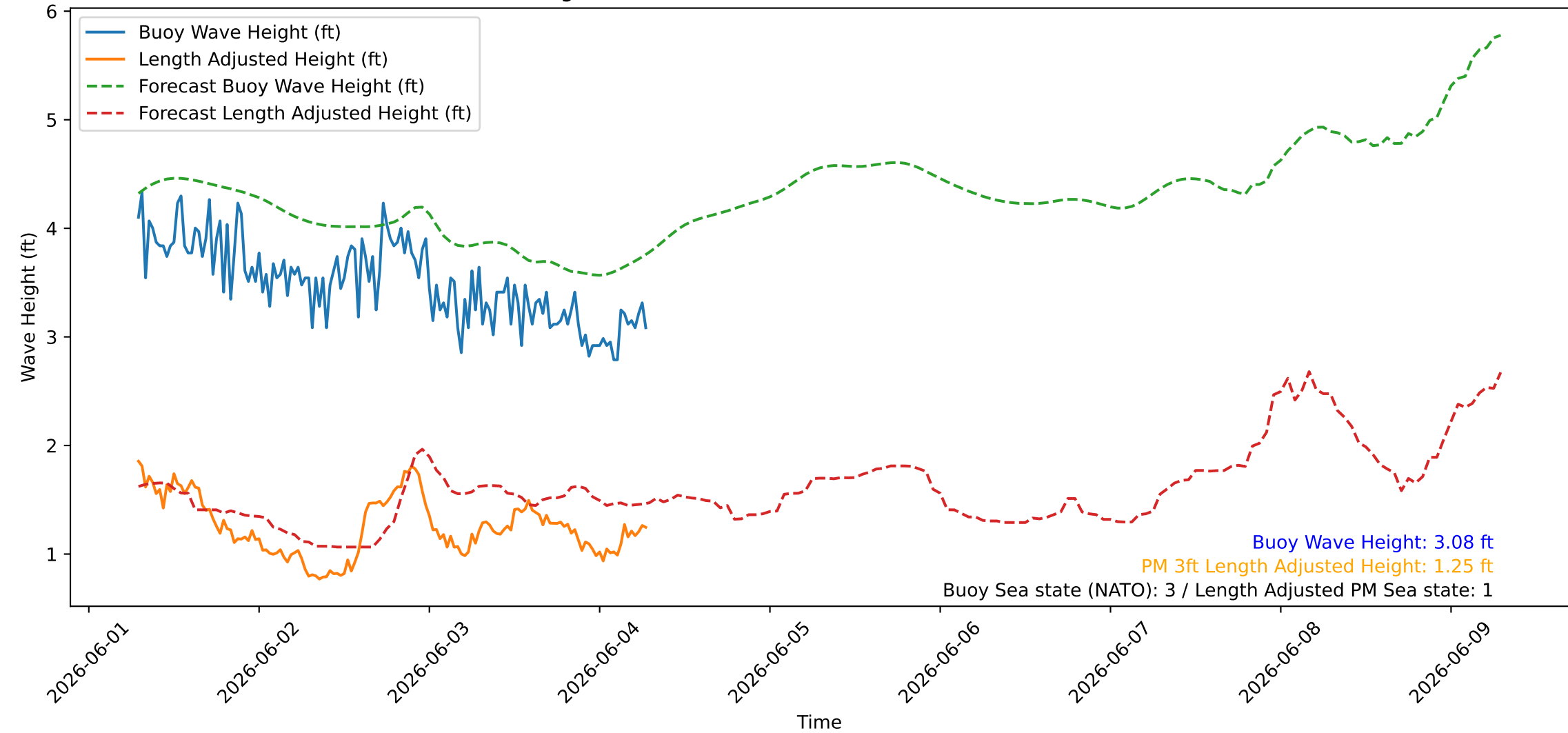
Wave Heights over Time for Green Beach at 2026-06-04 07:11:08
