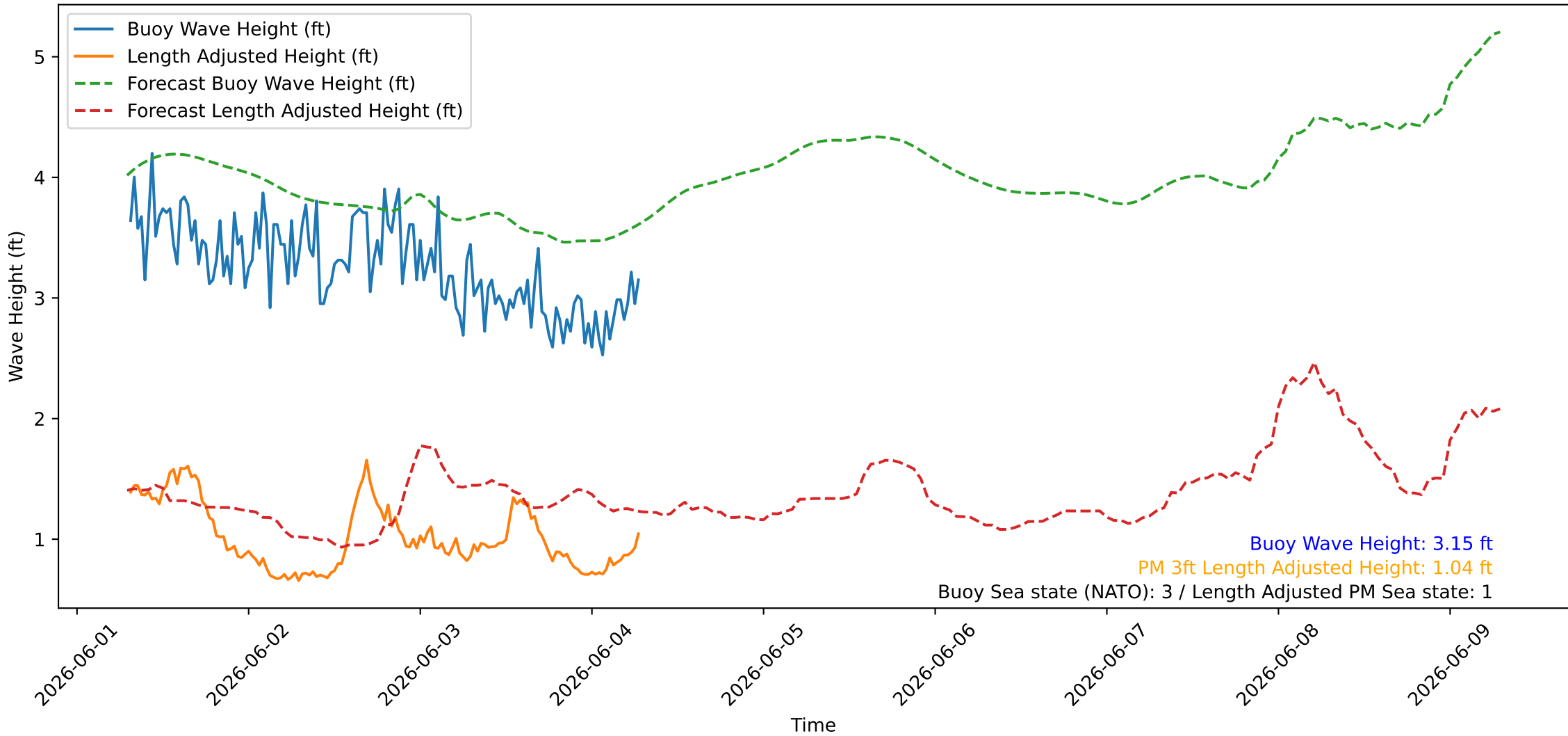
Wave Heights over Time for Red Beach at 2026-06-04 07:10:46
