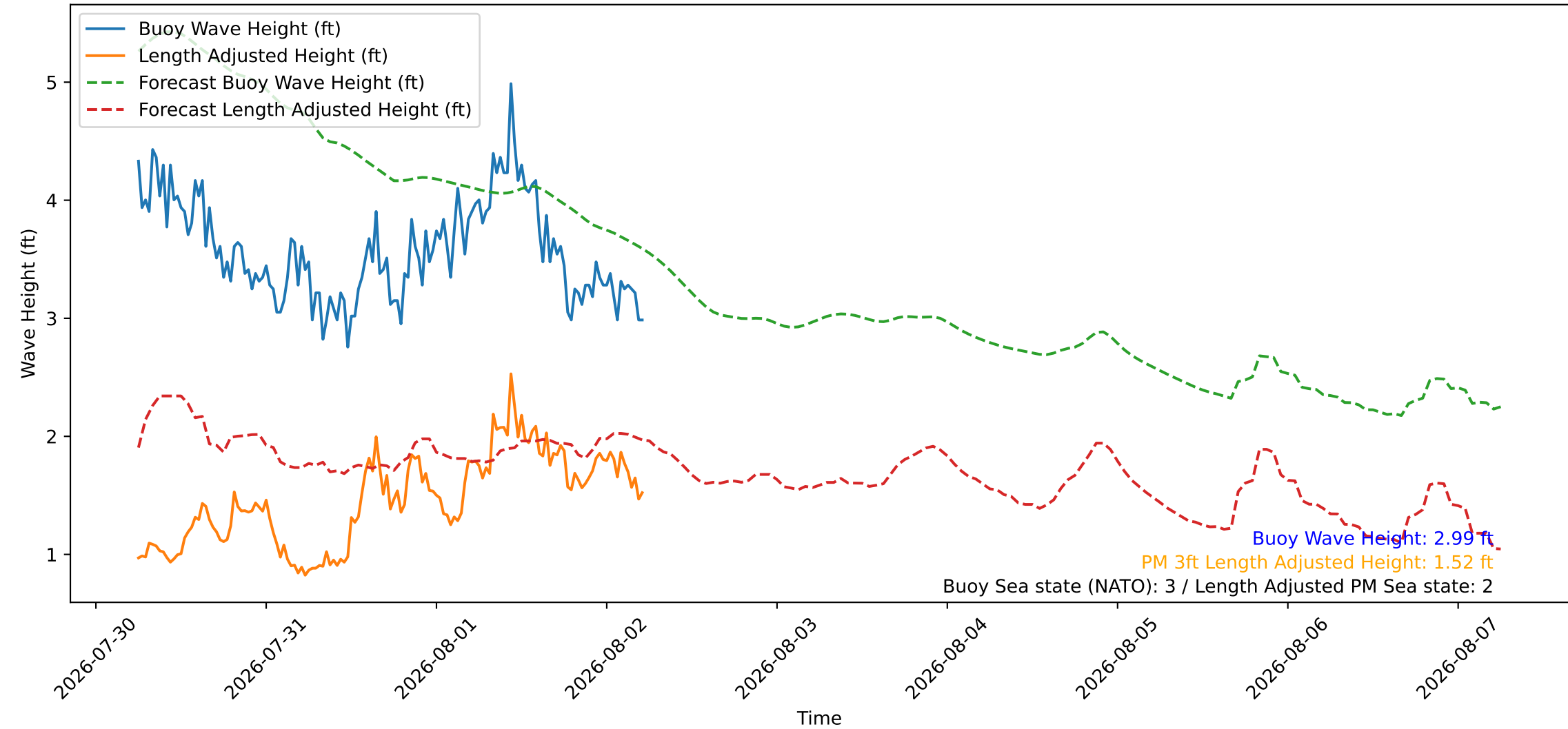
Wave Heights over Time for Green Beach at 2026-08-02 06:01:08
