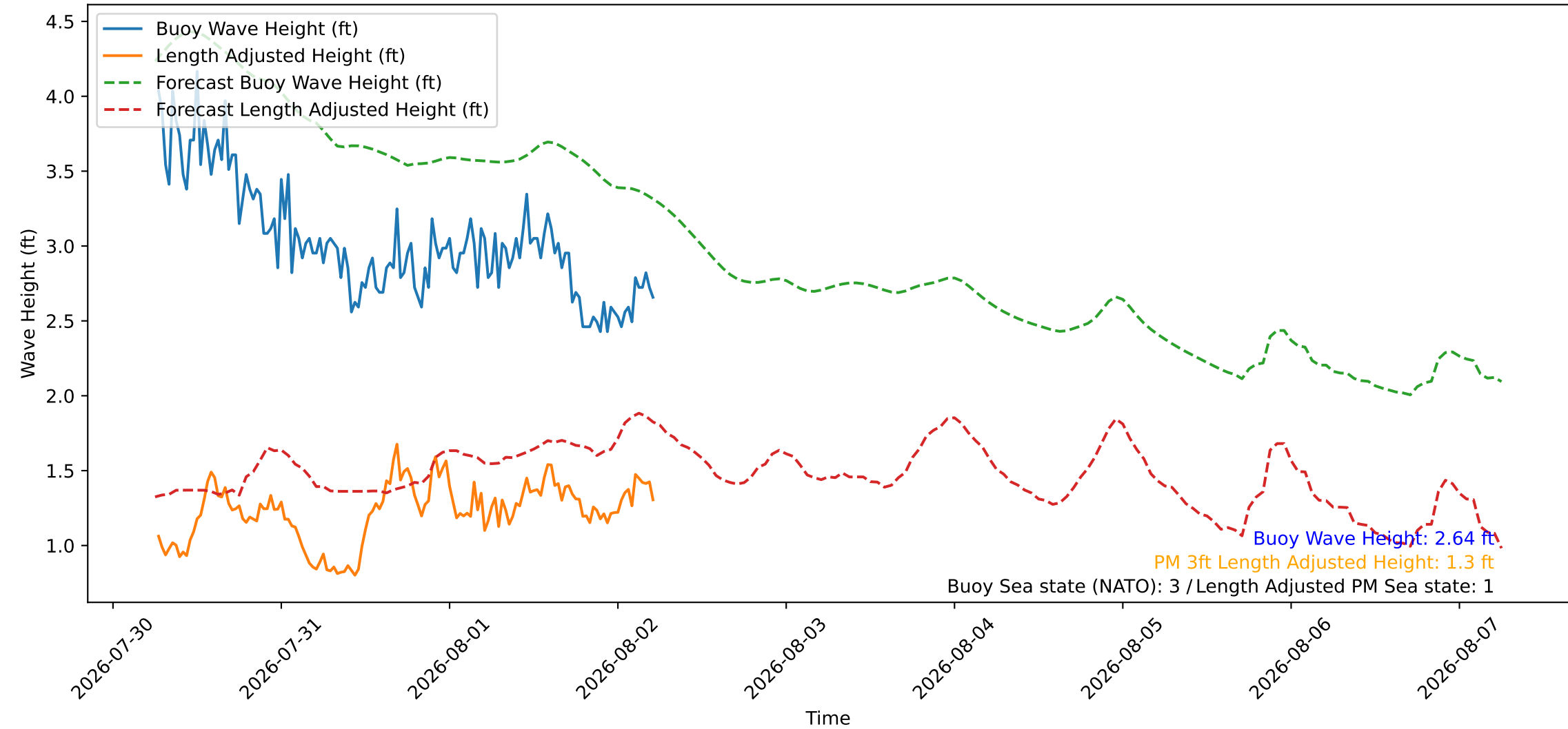
Wave Heights over Time for Red Beach at 2026-08-02 06:00:46
