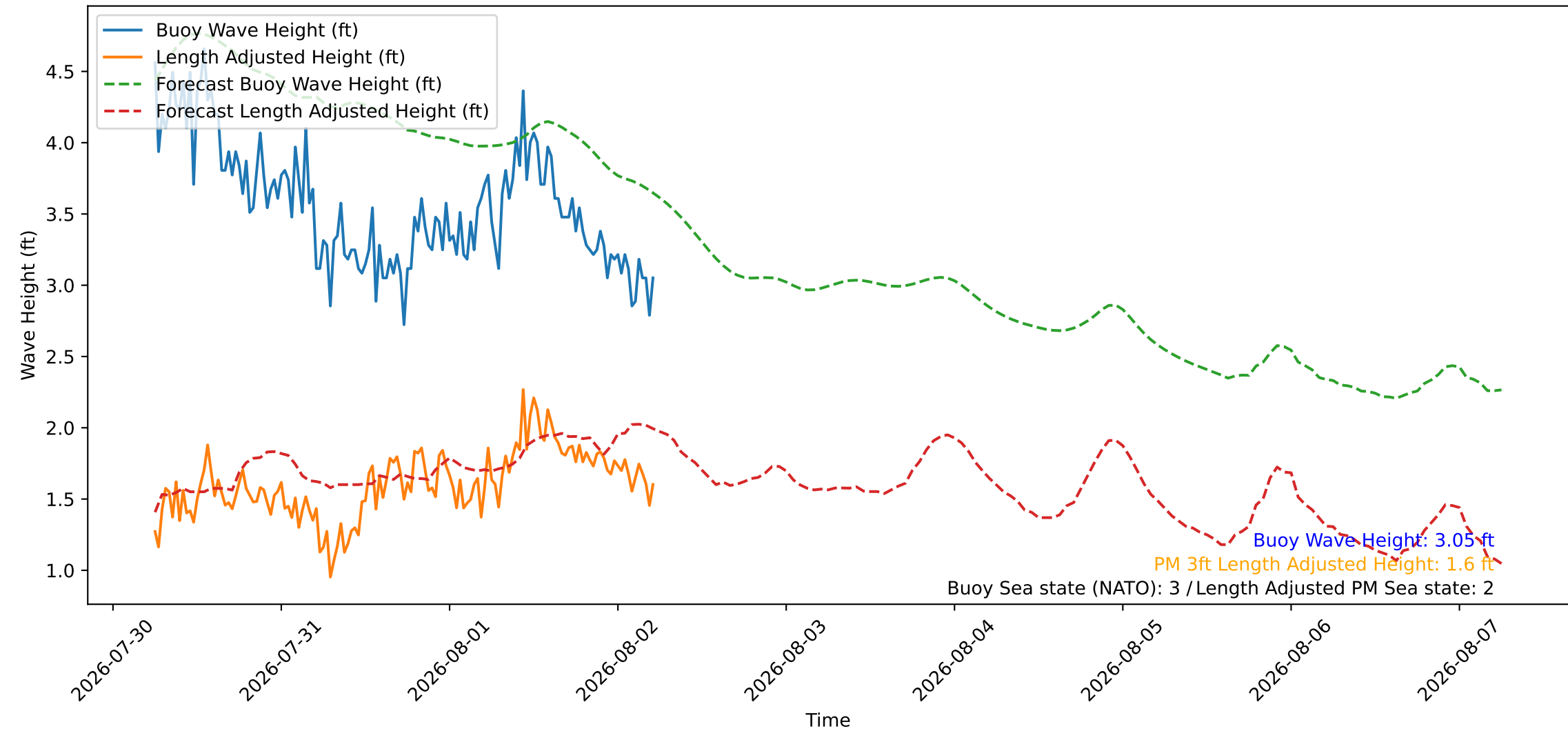
Wave Heights over Time for Oceanside Harbor at 2026-08-02 06:00:26
