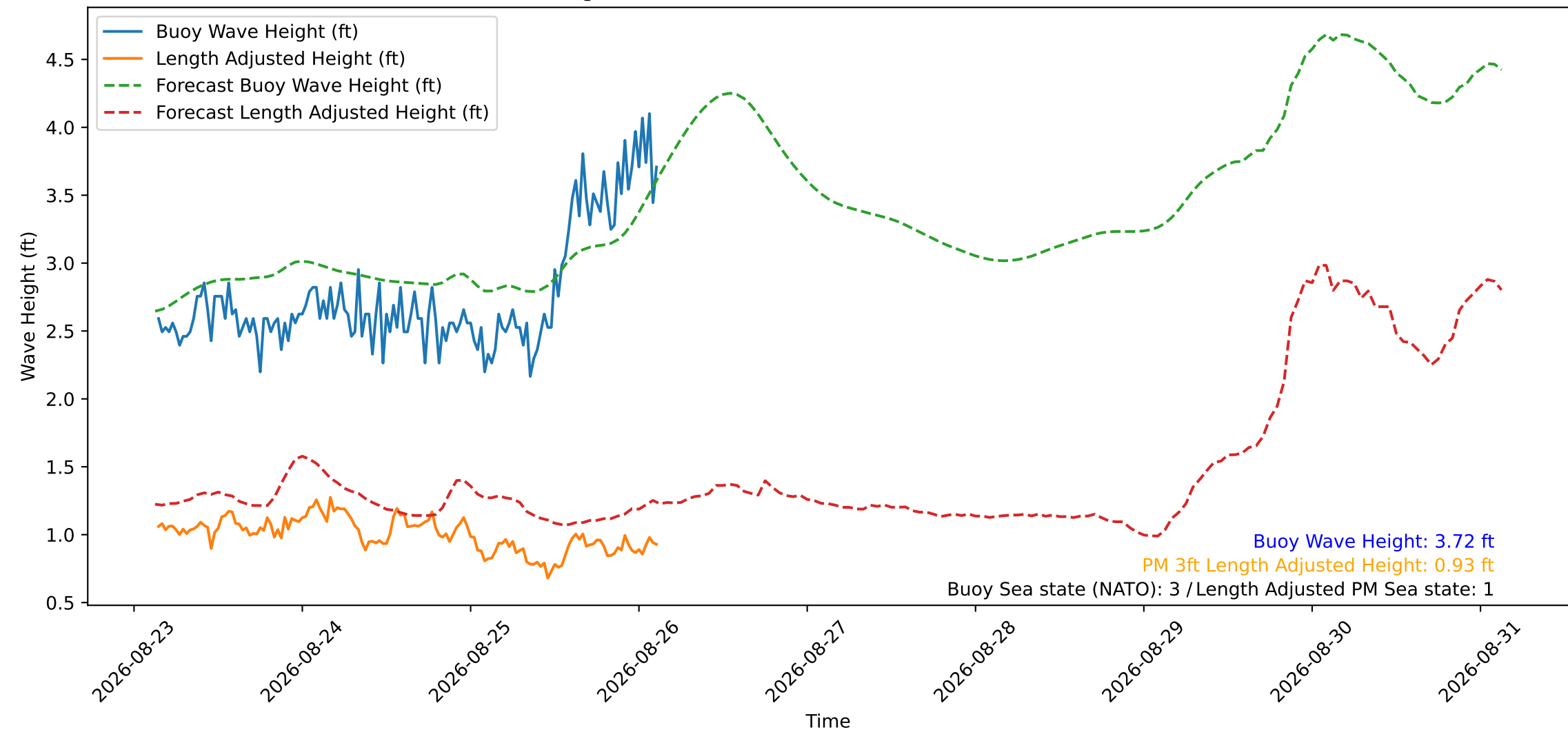
Wave Heights over Time for Red Beach at 2026-08-26 03:20:50
