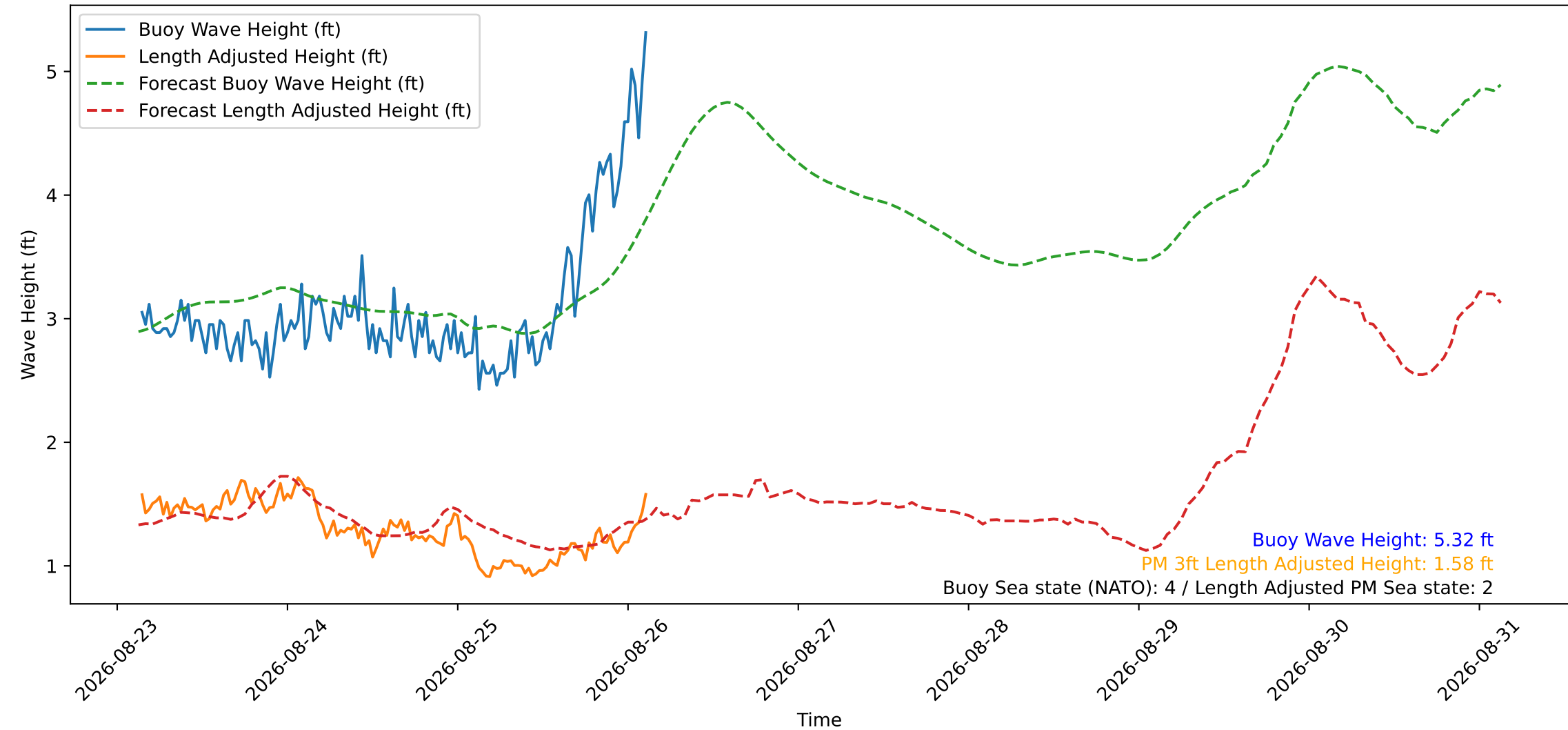
Wave Heights over Time for Oceanside Harbor at 2026-08-26 03:20:29
