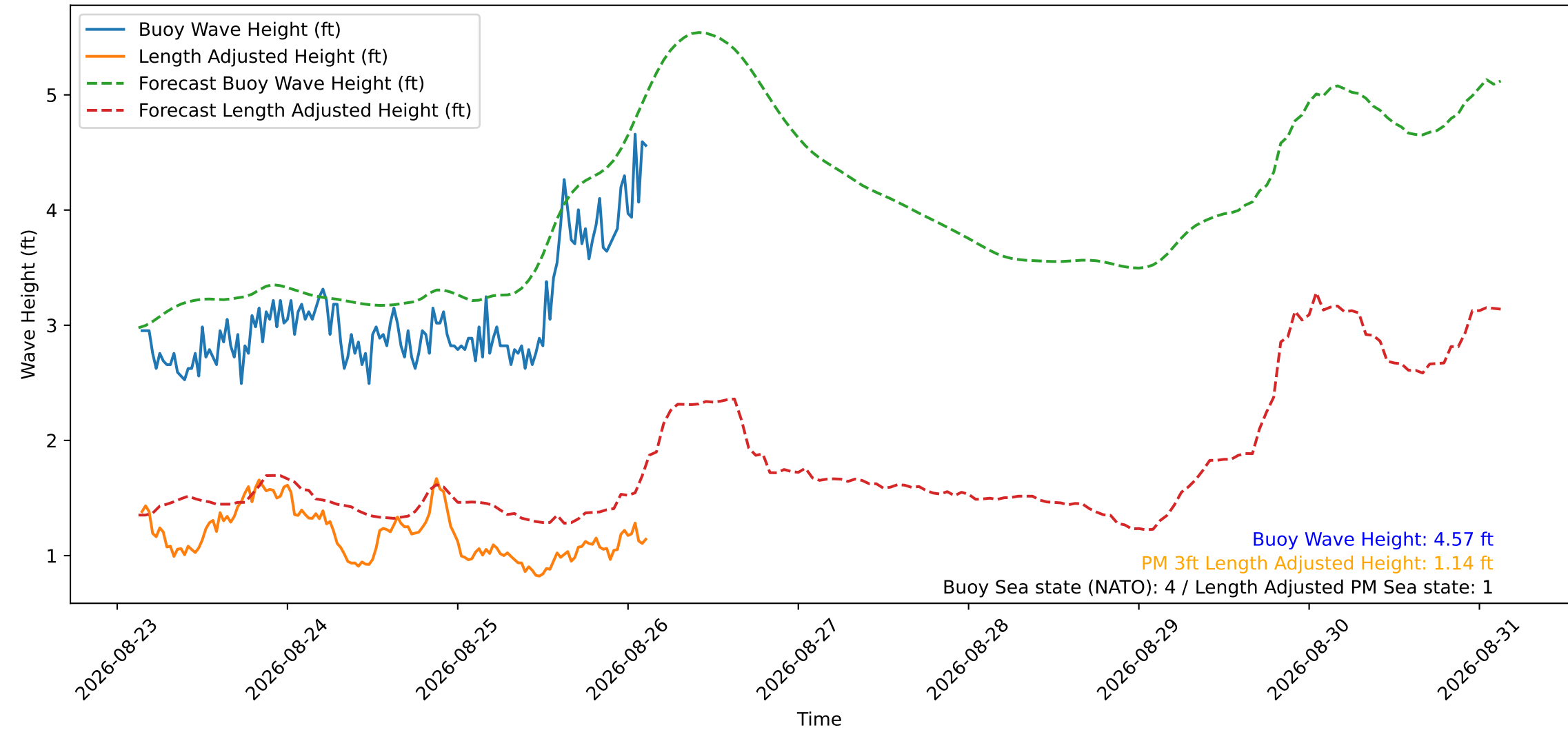
Wave Heights over Time for Green Beach at 2026-08-26 03:21:13
