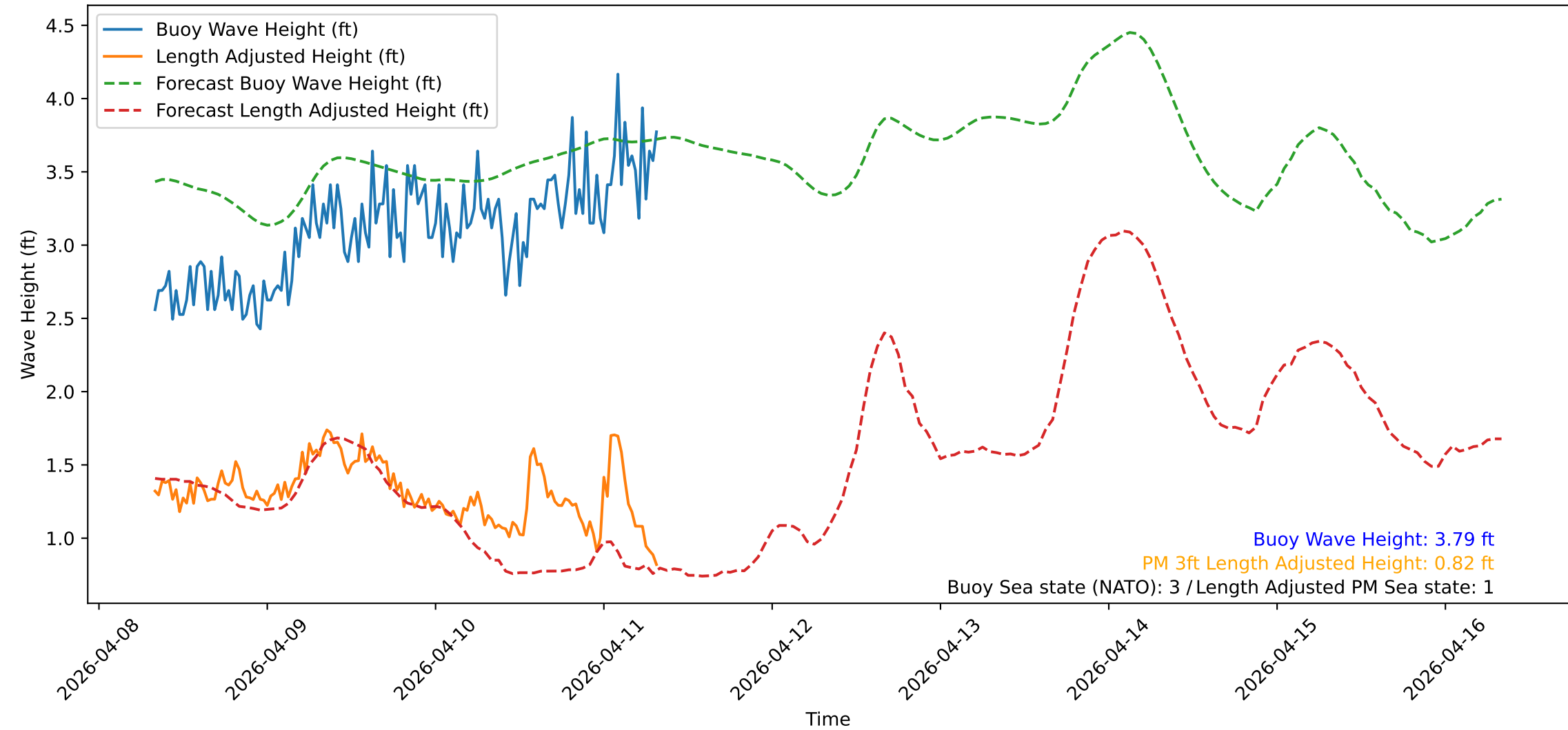
Wave Heights over Time for Oceanside Harbor at 2026-04-11 08:00:32
