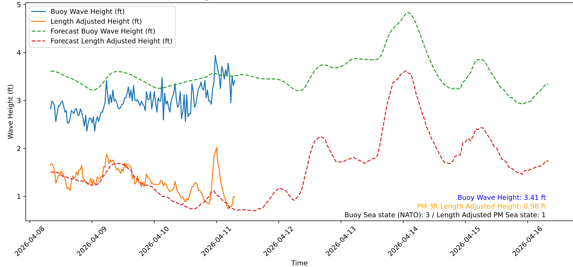
Wave Heights over Time for Green Beach at 2026-04-11 08:01:13
