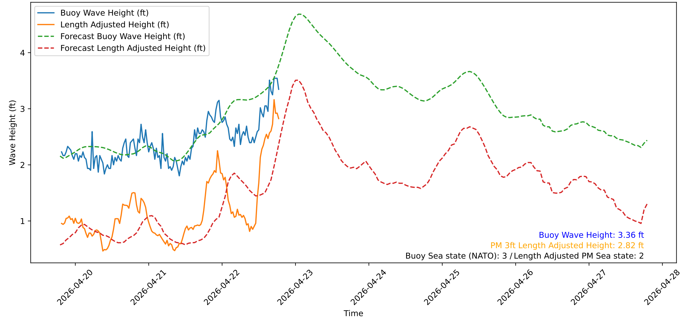
Wave Heights over Time for Red Beach at 2026-04-22 19:20:51
