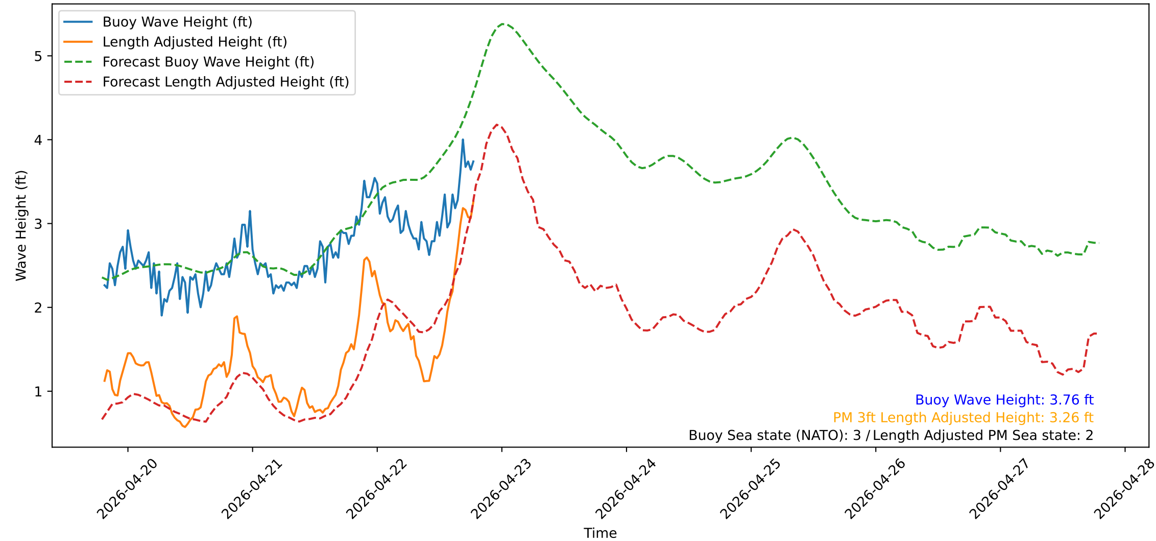
Wave Heights over Time for Green Beach at 2026-04-22 19:21:14
