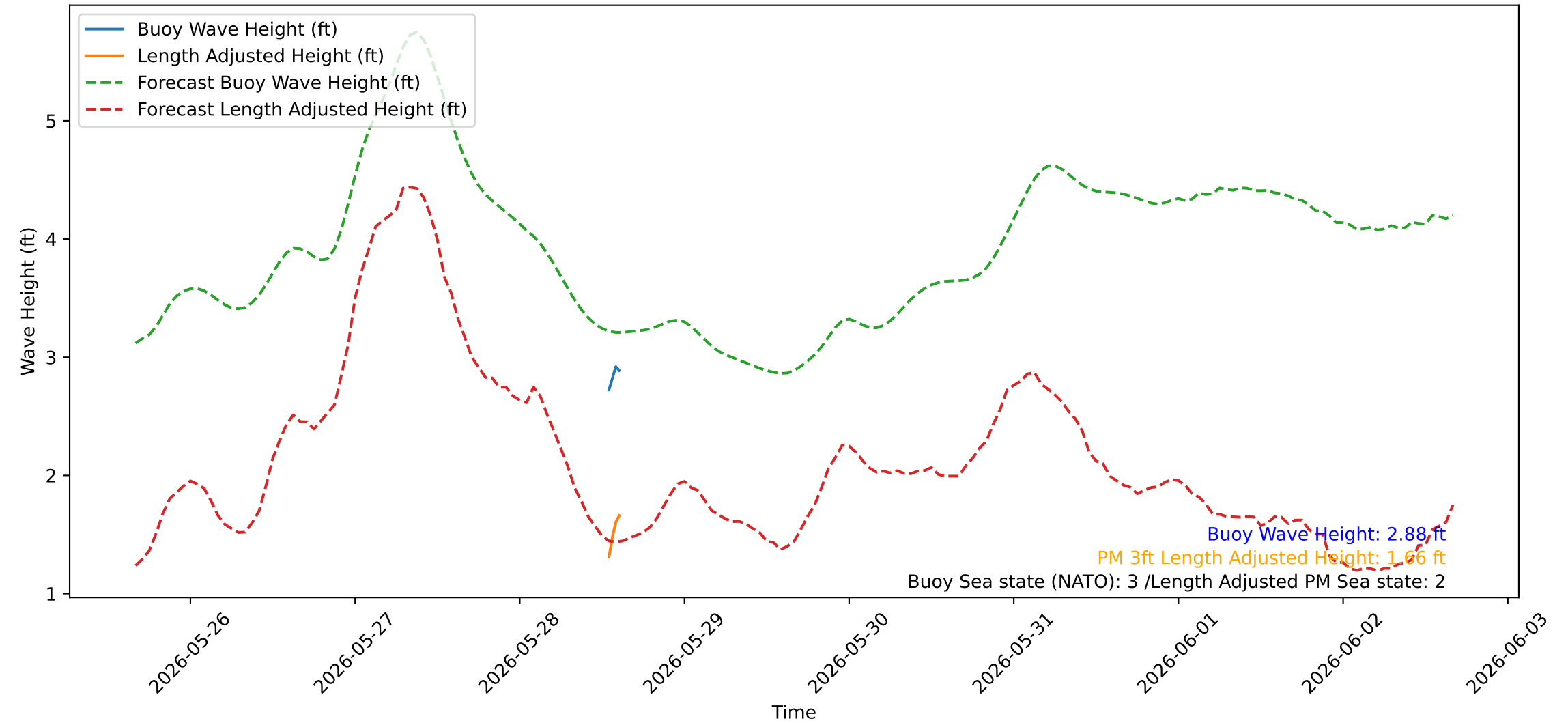
Wave Heights over Time for Oceanside Harbor at 2026-05-28 15:30:19
