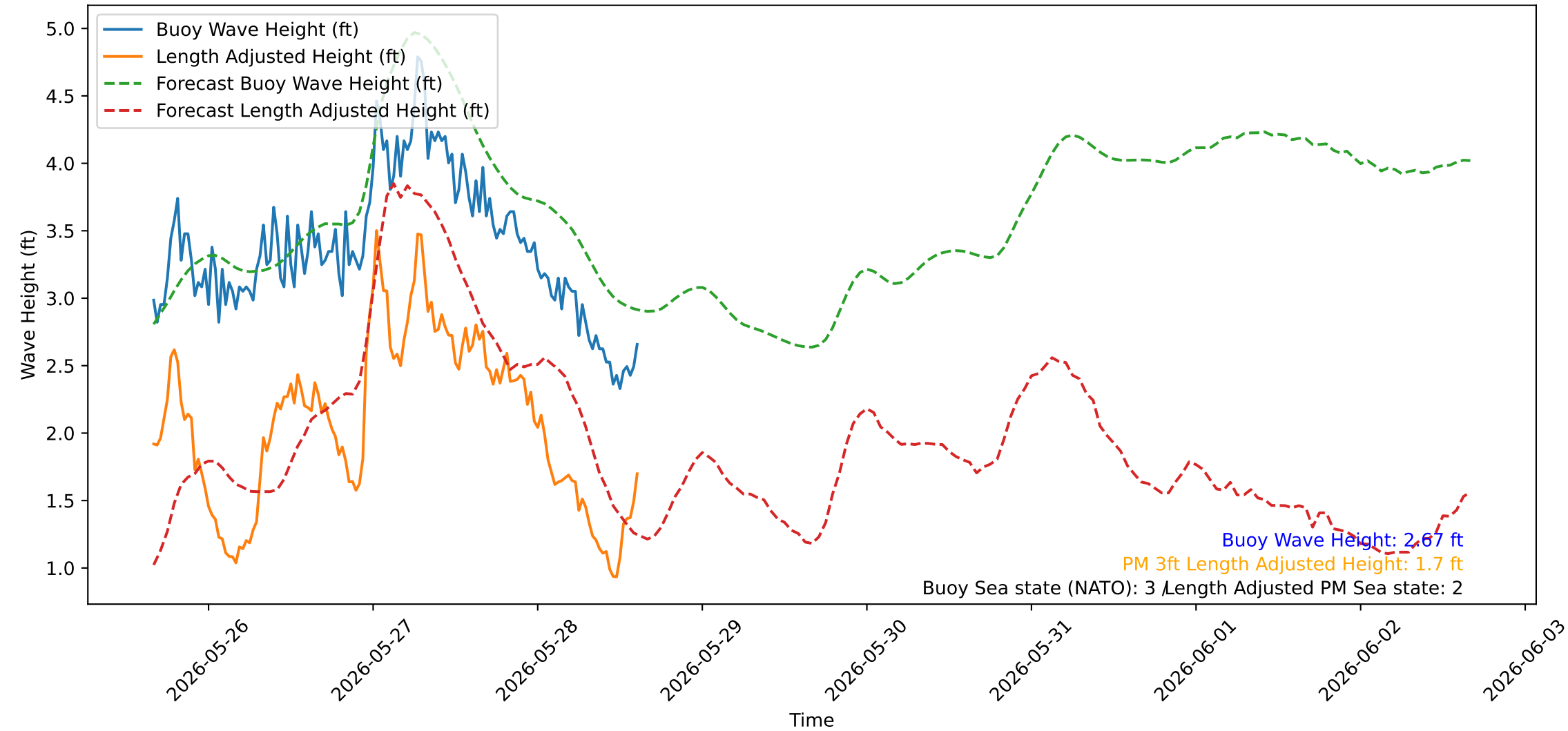
Wave Heights over Time for Red Beach at 2026-05-28 15:30:38
