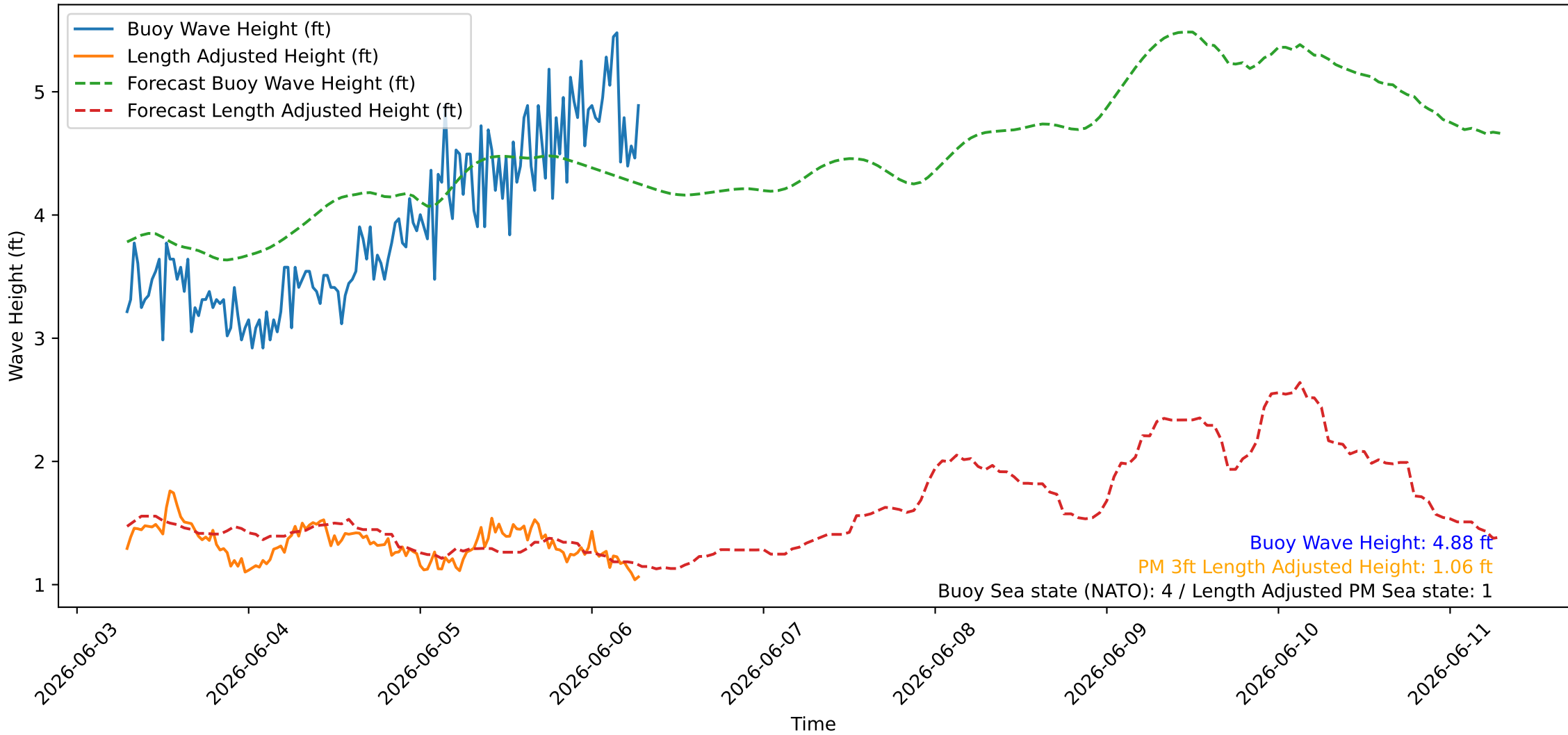
Wave Heights over Time for Oceanside Harbor at 2026-06-06 07:10:26
