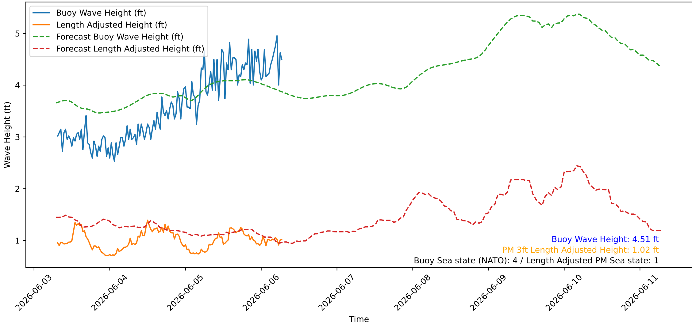
Wave Heights over Time for Red Beach at 2026-06-06 07:10:46
