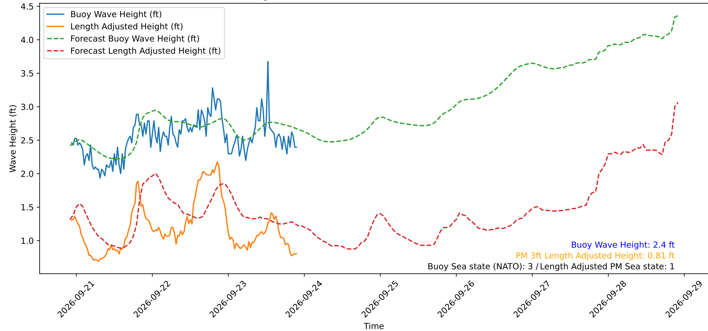
Wave Heights over Time for Red Beach at 2026-09-23 22:10:49
