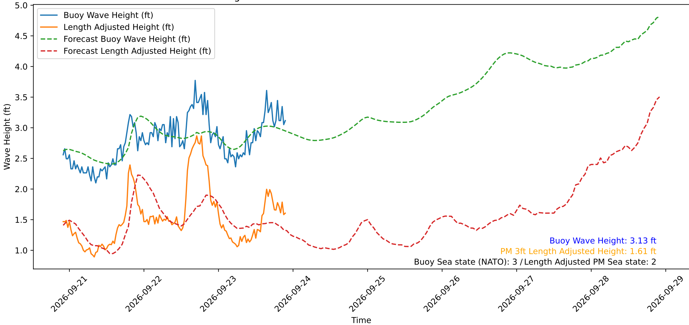
Wave Heights over Time for Oceanside Harbor at 2026-09-23 22:10:30
