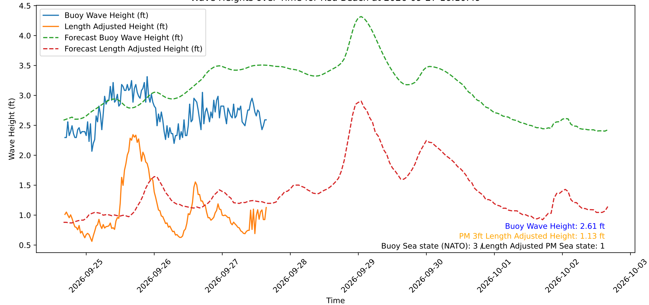
Wave Heights over Time for Red Beach at 2026-09-27 16:10:49
