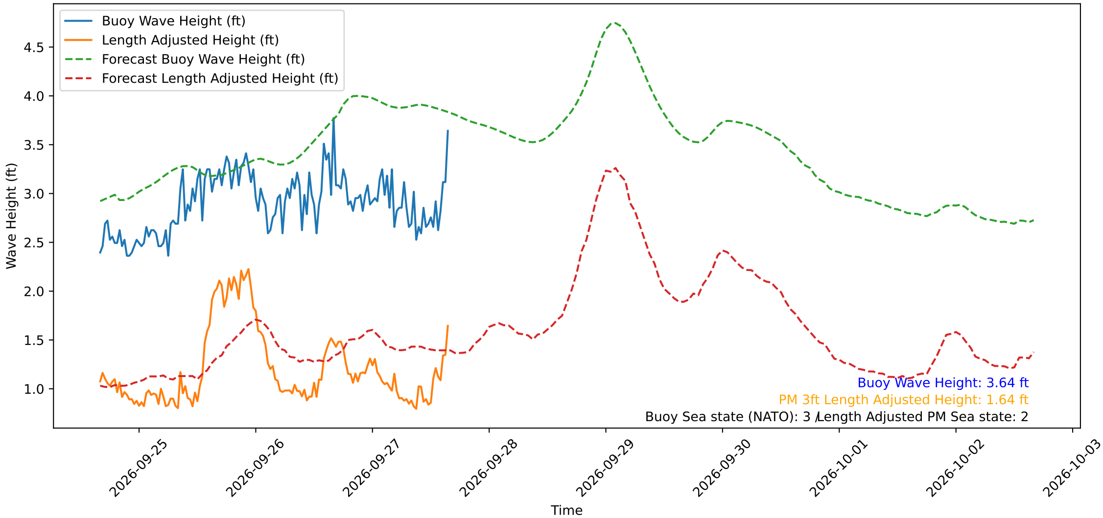
Wave Heights over Time for Oceanside Harbor at 2026-09-27 16:10:29
