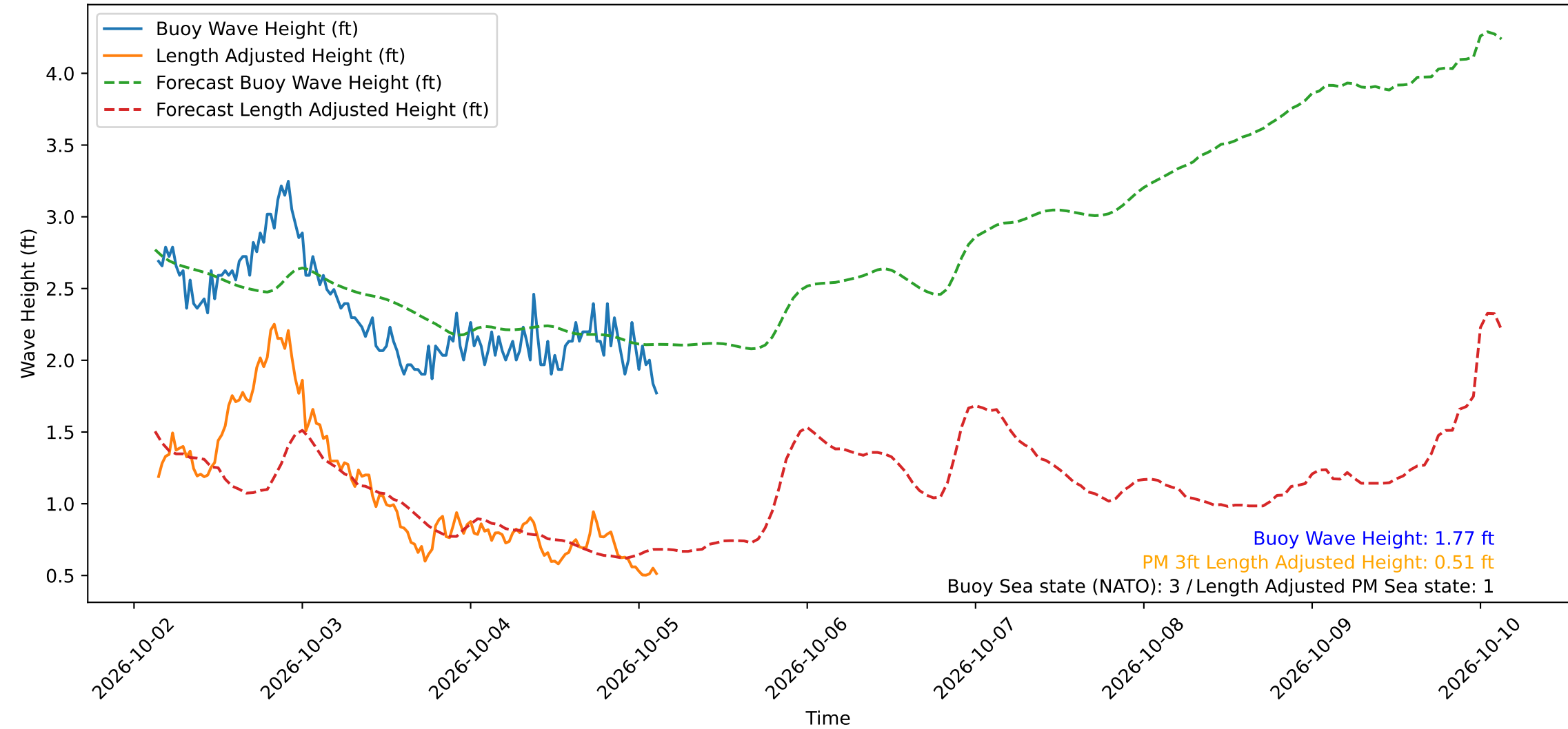
Wave Heights over Time for Red Beach at 2026-10-05 03:10:49
