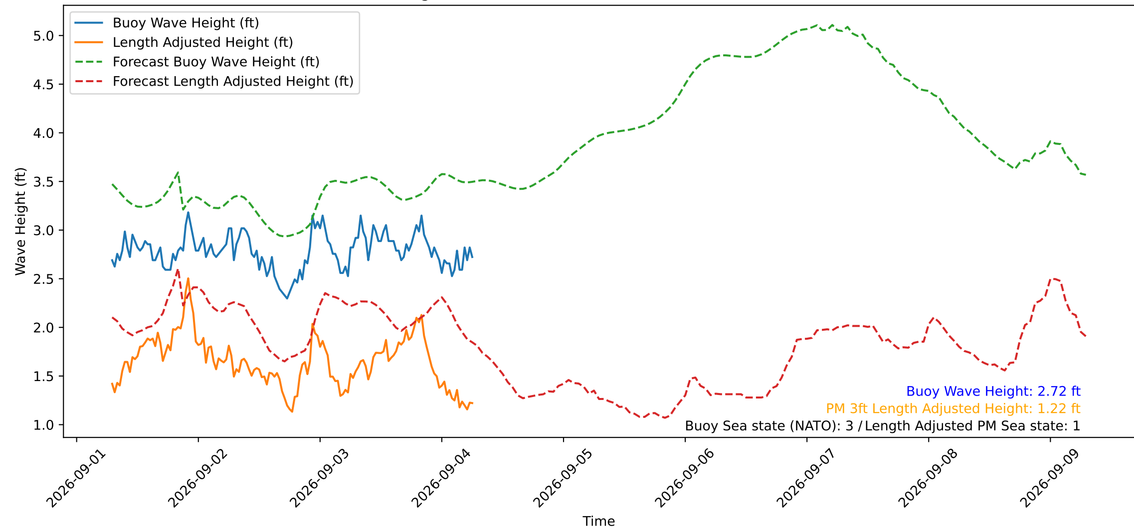
Wave Heights over Time for Red Beach at 2026-09-04 06:50:51
